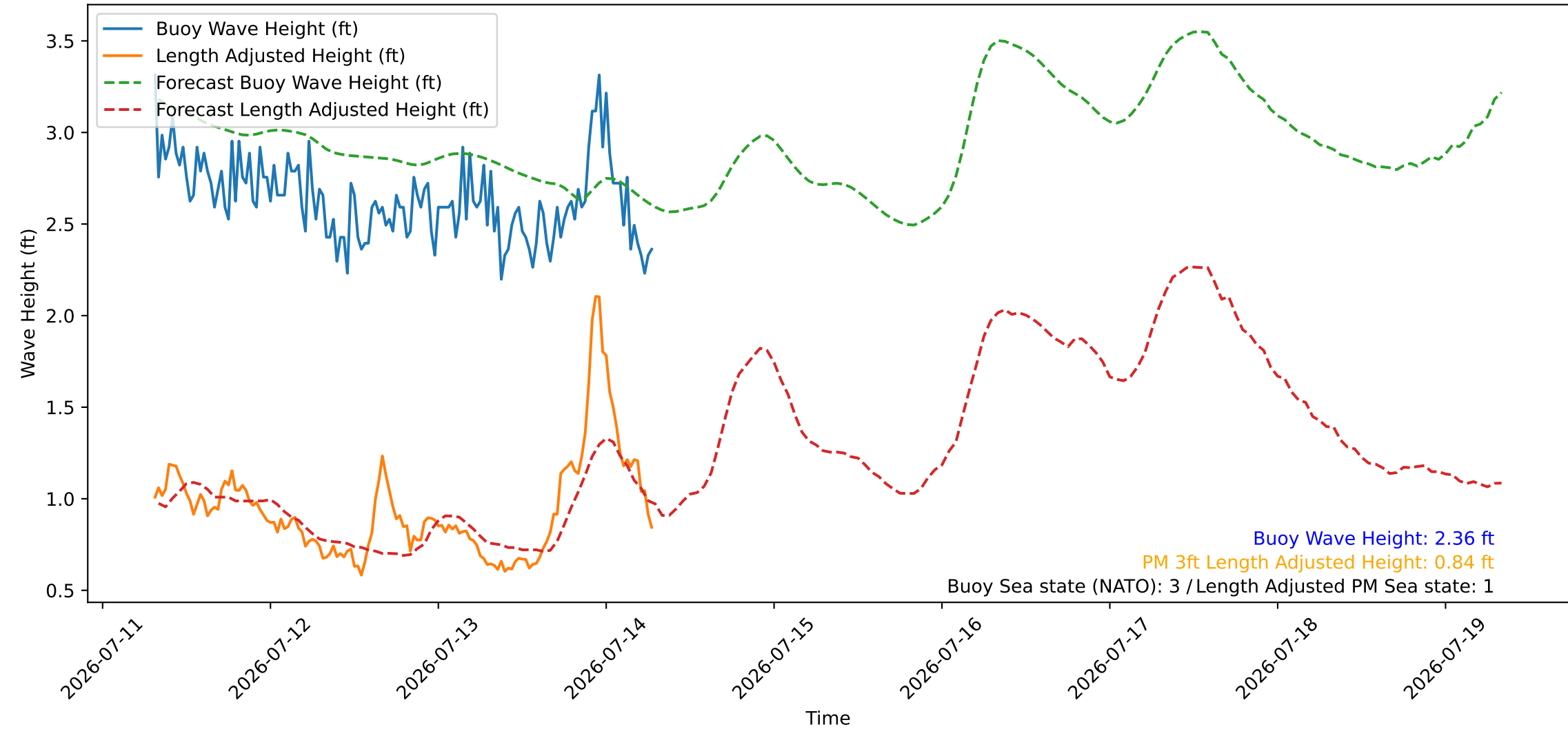
Wave Heights over Time for Green Beach at 2026-07-14 07:31:08
