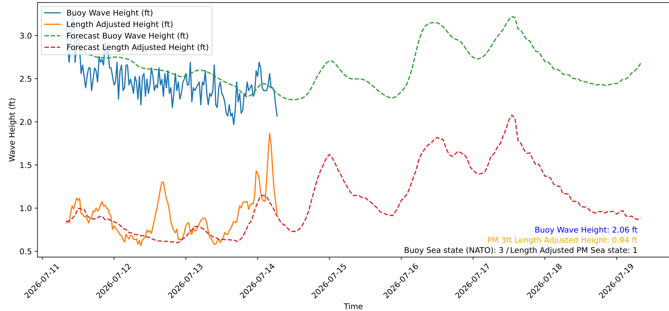
Wave Heights over Time for Red Beach at 2026-07-14 07:30:46
