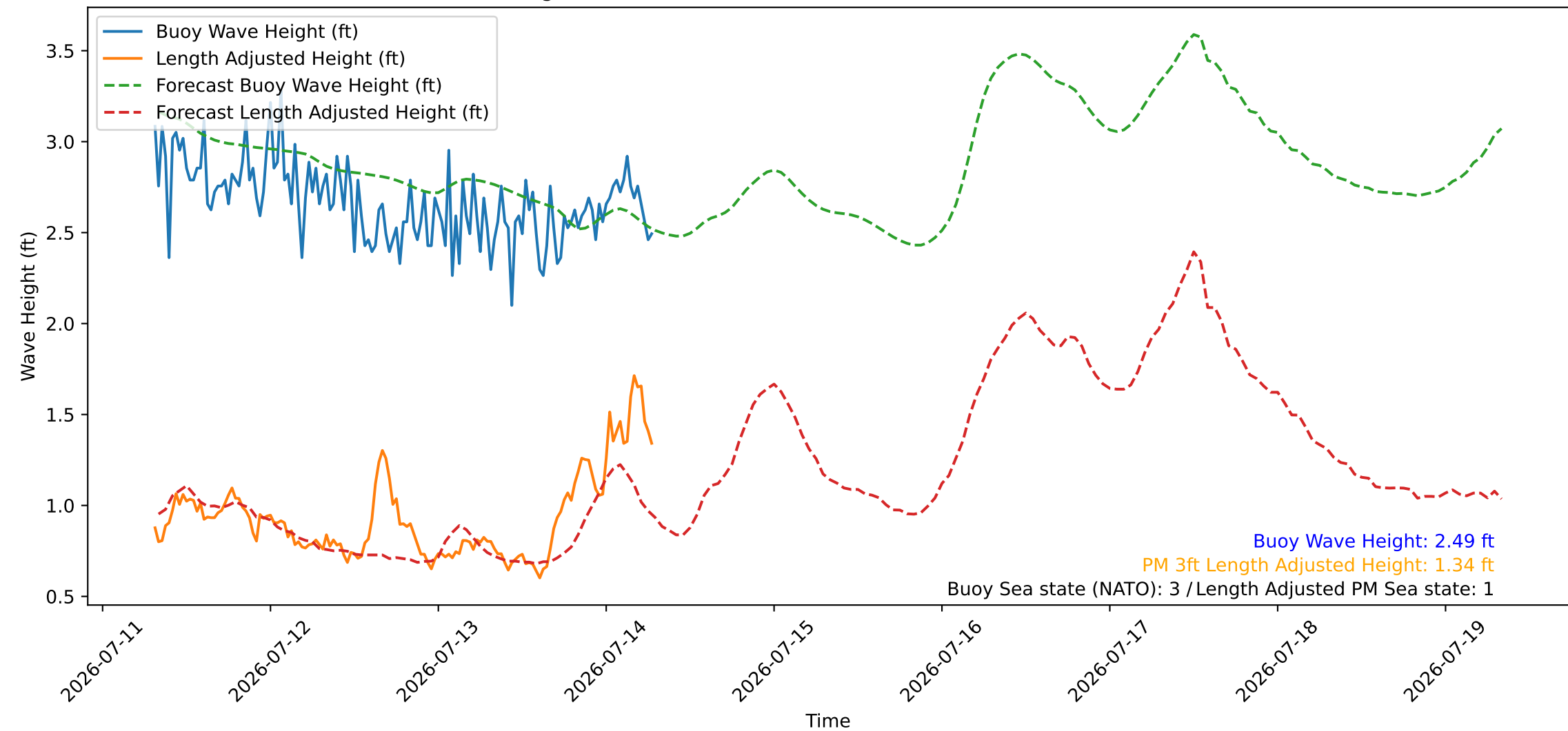
Wave Heights over Time for Oceanside Harbor at 2026-07-14 07:30:26
