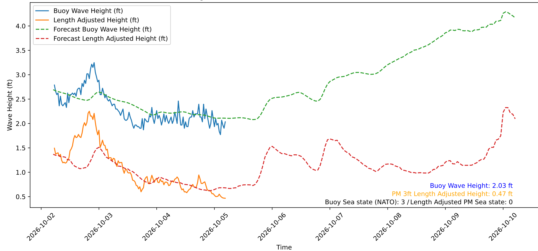
Wave Heights over Time for Red Beach at 2026-10-05 05:20:51
