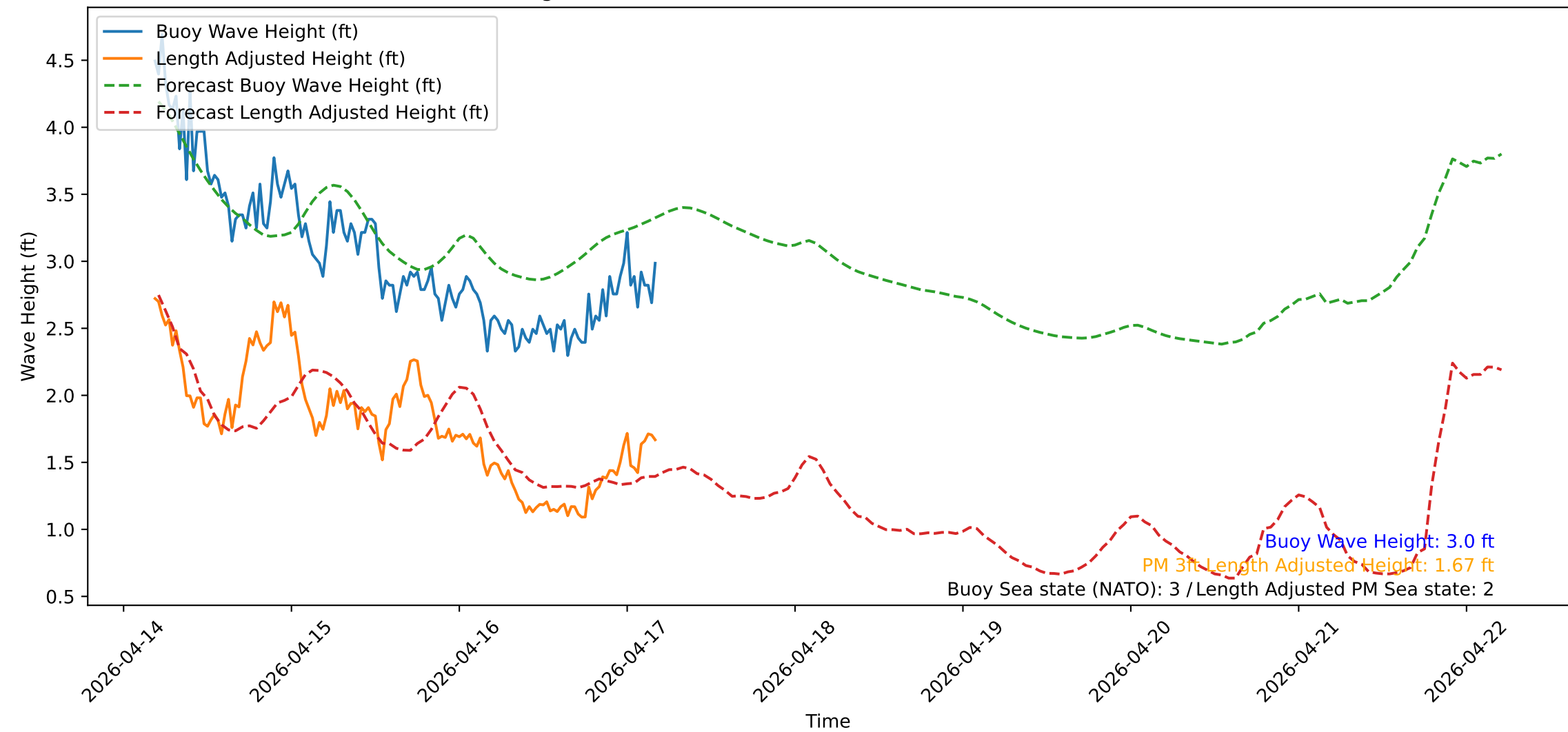
Wave Heights over Time for Oceanside Harbor at 2026-04-17 04:30:32
