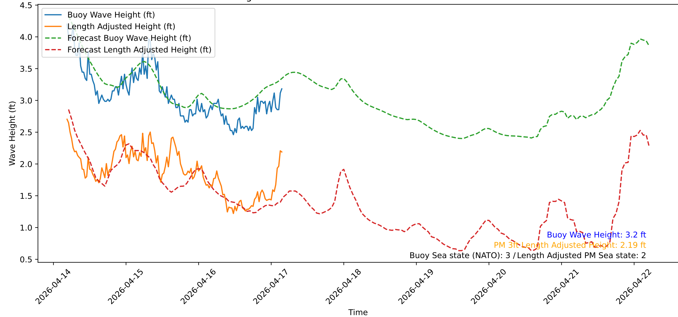
Wave Heights over Time for Green Beach at 2026-04-17 04:31:14
