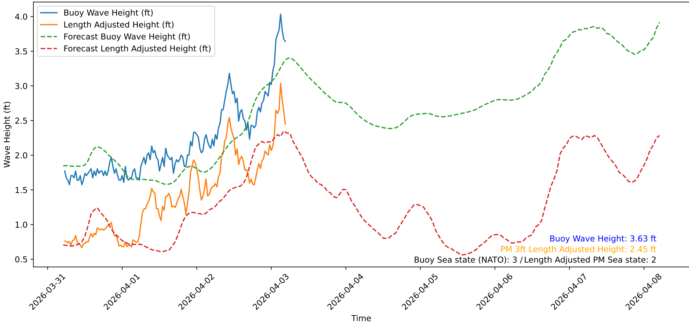
Wave Heights over Time for Oceanside Harbor at 2026-04-03 05:20:31
