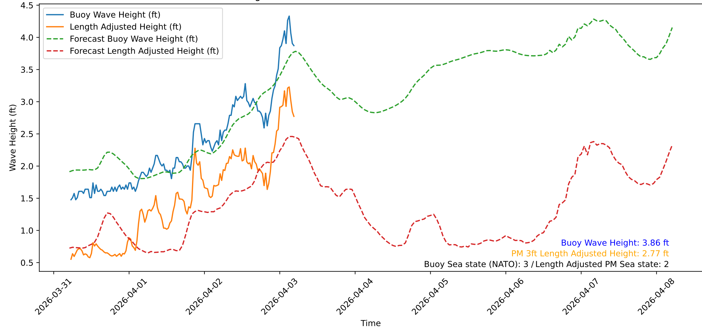
Wave Heights over Time for Green Beach at 2026-04-03 05:21:10
