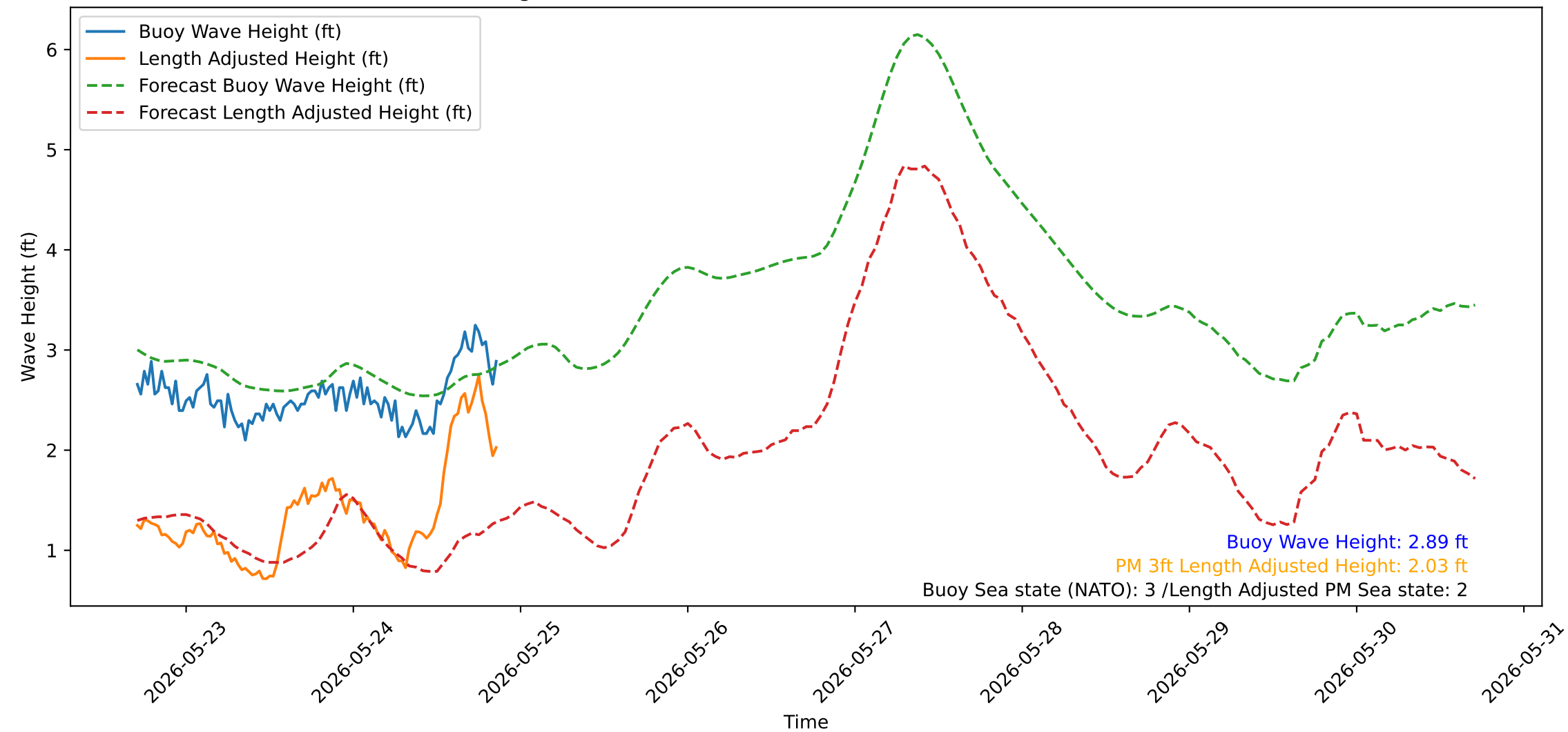
Wave Heights over Time for Oceanside Harbor at 2026-05-25 17:00:29
