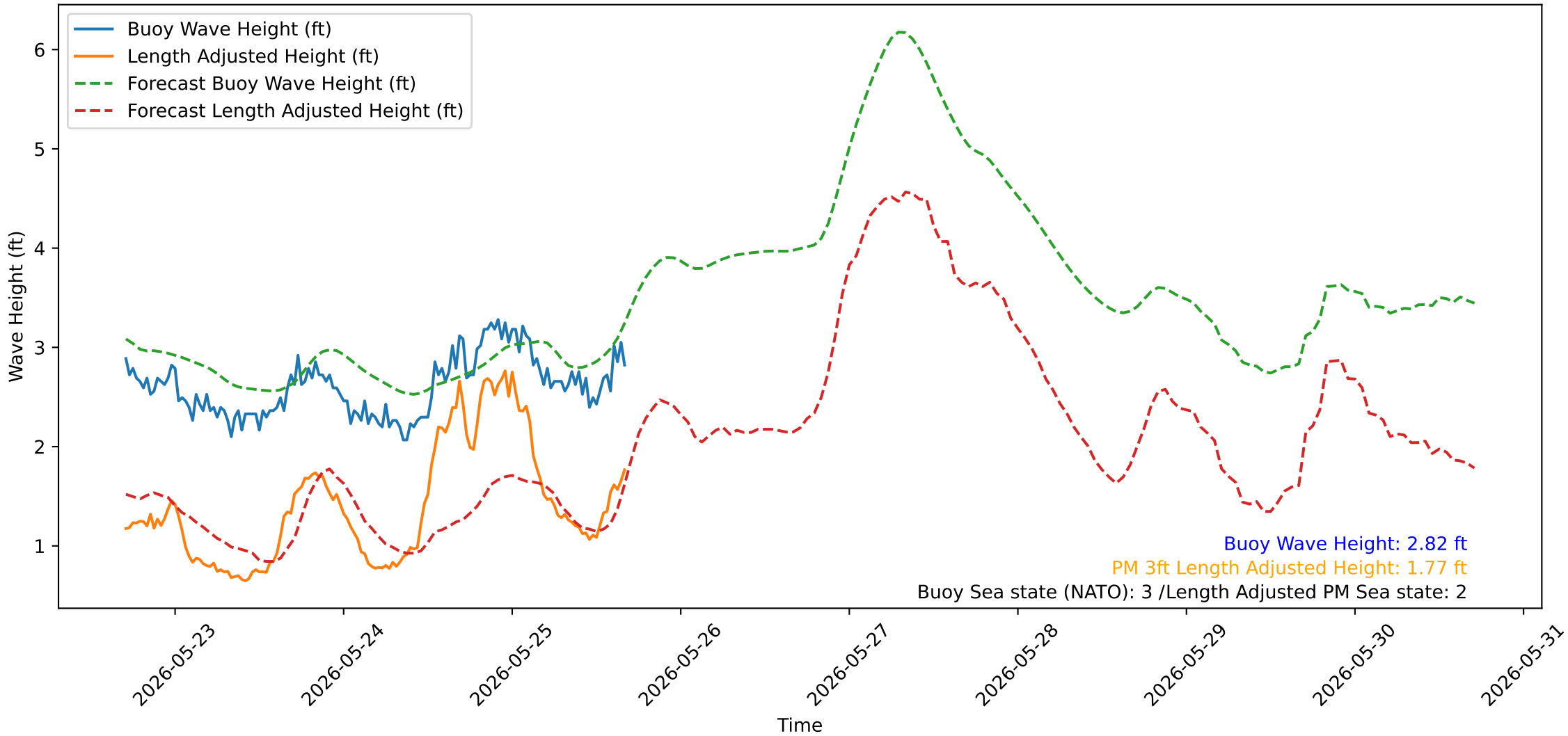
Wave Heights over Time for Green Beach at 2026-05-25 17:01:12
