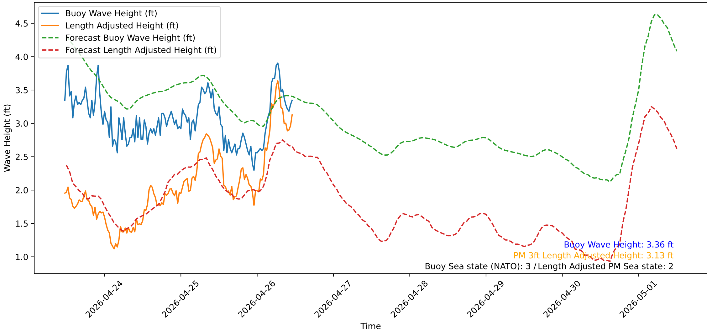
Wave Heights over Time for Oceanside Harbor at 2026-04-26 11:40:31
