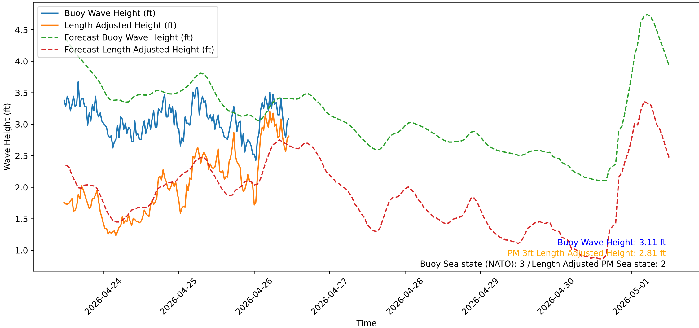
Wave Heights over Time for Green Beach at 2026-04-26 11:41:13
