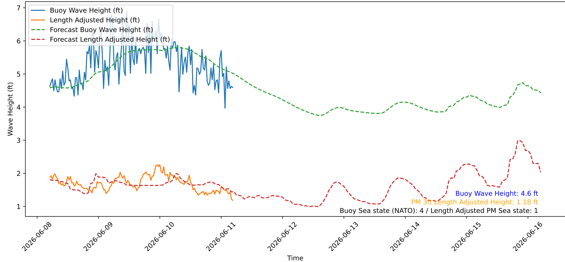
Wave Heights over Time for Green Beach at 2026-06-11 05:11:09
