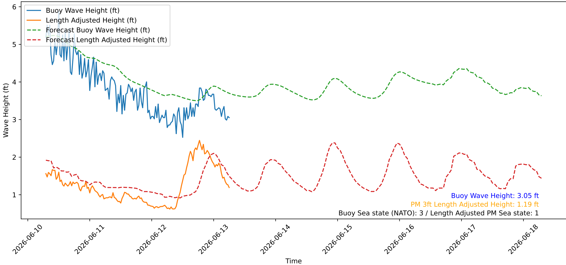
Wave Heights over Time for Red Beach at 2026-06-13 06:50:47
