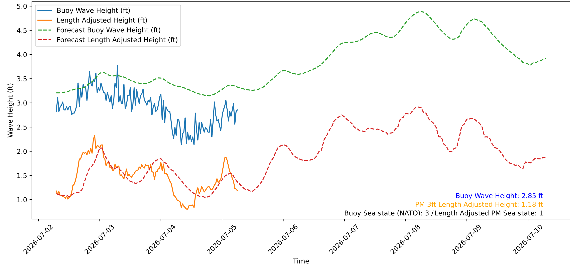
Wave Heights over Time for Oceanside Harbor at 2026-07-05 07:00:26
