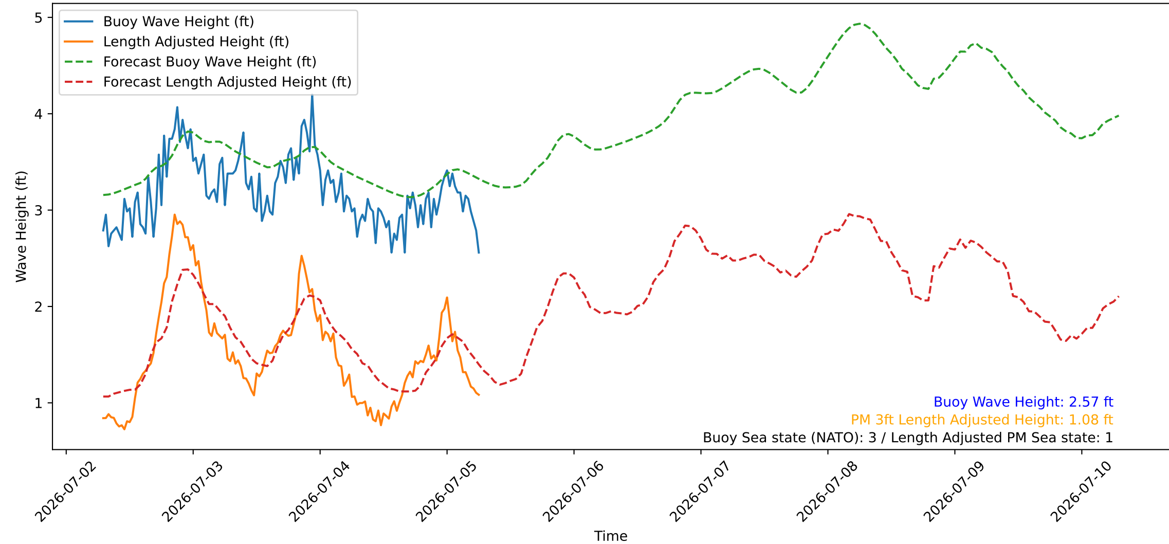
Wave Heights over Time for Green Beach at 2026-07-05 07:01:08
