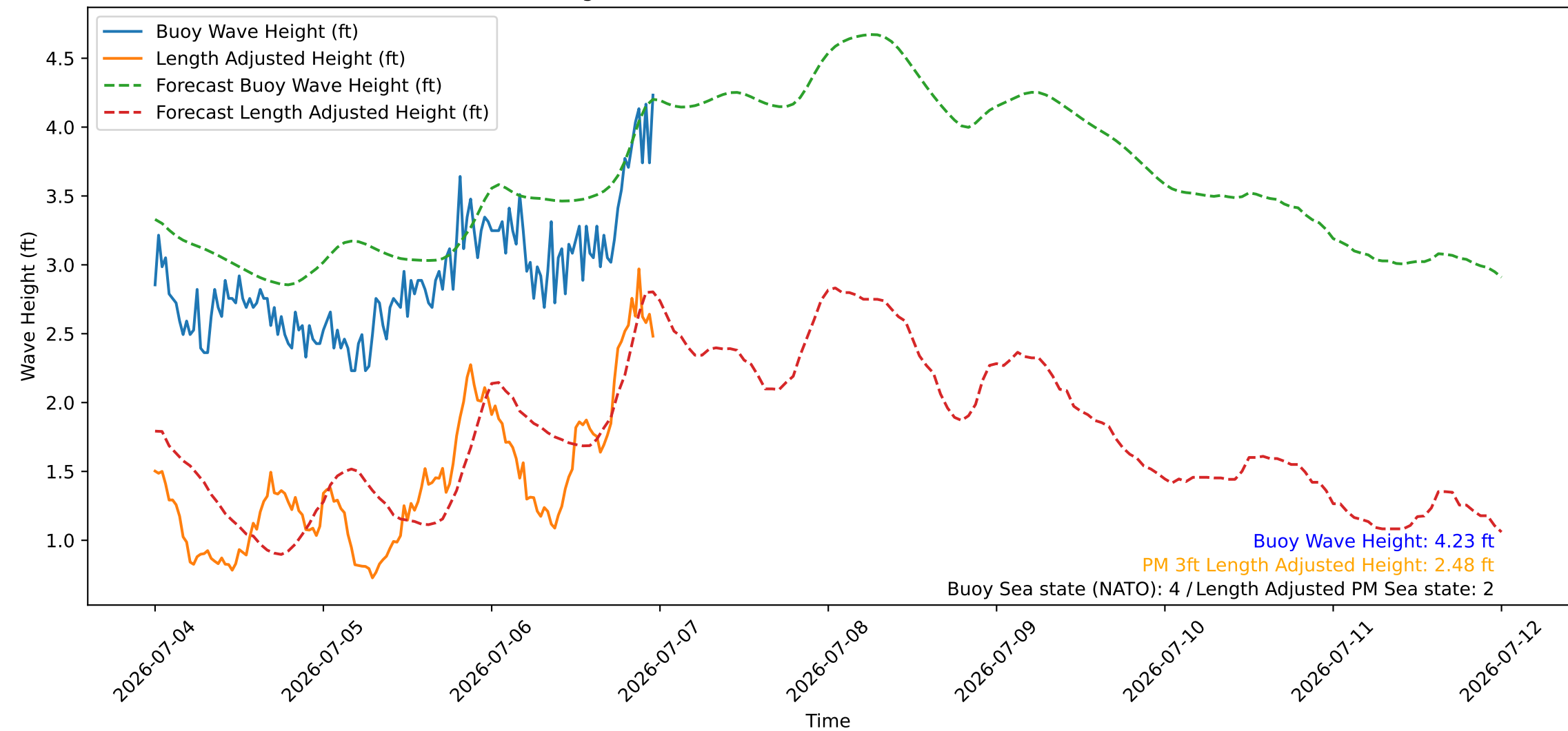
Wave Heights over Time for Red Beach at 2026-07-06 23:50:46
