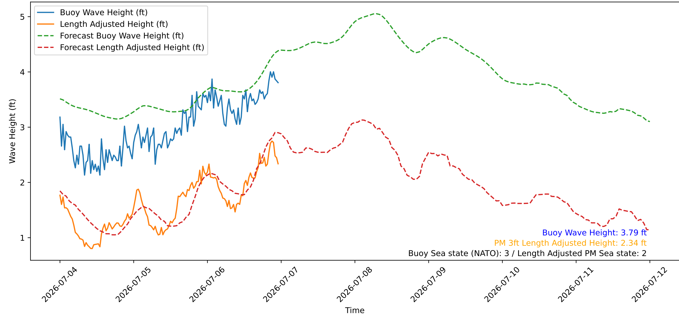
Wave Heights over Time for Oceanside Harbor at 2026-07-06 23:50:26
