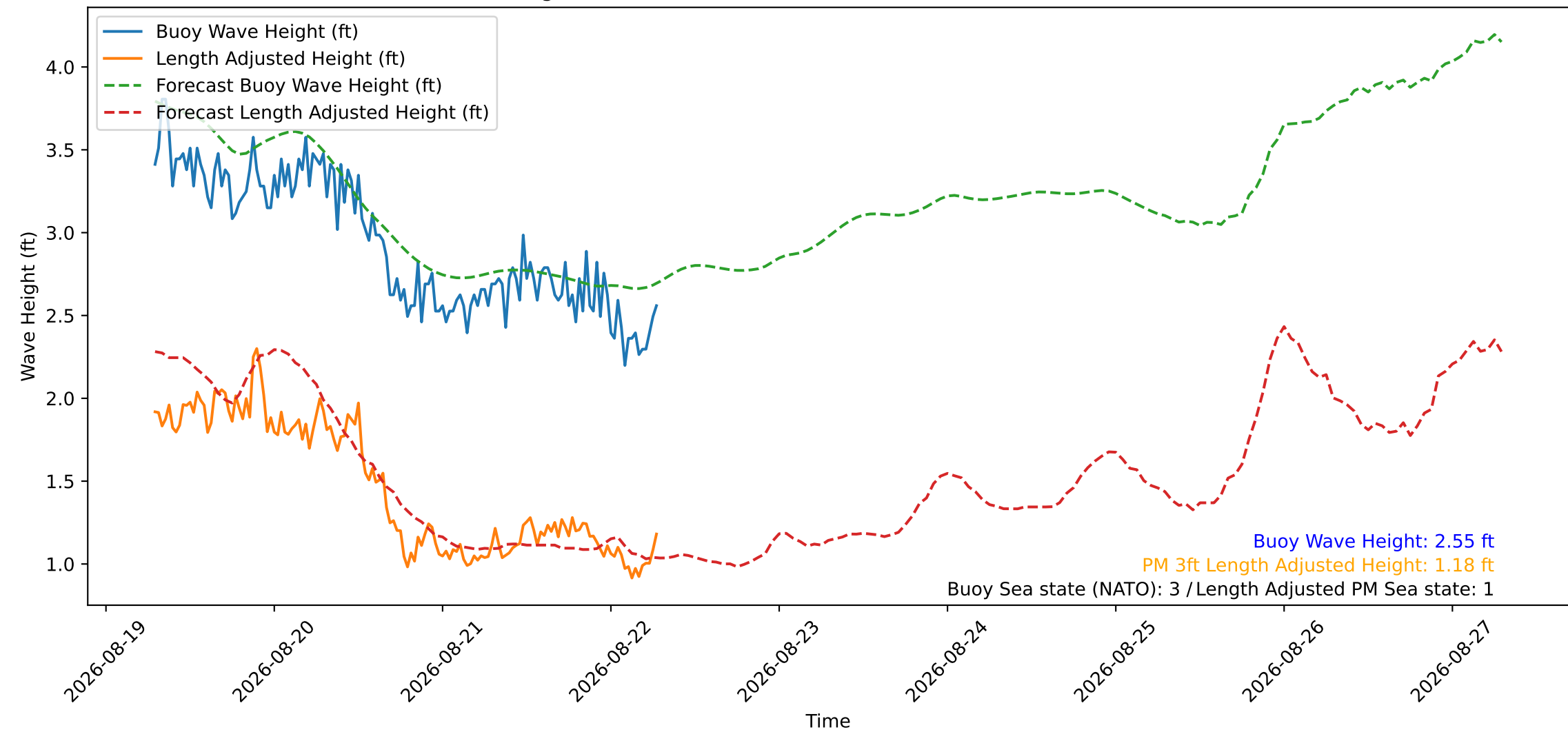
Wave Heights over Time for Oceanside Harbor at 2026-08-22 07:10:30
