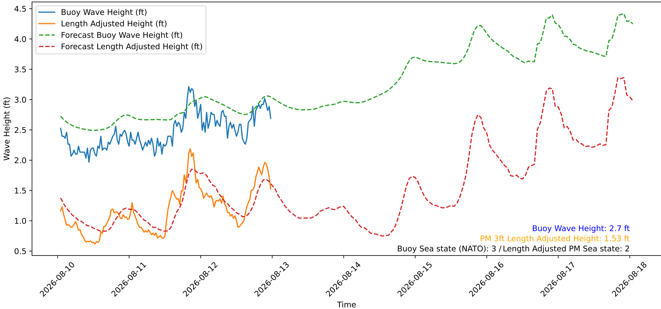
Wave Heights over Time for Green Beach at 2026-08-13 01:01:09
