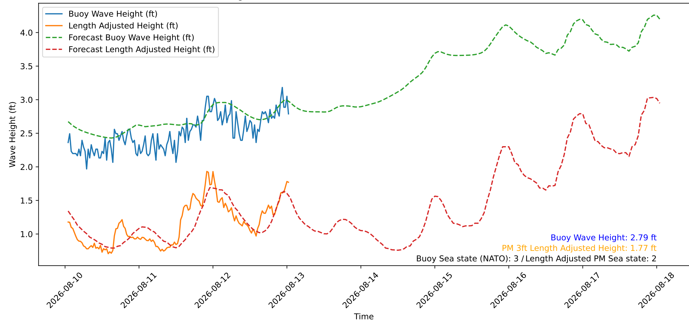
Wave Heights over Time for Oceanside Harbor at 2026-08-13 01:00:28
