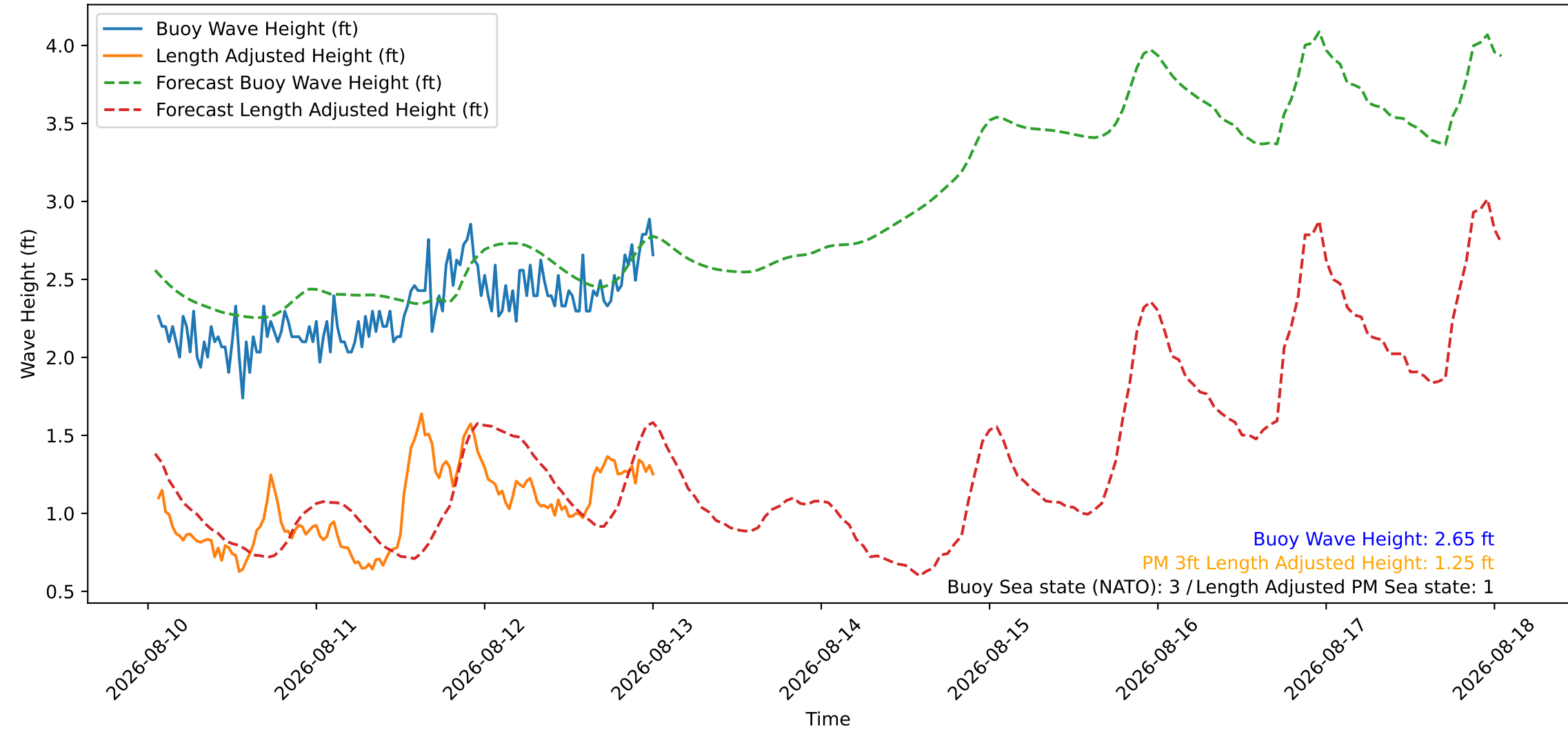
Wave Heights over Time for Red Beach at 2026-08-13 01:00:47
