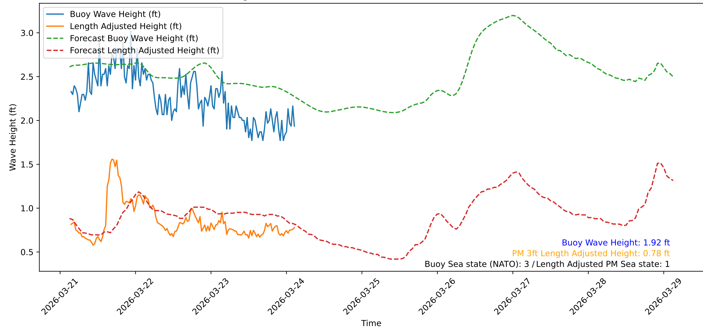
Wave Heights over Time for Oceanside Harbor at 2026-03-24 03:20:32
