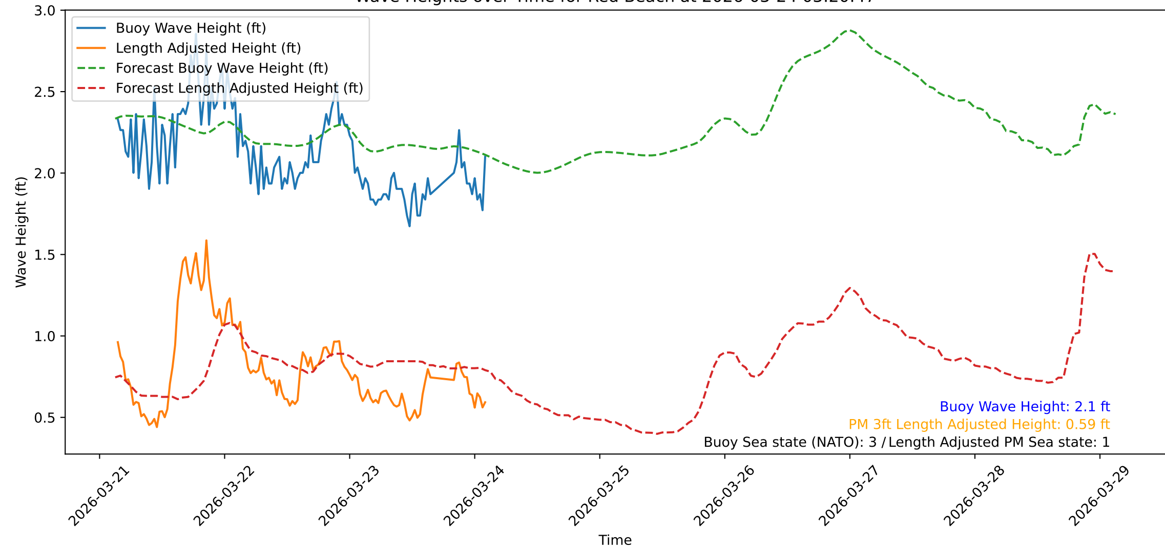
Wave Heights over Time for Red Beach at 2026-03-24 03:20:47
