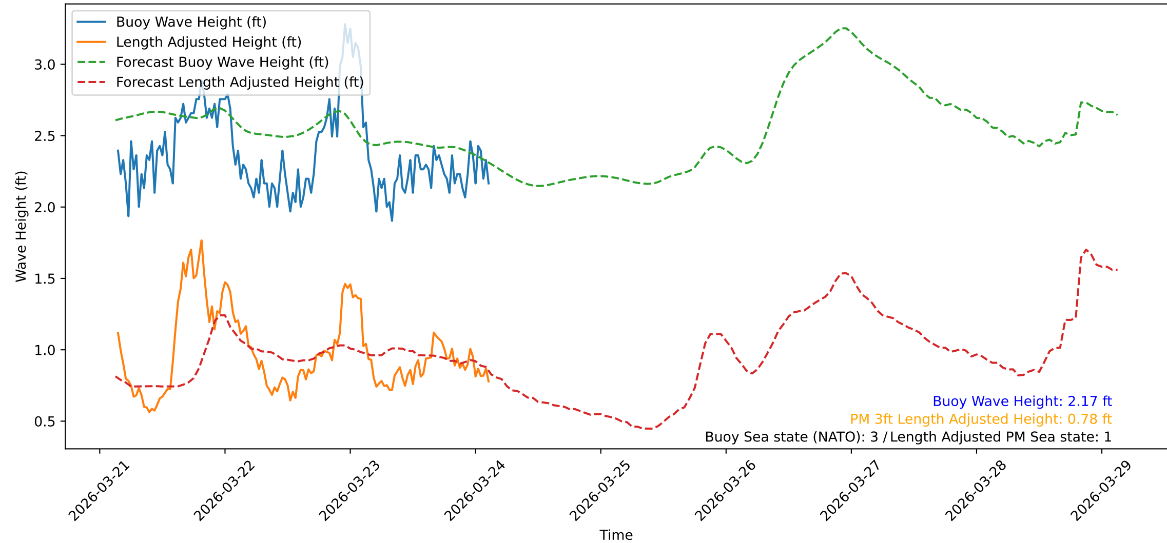
Wave Heights over Time for Green Beach at 2026-03-24 03:21:09
