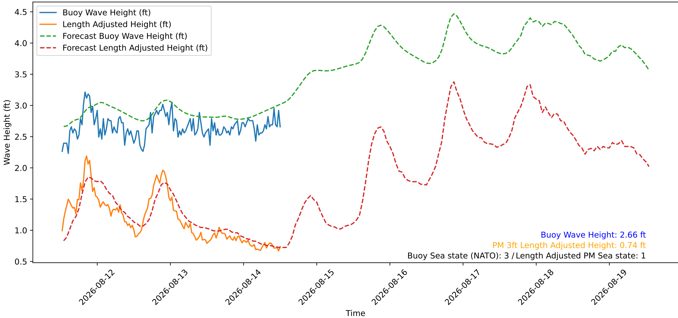
Wave Heights over Time for Green Beach at 2026-08-14 12:41:08
