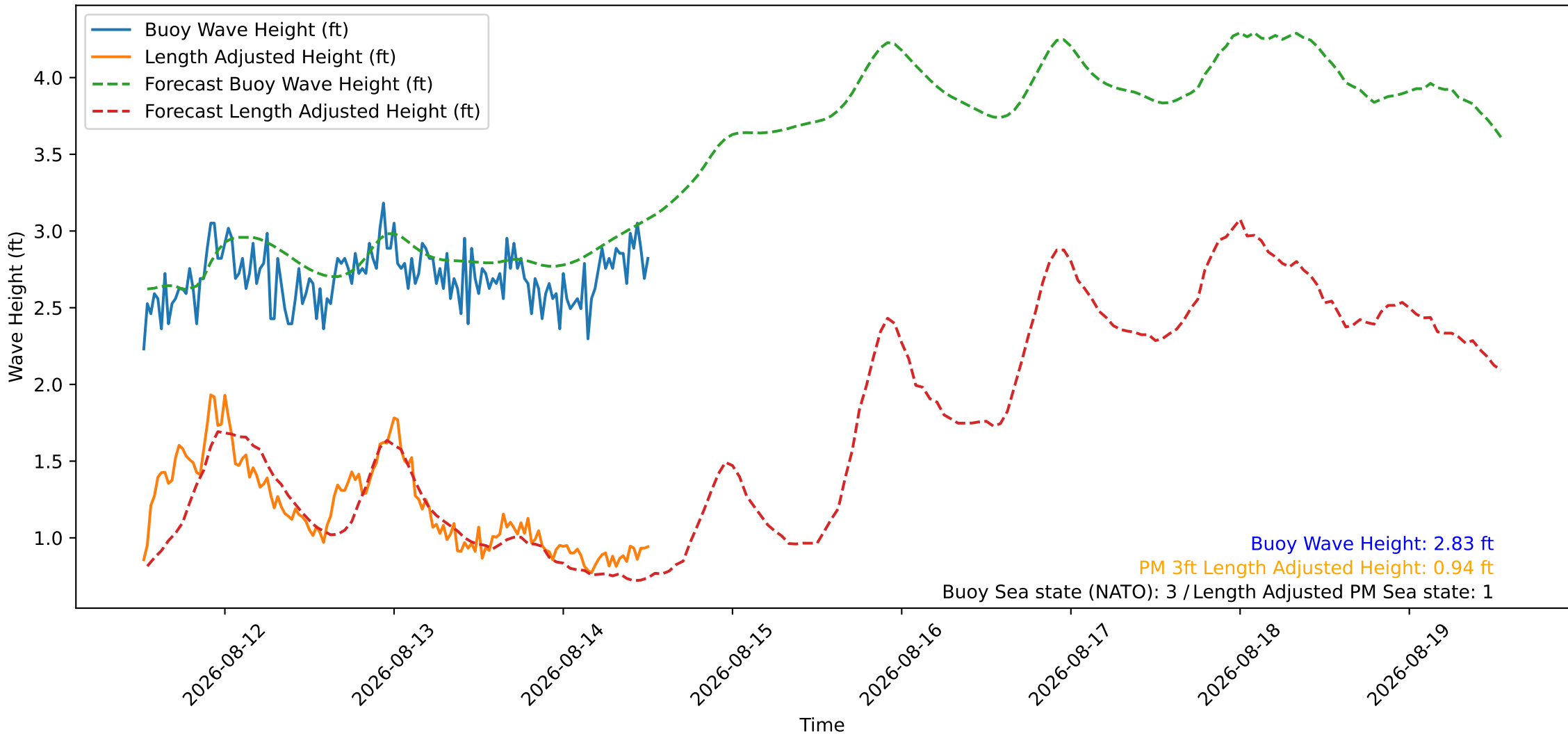
Wave Heights over Time for Oceanside Harbor at 2026-08-14 12:40:26
