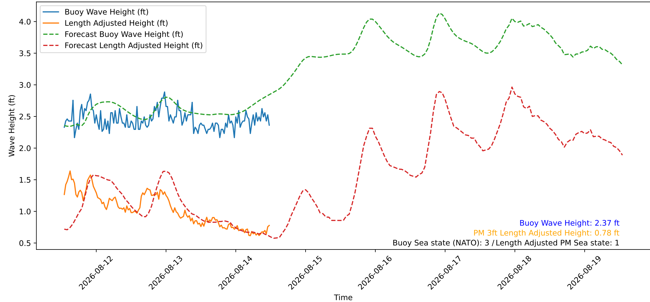
Wave Heights over Time for Red Beach at 2026-08-14 12:40:45
