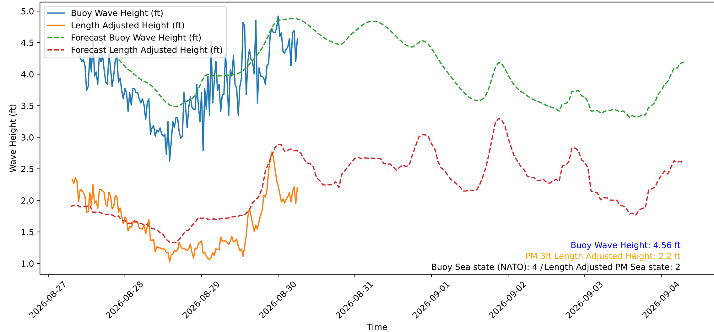
Wave Heights over Time for Green Beach at 2026-08-30 07:11:11
