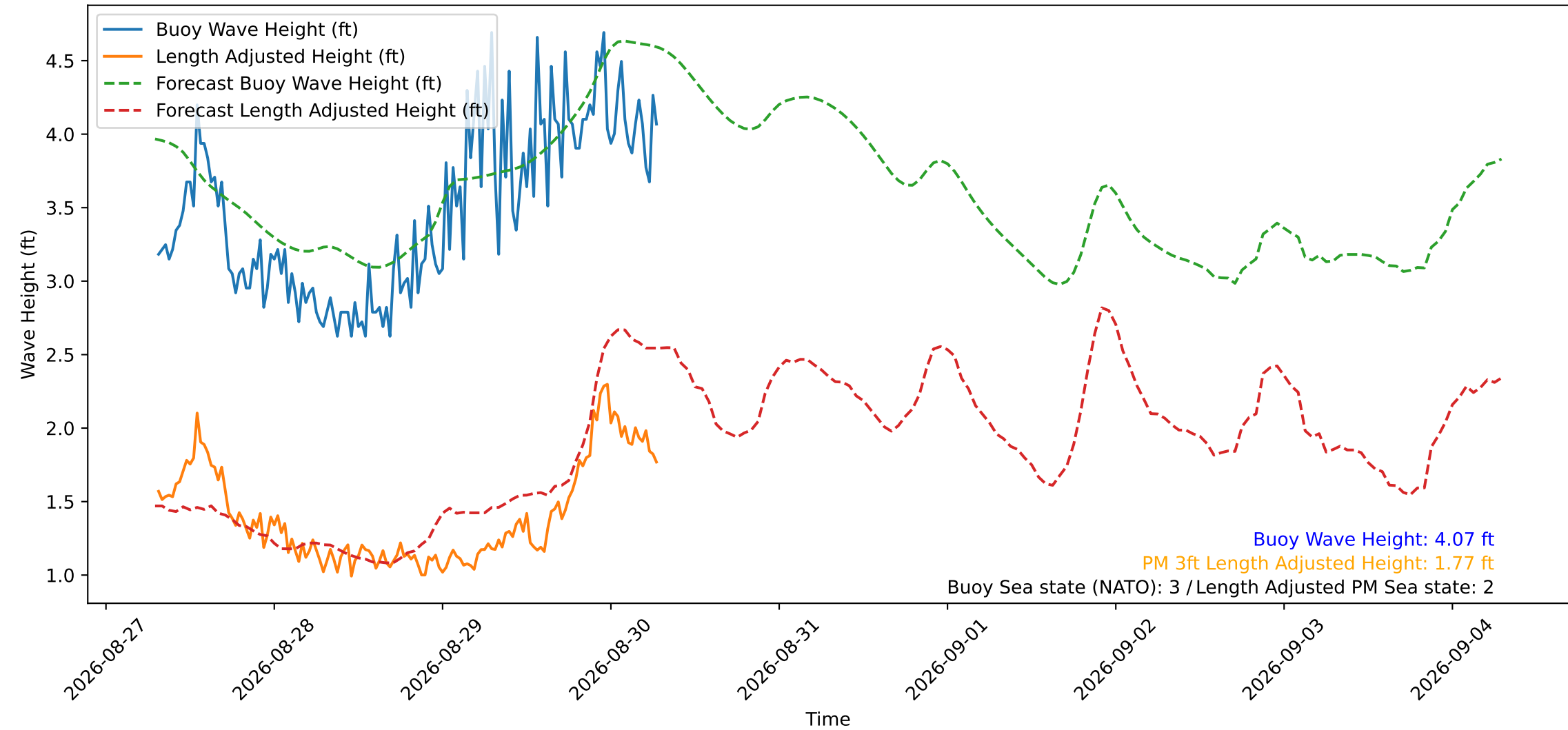
Wave Heights over Time for Red Beach at 2026-08-30 07:10:48
