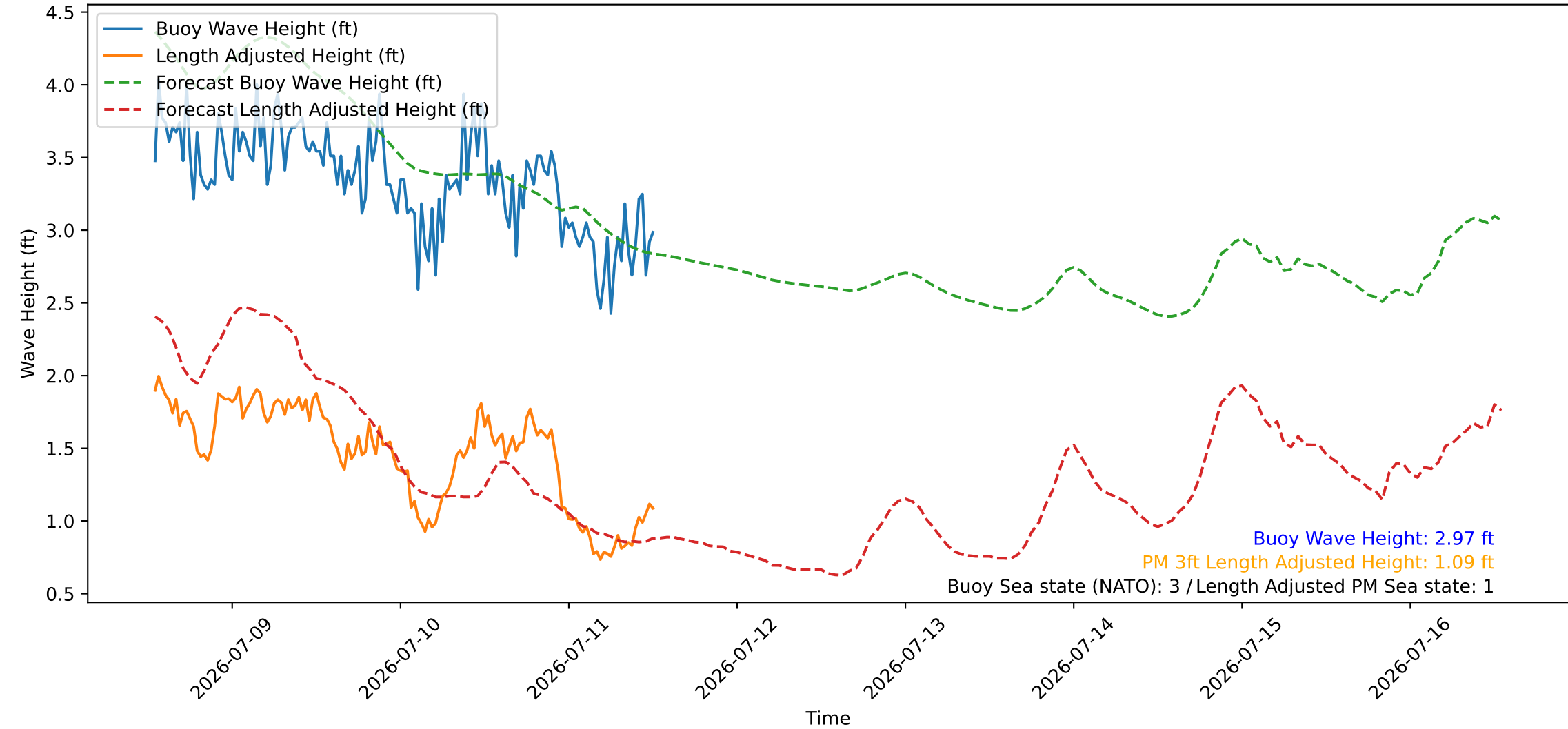
Wave Heights over Time for Red Beach at 2026-07-11 12:50:47
