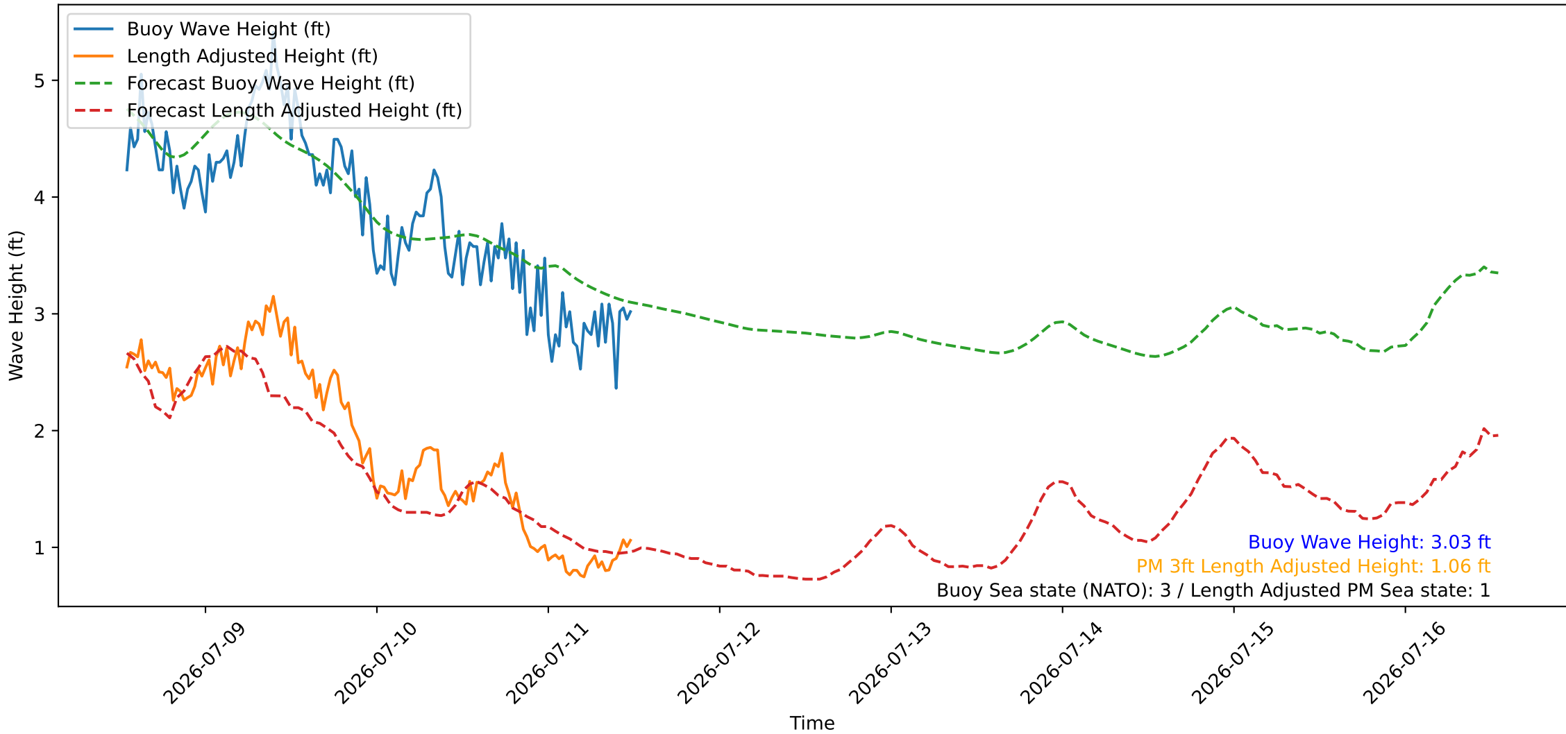
Wave Heights over Time for Oceanside Harbor at 2026-07-11 12:50:26
