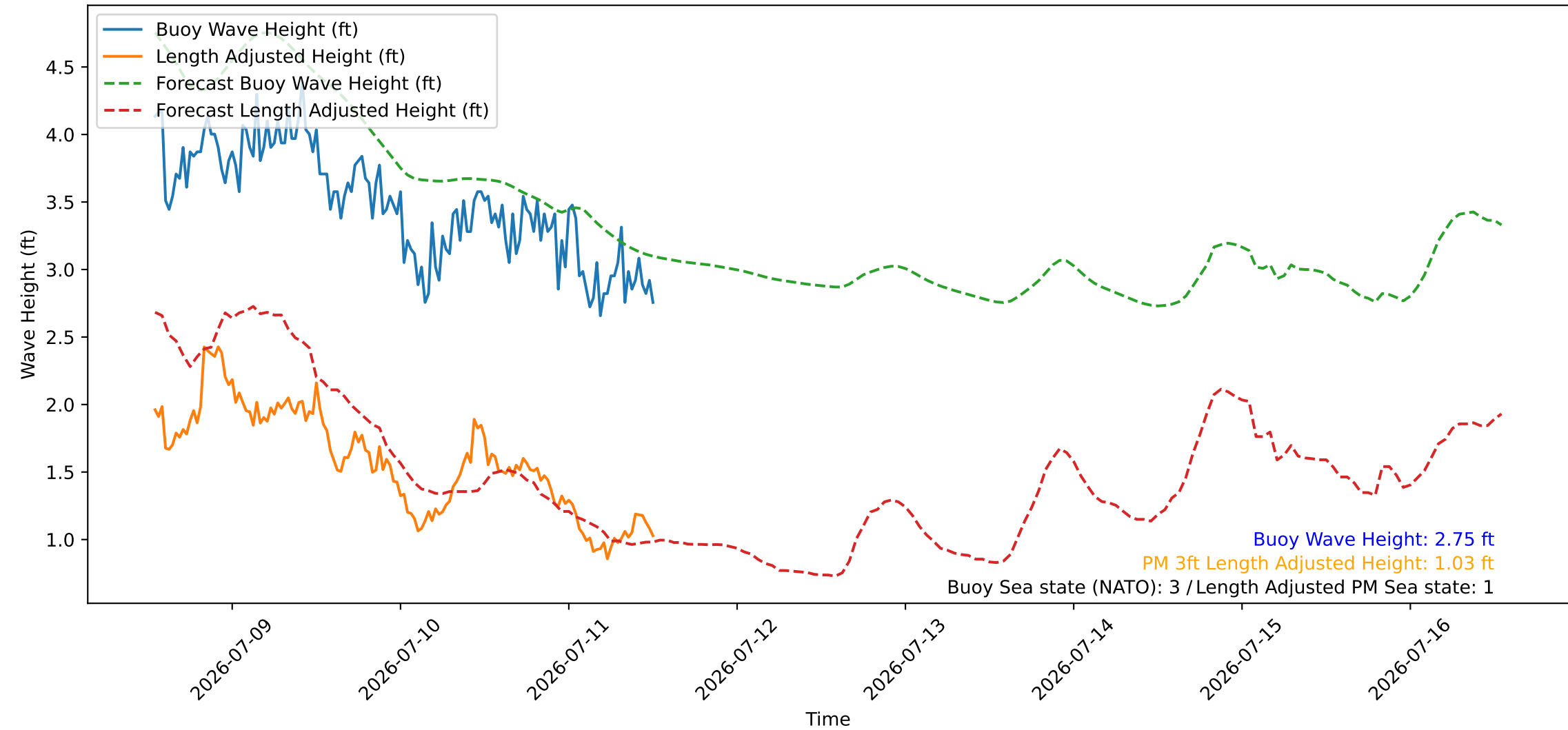
Wave Heights over Time for Green Beach at 2026-07-11 12:51:09
