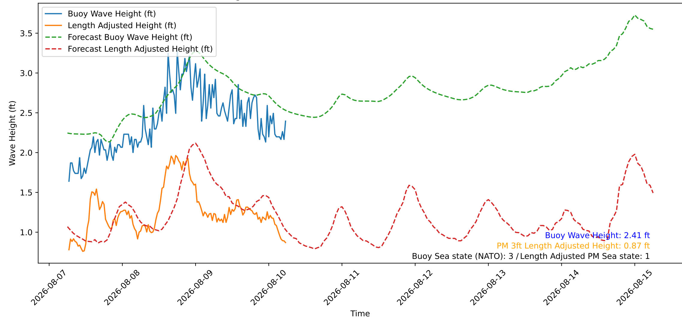
Wave Heights over Time for Oceanside Harbor at 2026-08-10 06:20:27
