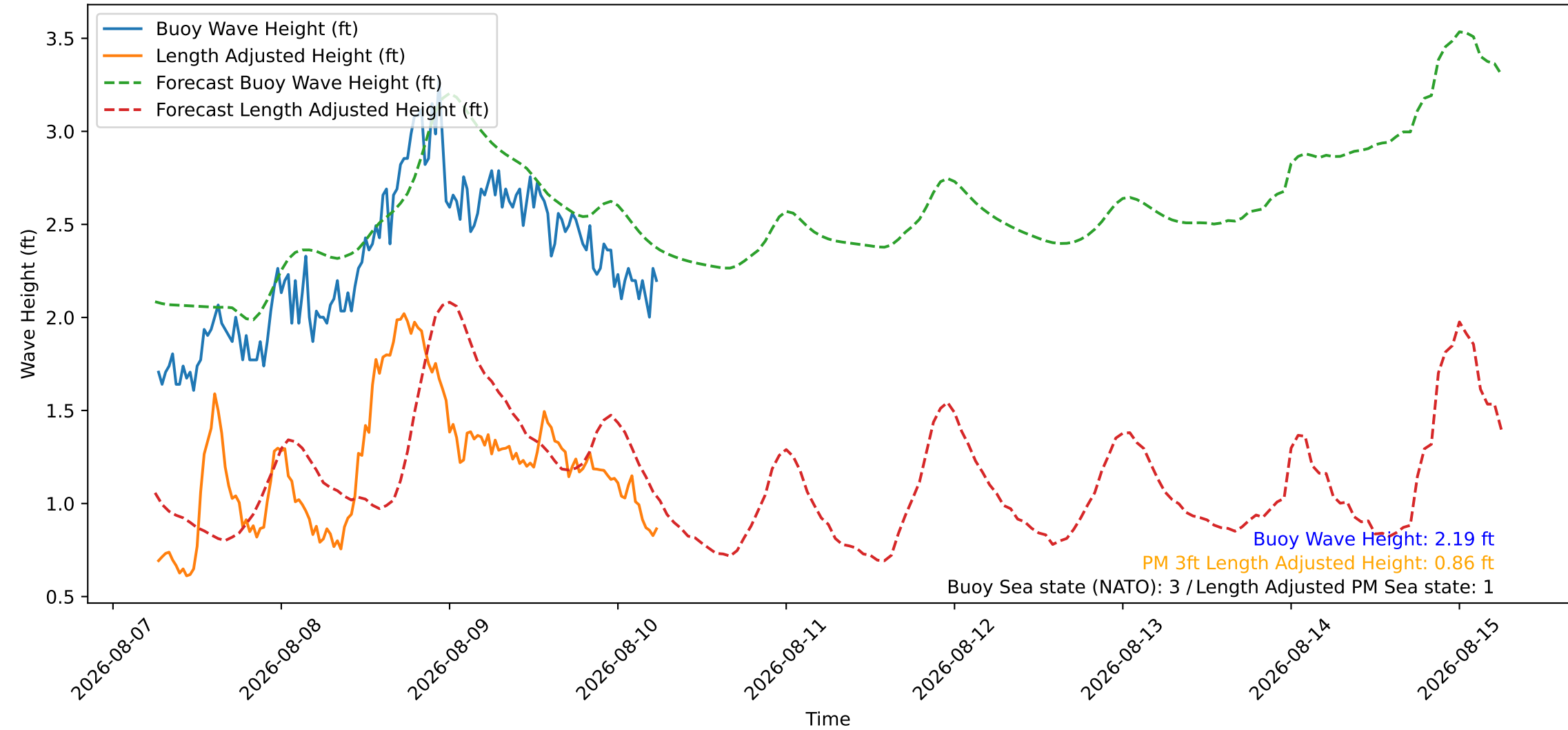
Wave Heights over Time for Red Beach at 2026-08-10 06:20:48
