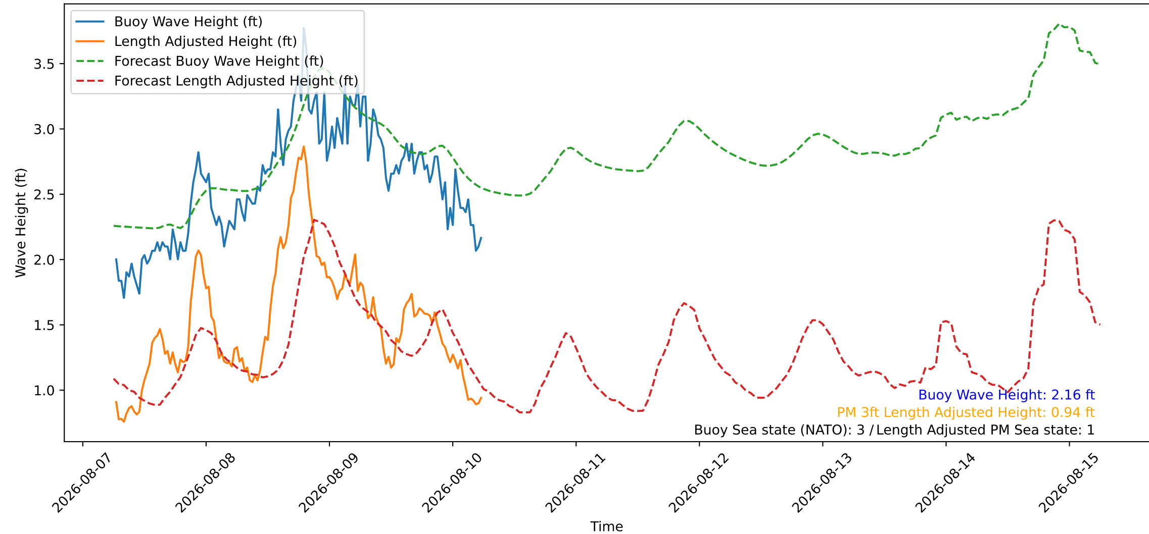
Wave Heights over Time for Green Beach at 2026-08-10 06:21:11
