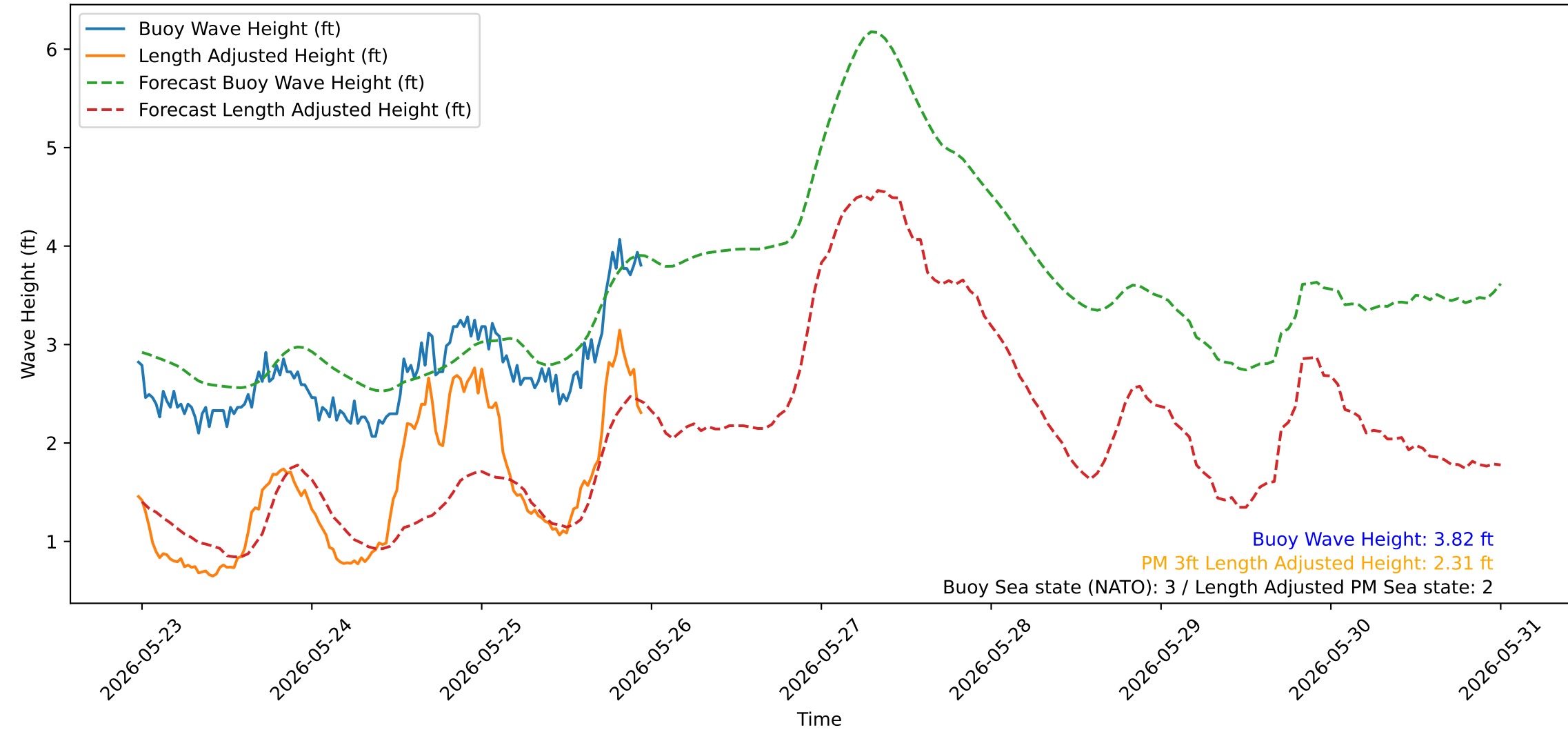
Wave Heights over Time for Green Beach at 2026-05-25 23:31:12
