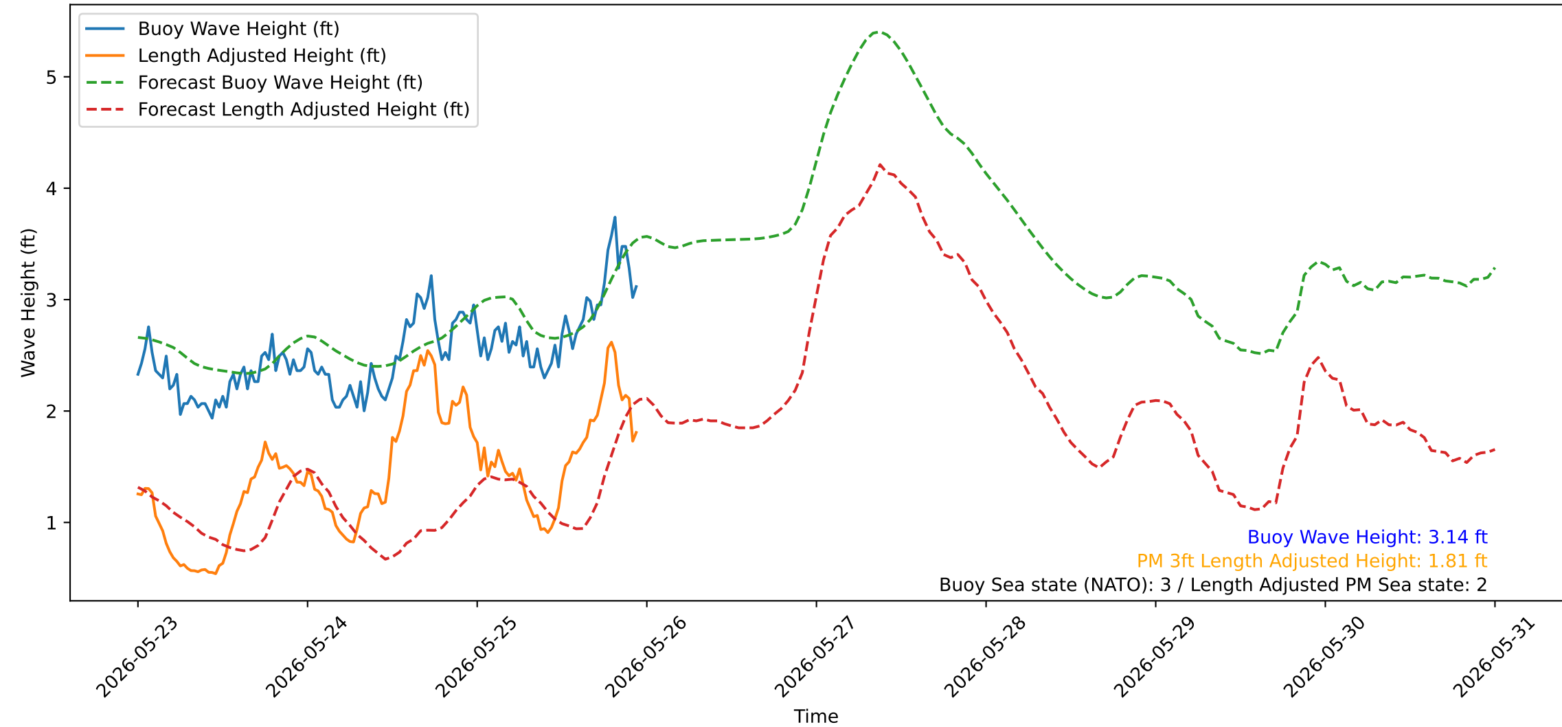
Wave Heights over Time for Red Beach at 2026-05-25 23:30:49
