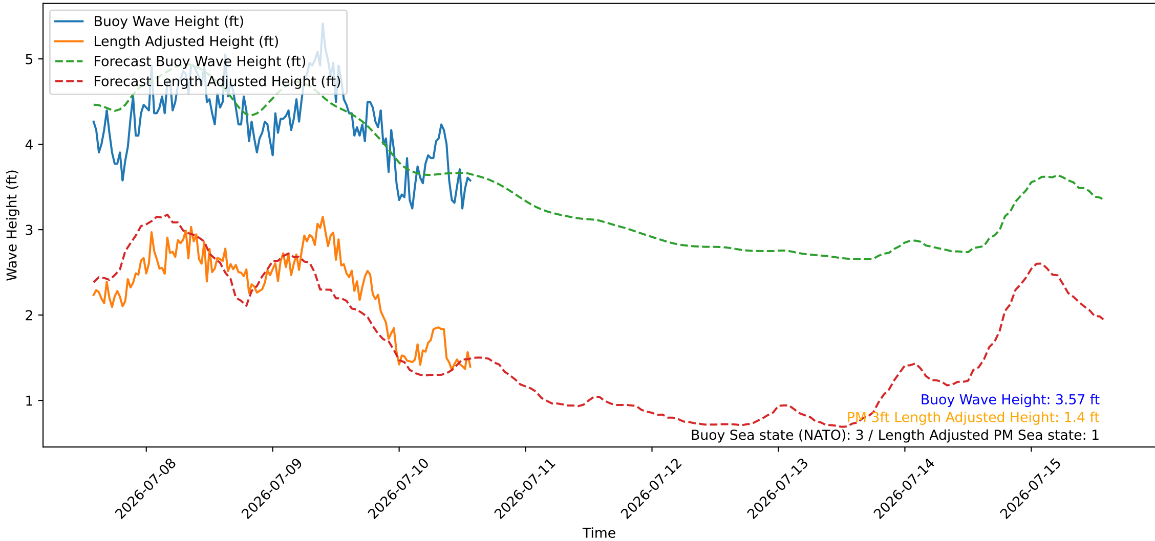
Wave Heights over Time for Oceanside Harbor at 2026-07-10 14:00:26
