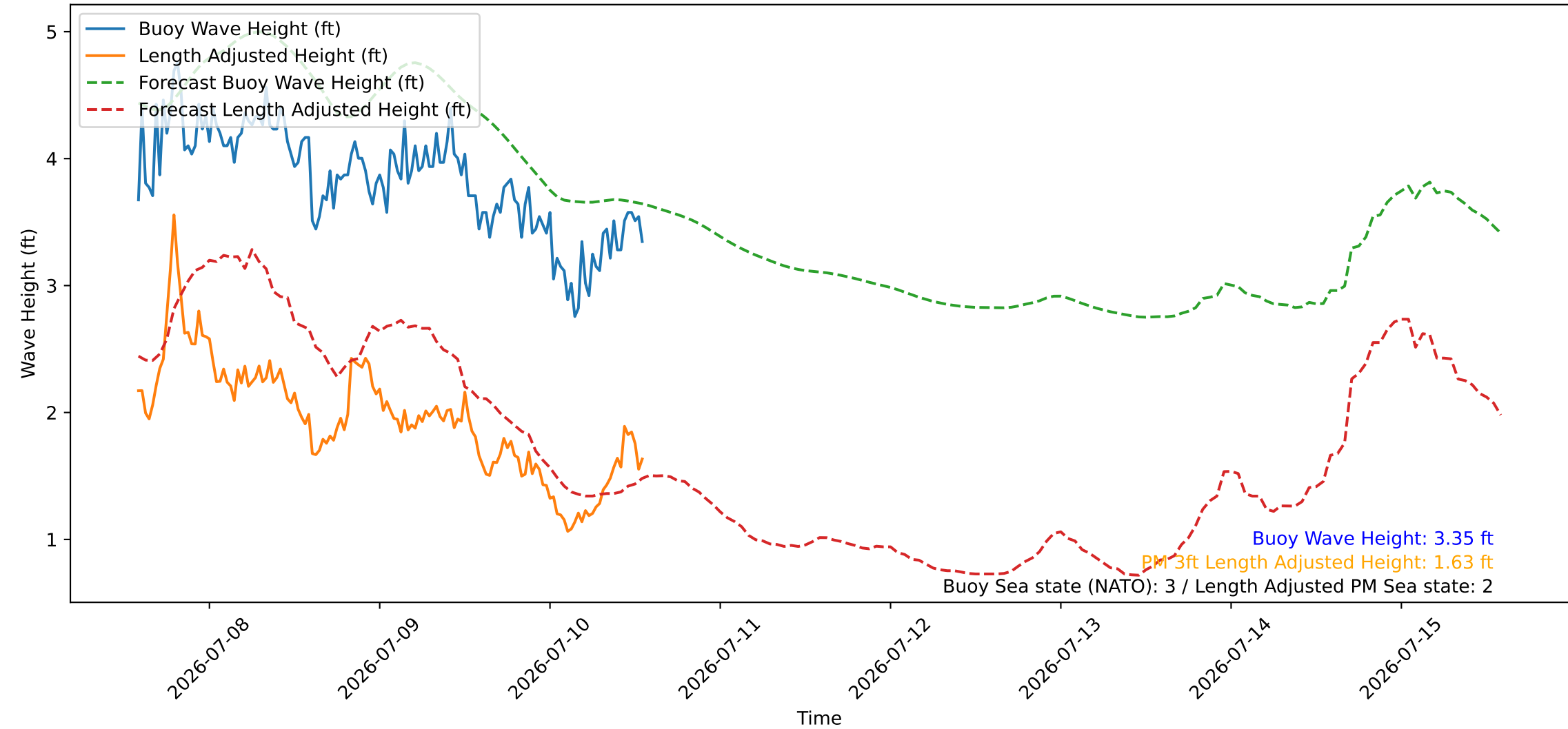
Wave Heights over Time for Green Beach at 2026-07-10 14:01:08
