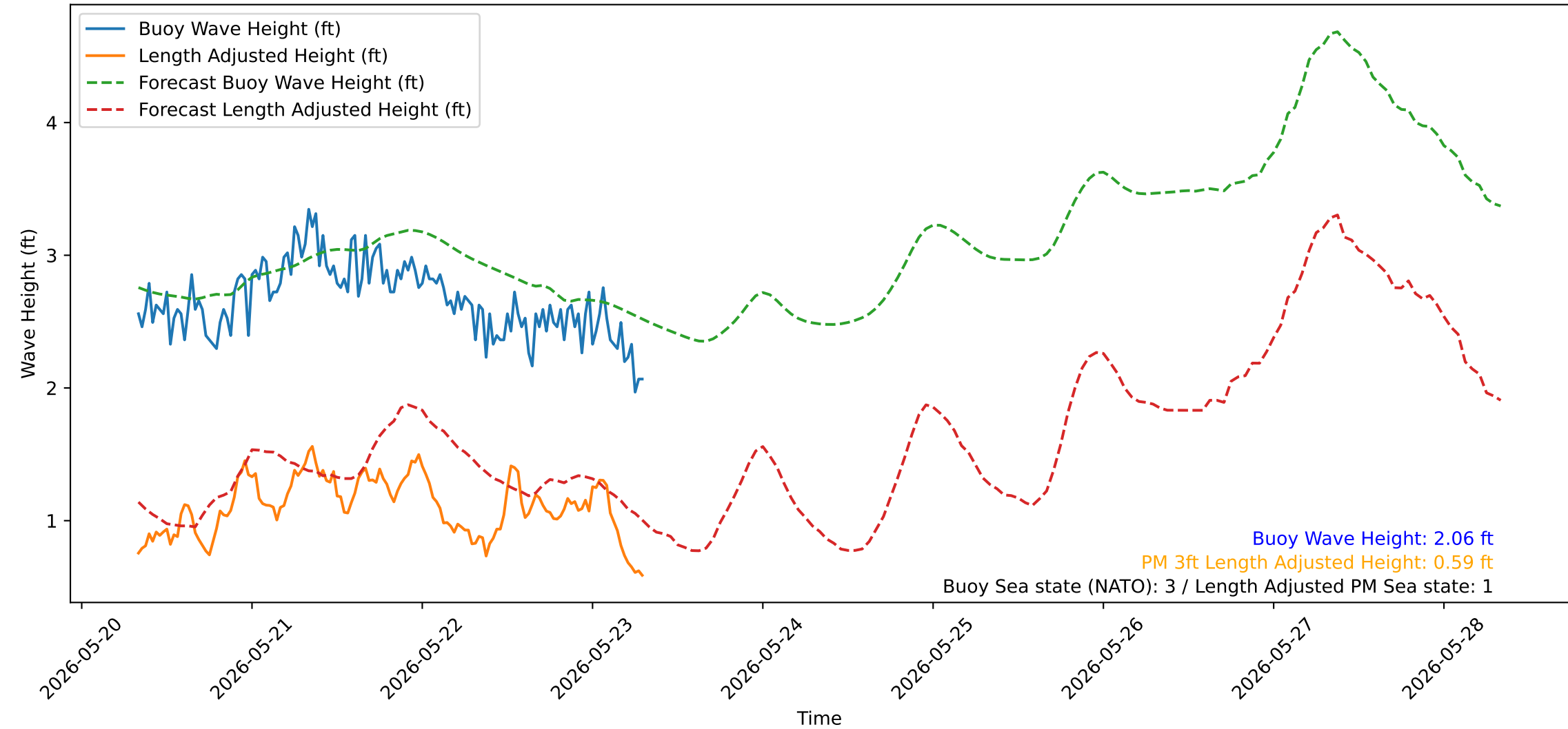
Wave Heights over Time for Red Beach at 2026-05-23 07:50:52
