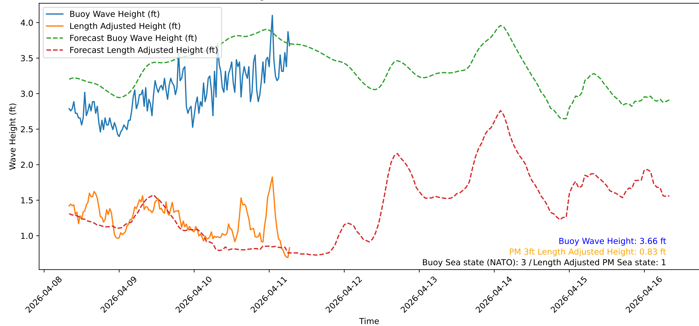
Wave Heights over Time for Red Beach at 2026-04-11 07:30:51
