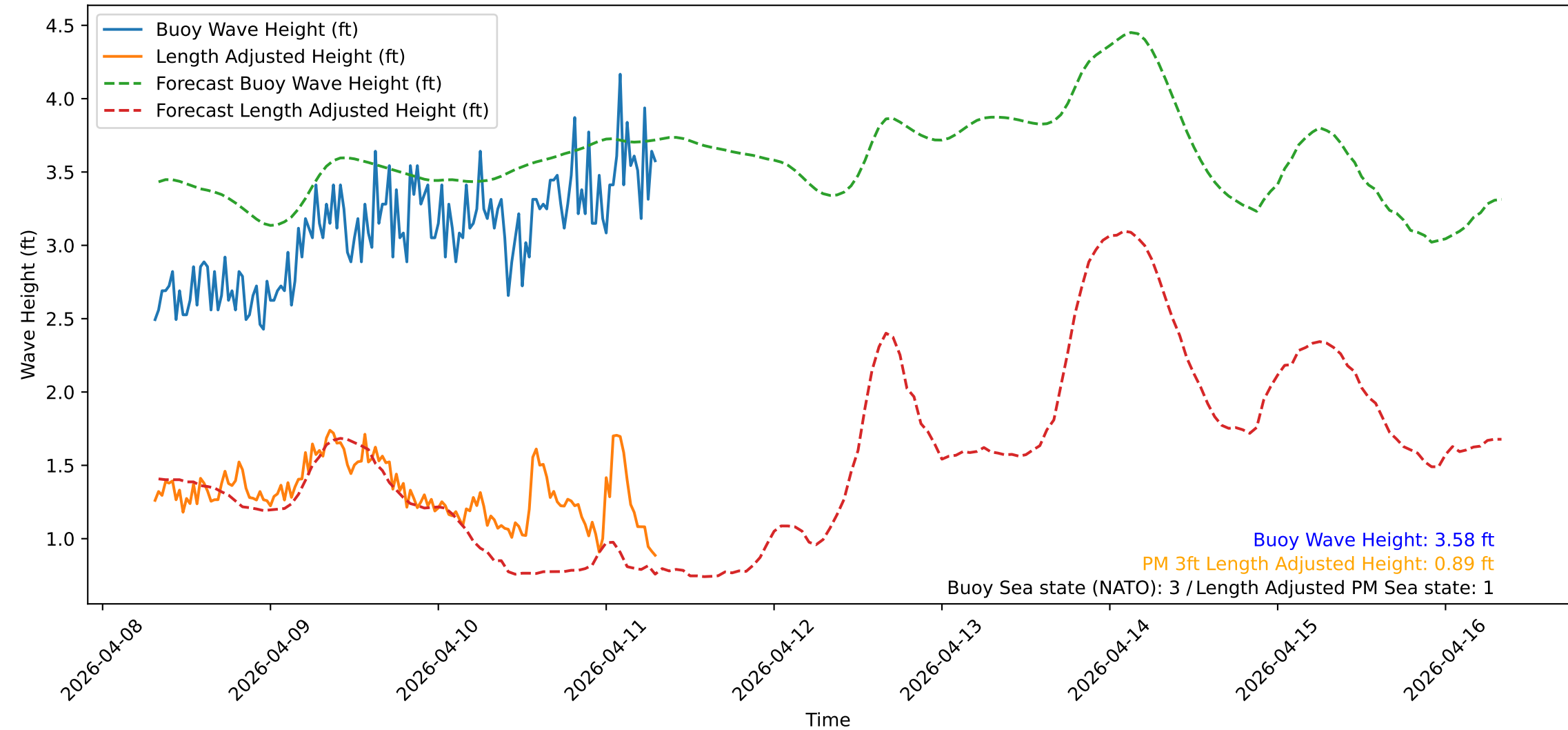
Wave Heights over Time for Oceanside Harbor at 2026-04-11 07:30:31
