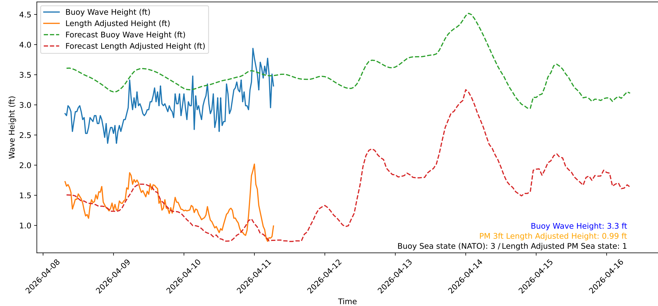
Wave Heights over Time for Green Beach at 2026-04-11 07:31:13
