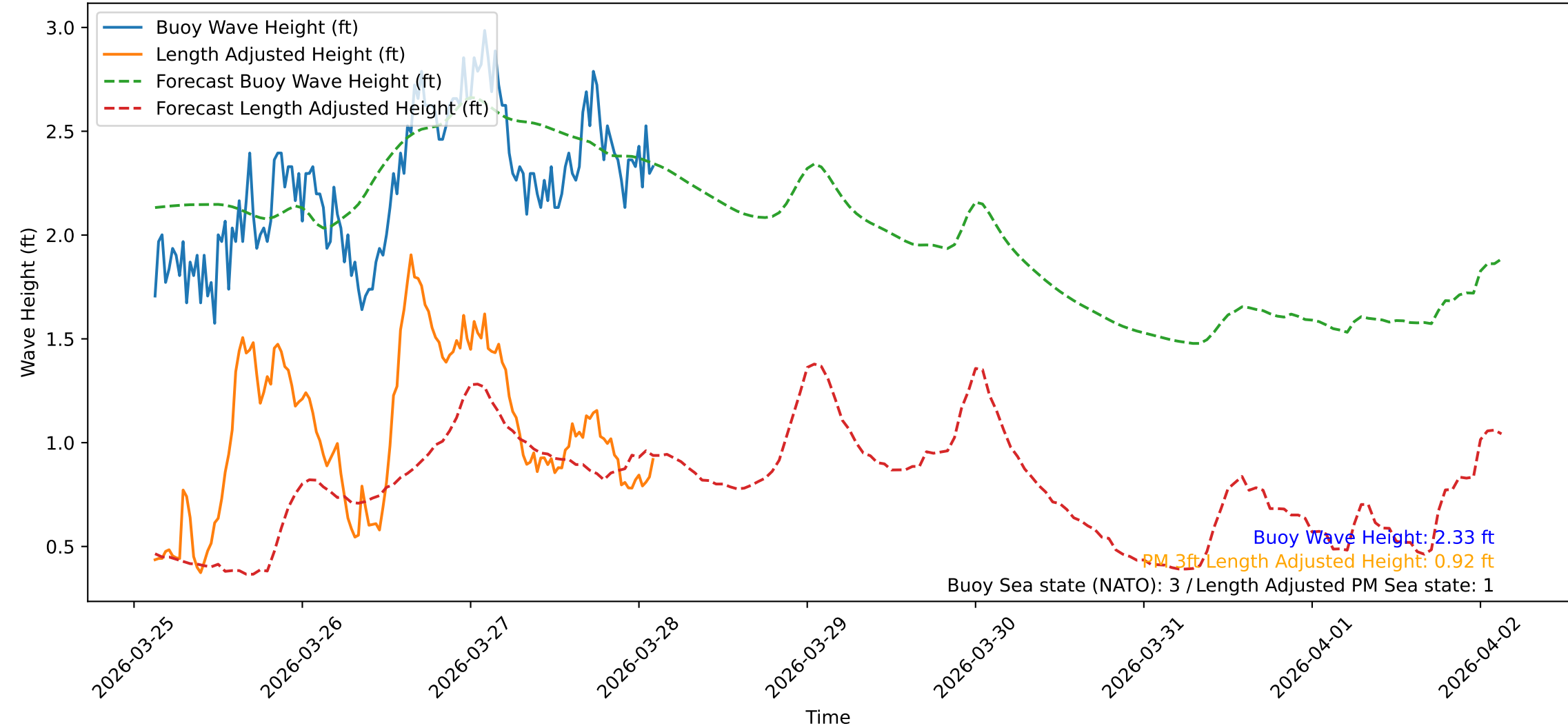
Wave Heights over Time for Red Beach at 2026-03-28 02:40:47
