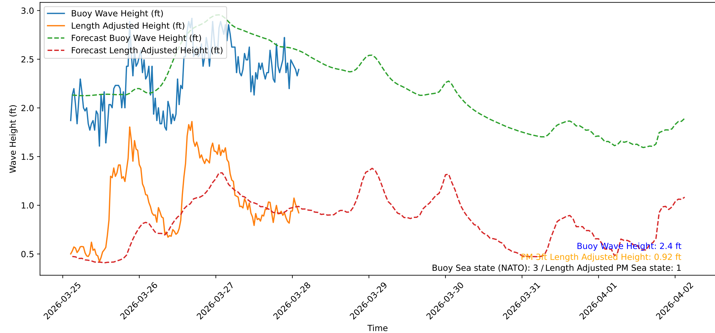
Wave Heights over Time for Oceanside Harbor at 2026-03-28 02:40:31
