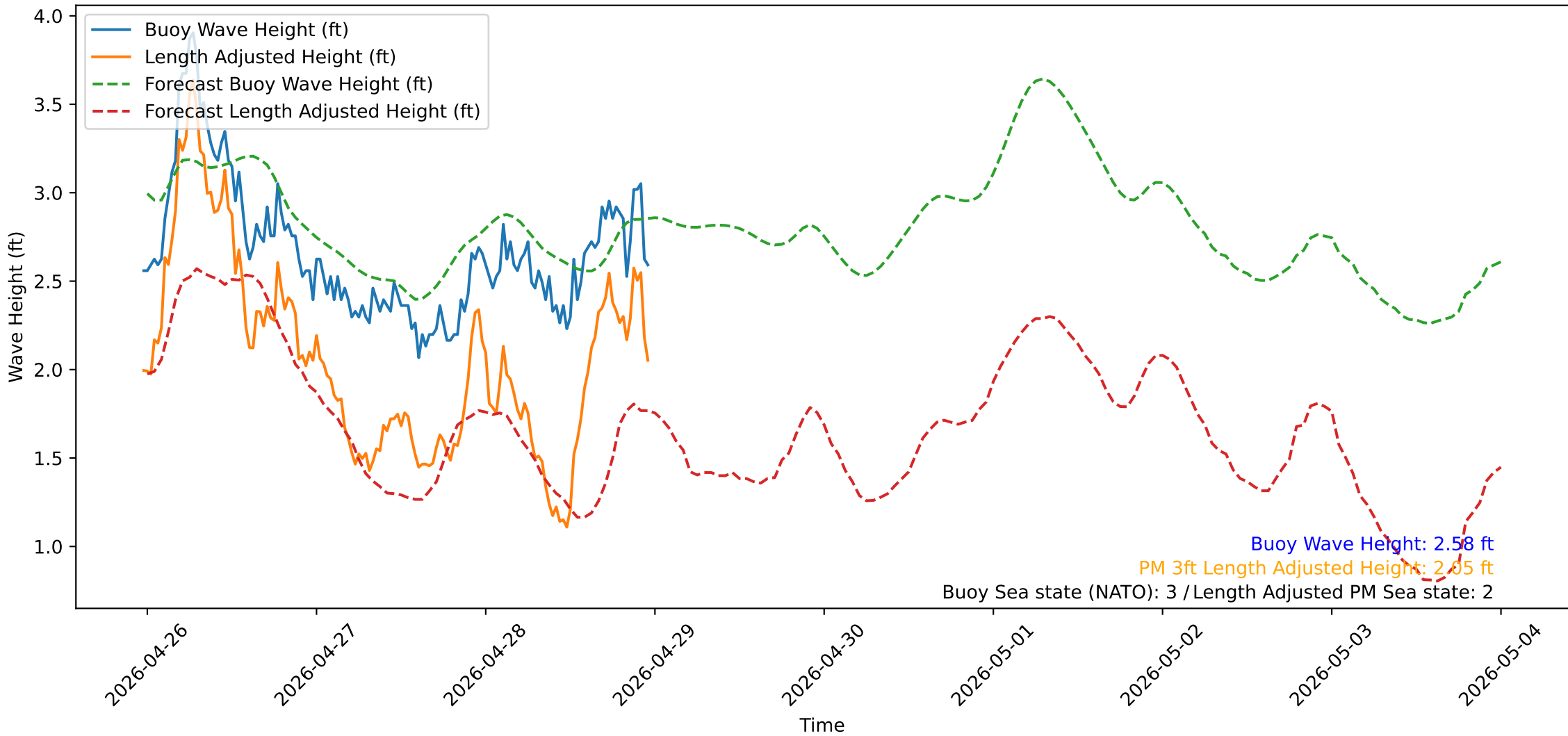
Wave Heights over Time for Oceanside Harbor at 2026-04-28 23:40:31
