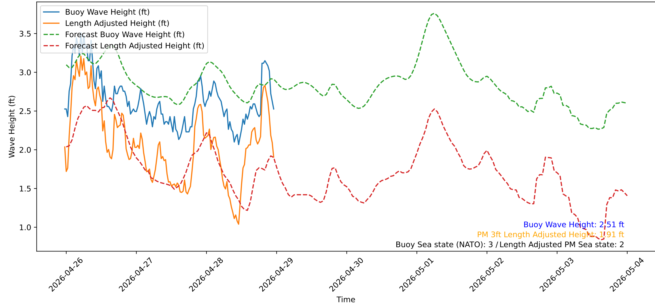
Wave Heights over Time for Green Beach at 2026-04-28 23:41:13
