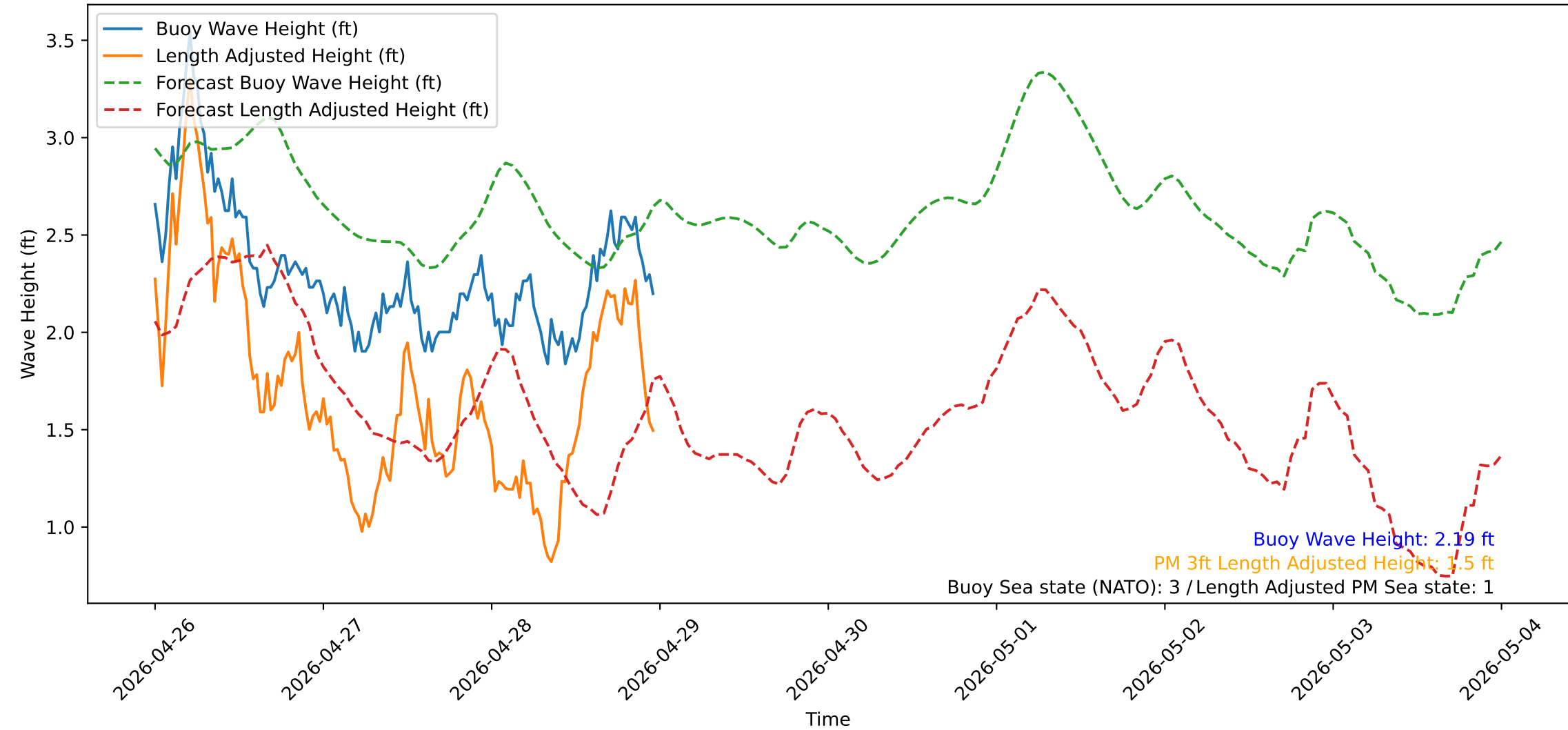
Wave Heights over Time for Red Beach at 2026-04-28 23:40:50
