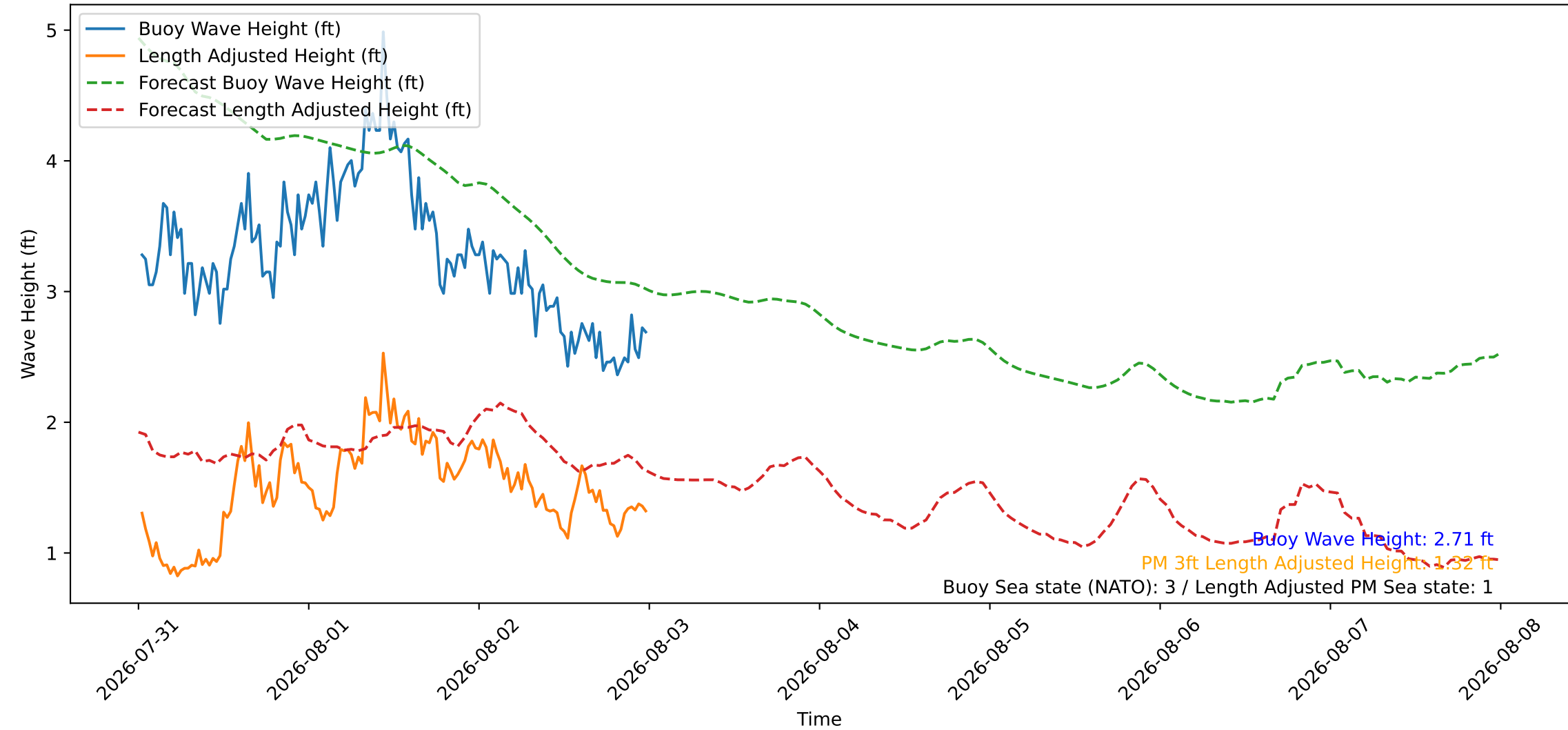
Wave Heights over Time for Green Beach at 2026-08-03 00:21:09
