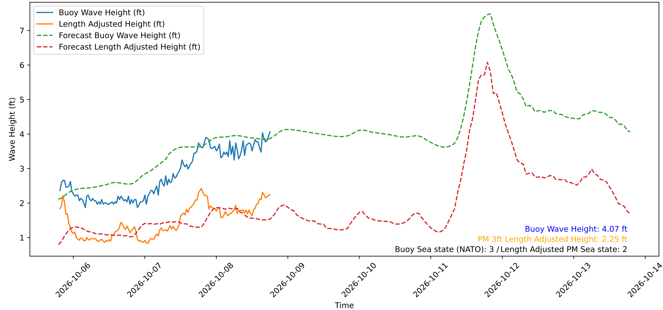
Wave Heights over Time for Red Beach at 2026-10-08 19:00:49
