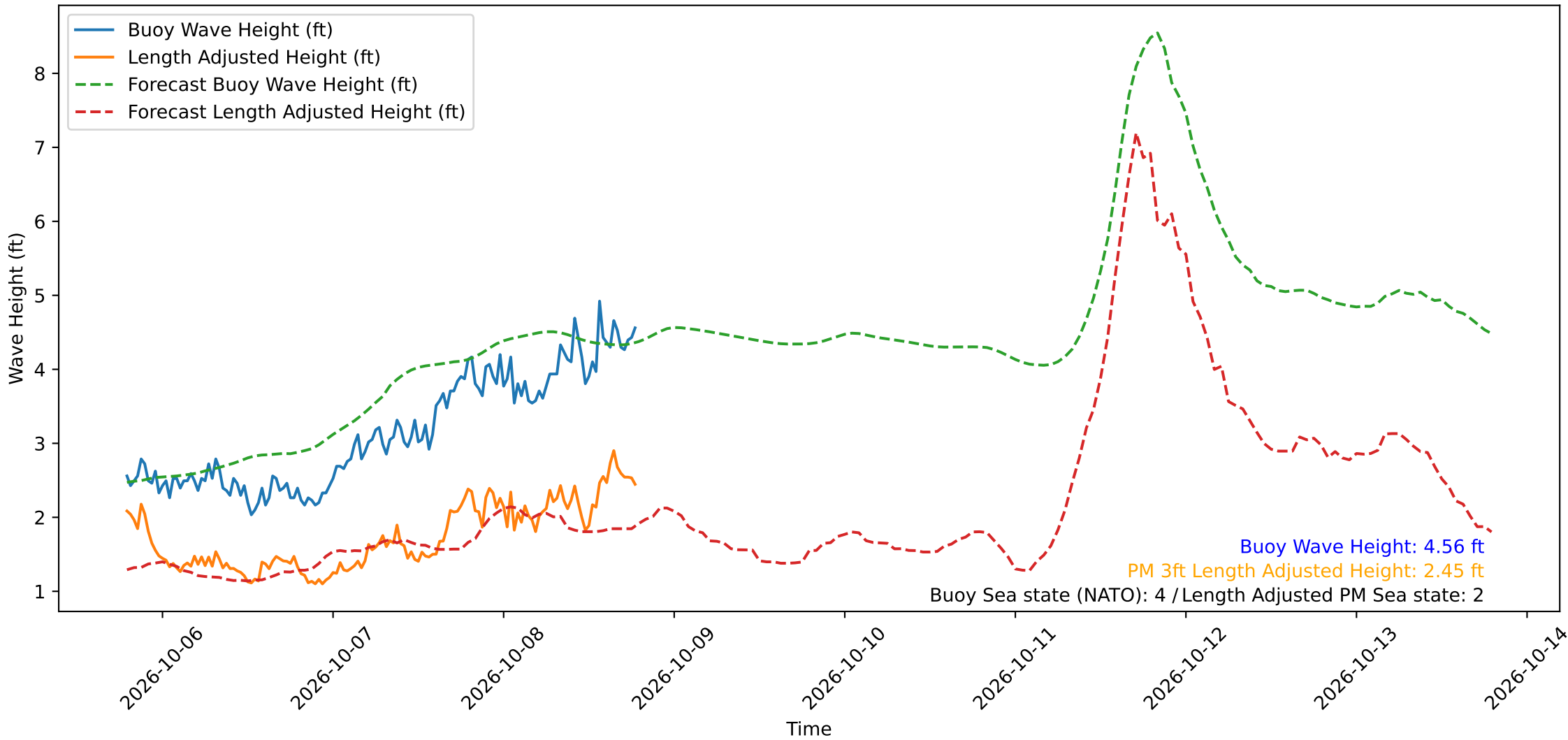
Wave Heights over Time for Oceanside Harbor at 2026-10-08 19:00:29
