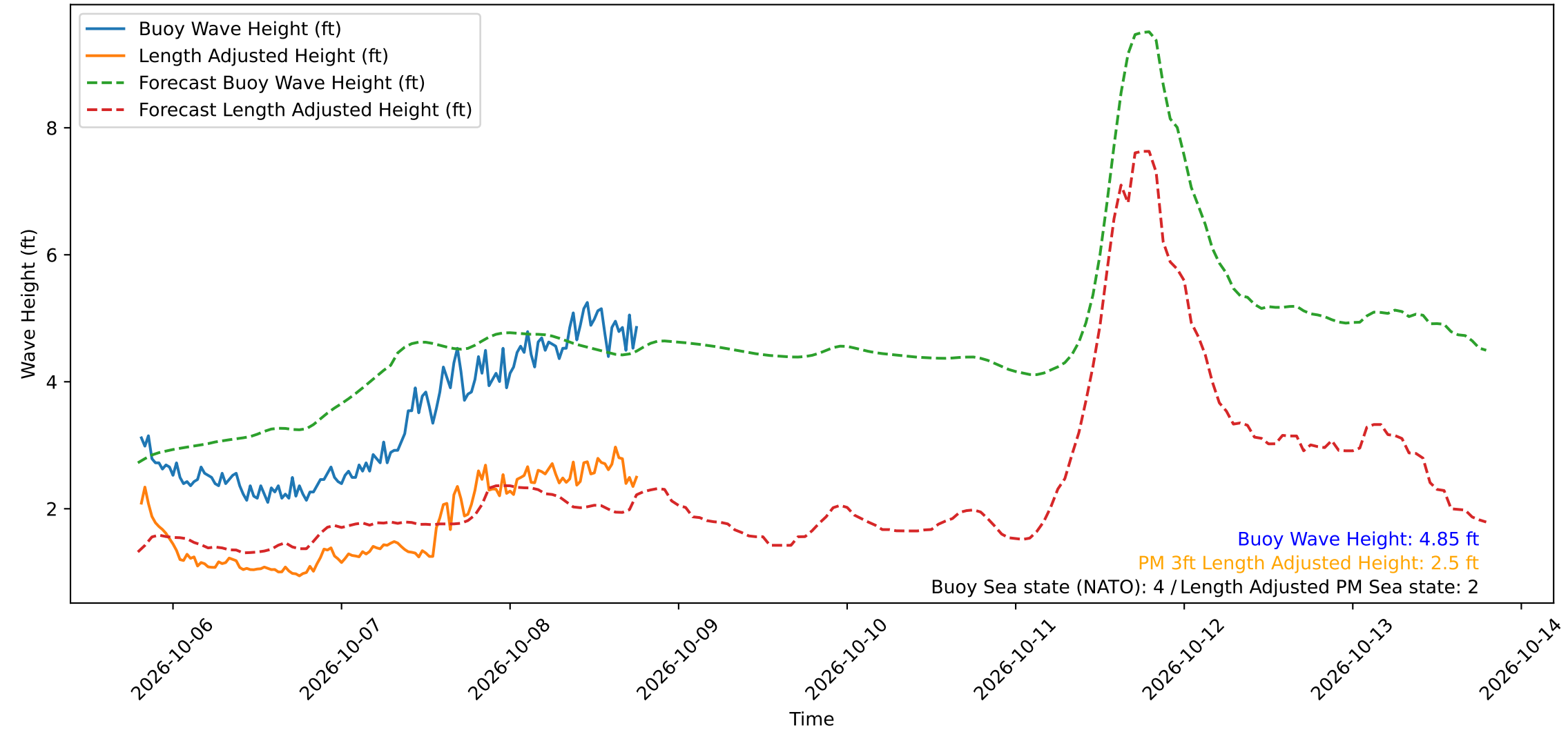
Wave Heights over Time for Green Beach at 2026-10-08 19:01:11
