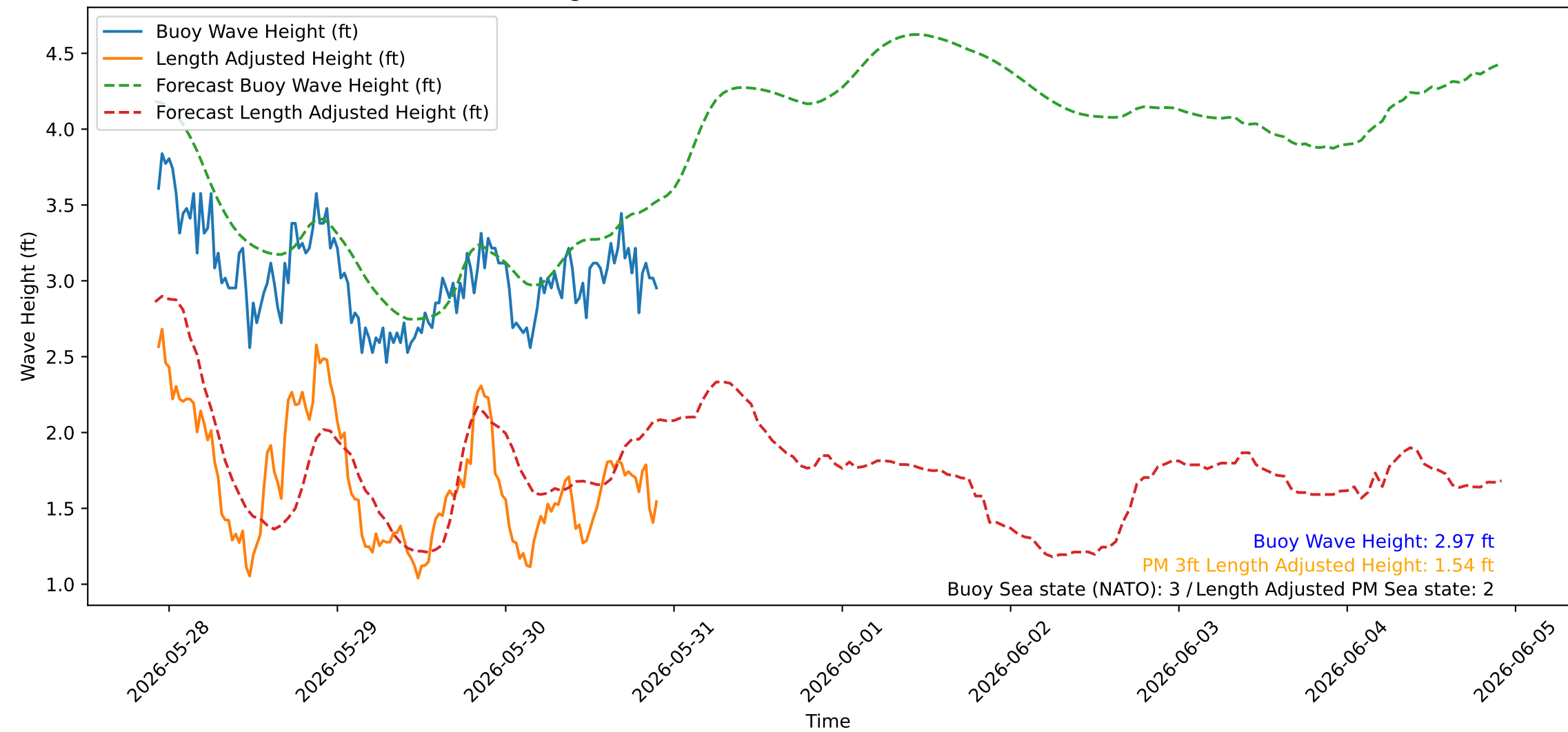
Wave Heights over Time for Green Beach at 2026-05-30 22:21:07
