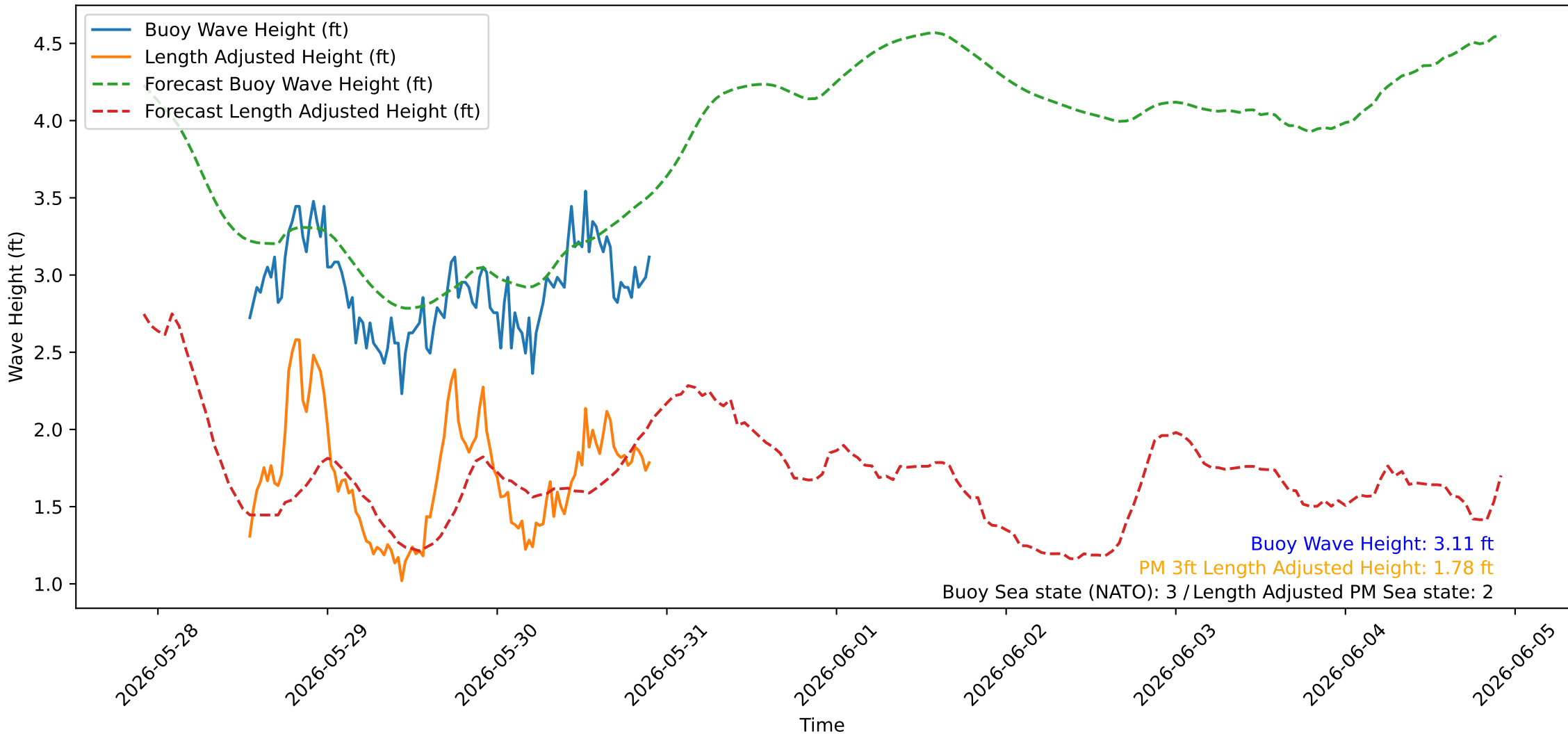
Wave Heights over Time for Oceanside Harbor at 2026-05-30 22:20:24
