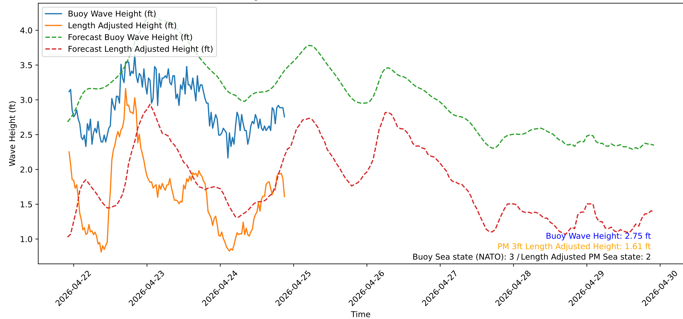
Wave Heights over Time for Red Beach at 2026-04-24 22:00:51
