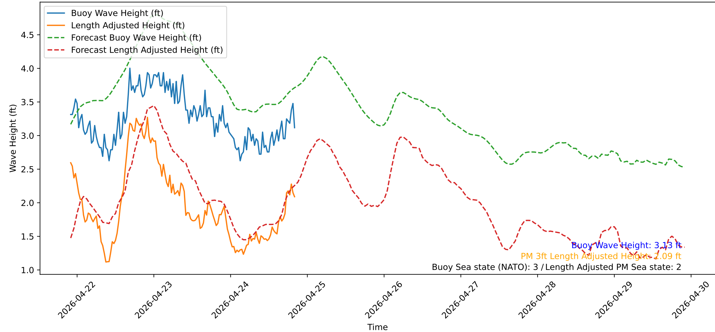
Wave Heights over Time for Green Beach at 2026-04-24 22:01:13
