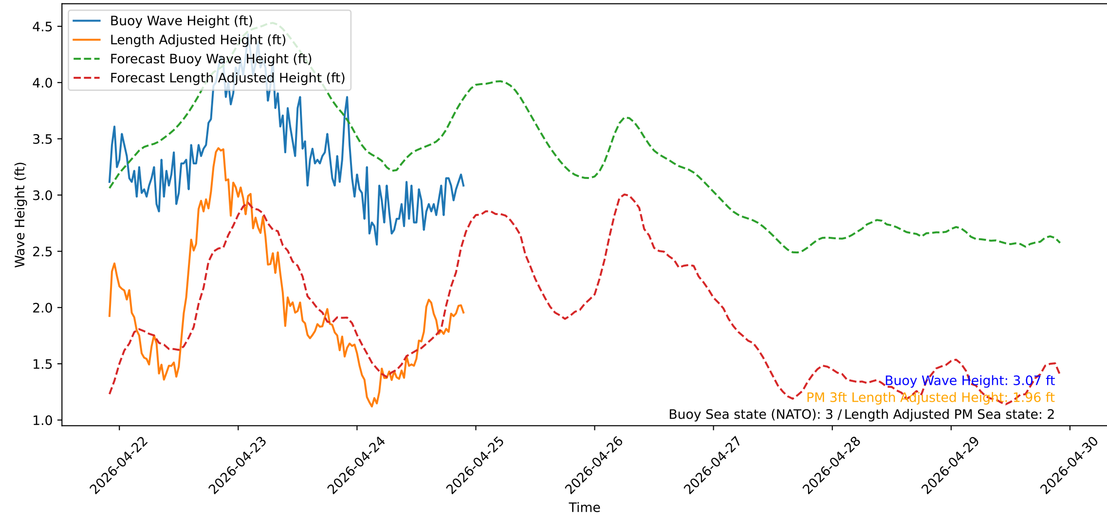
Wave Heights over Time for Oceanside Harbor at 2026-04-24 22:00:31
