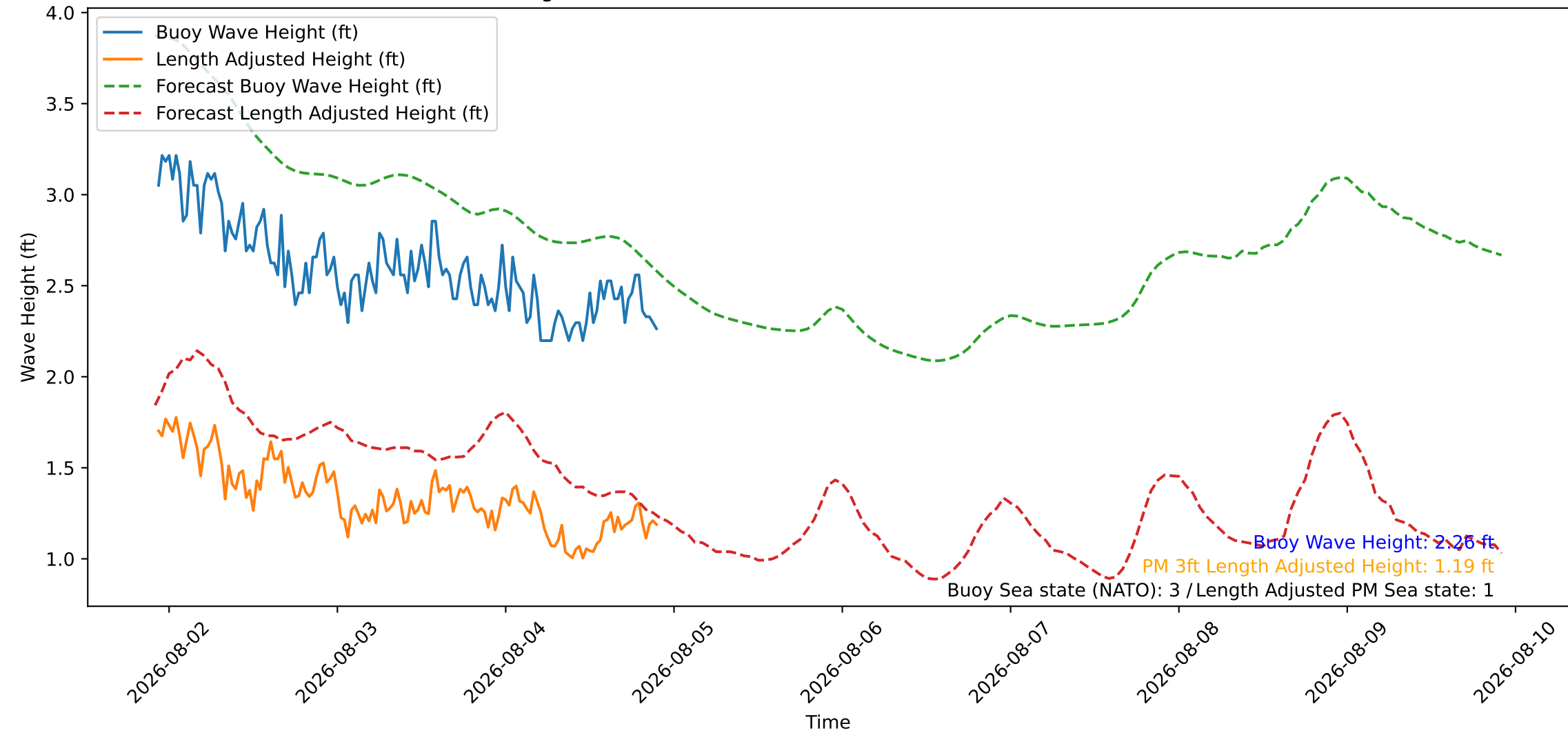
Wave Heights over Time for Oceanside Harbor at 2026-08-04 22:20:26
