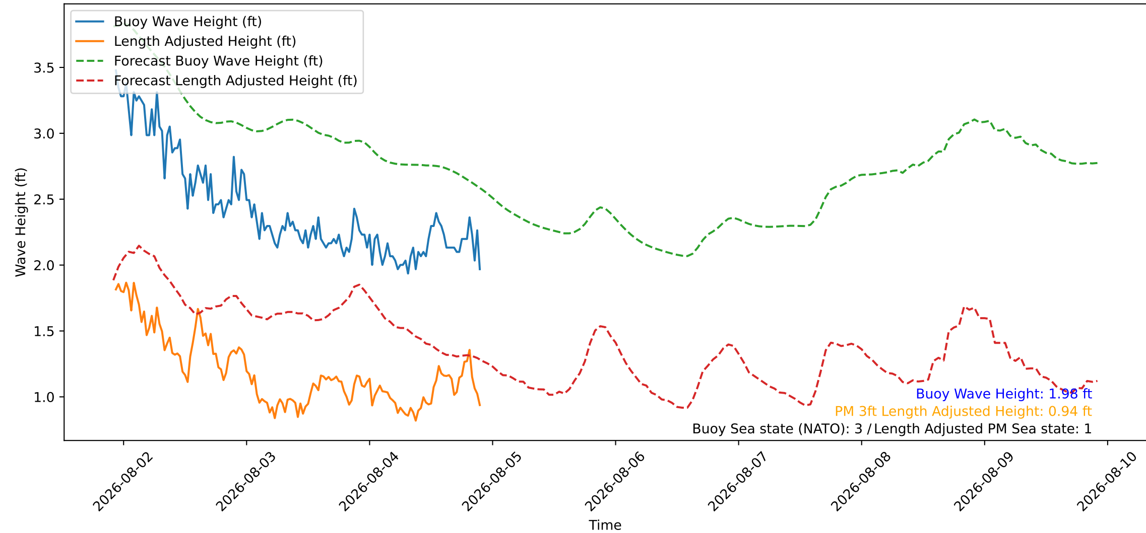
Wave Heights over Time for Green Beach at 2026-08-04 22:21:09
