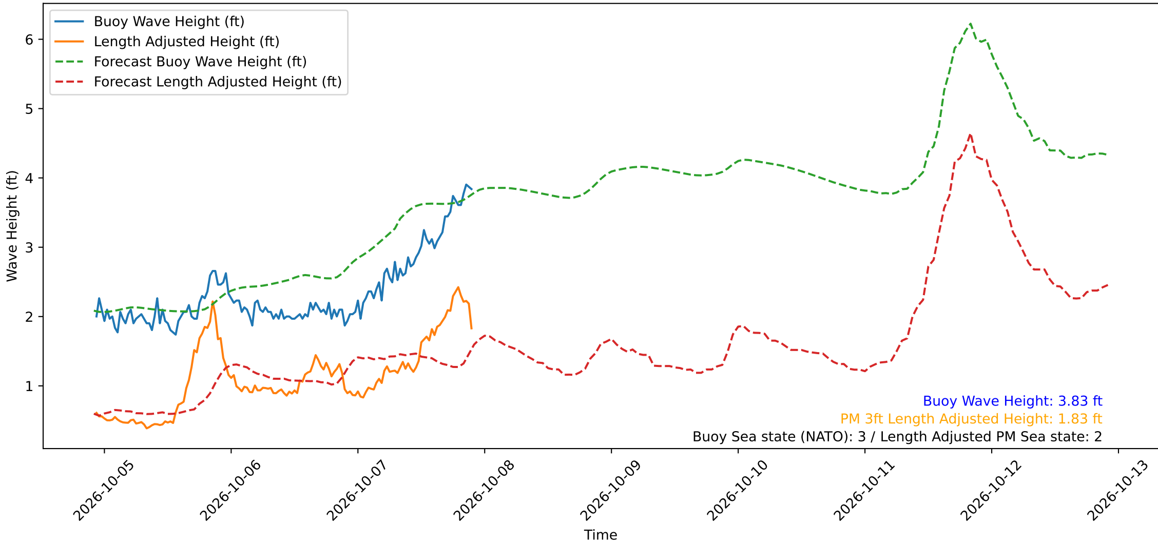
Wave Heights over Time for Red Beach at 2026-10-07 22:20:50
