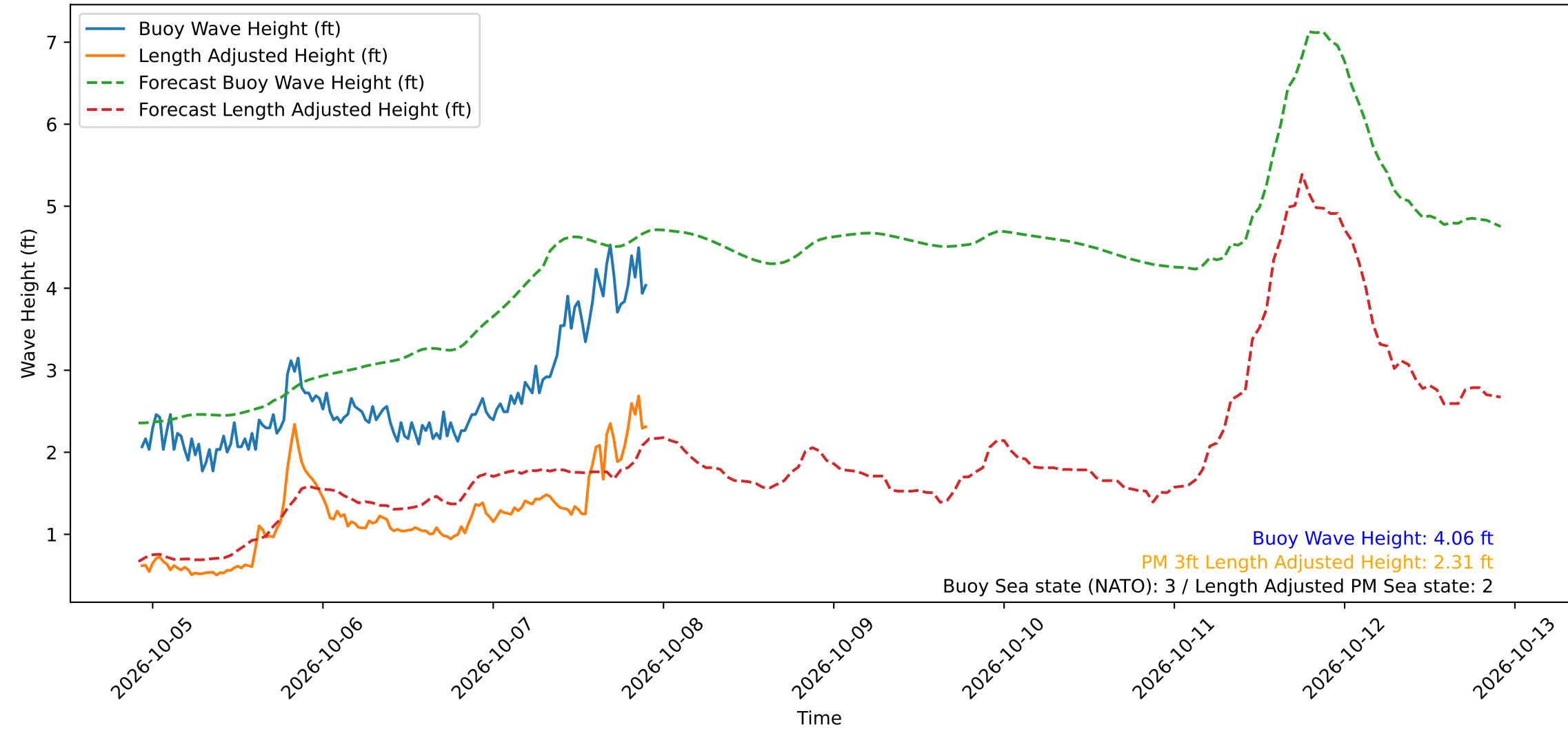
Wave Heights over Time for Green Beach at 2026-10-07 22:21:14
