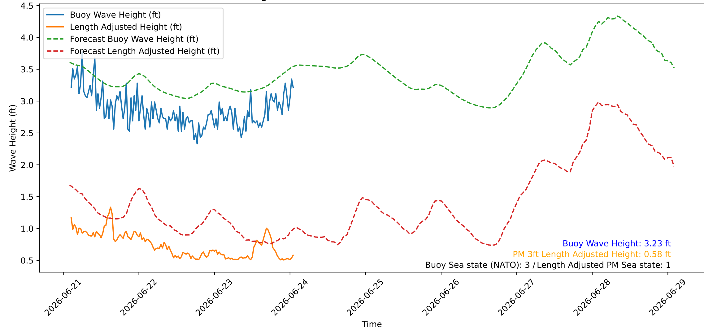
Wave Heights over Time for Red Beach at 2026-06-24 02:00:45
