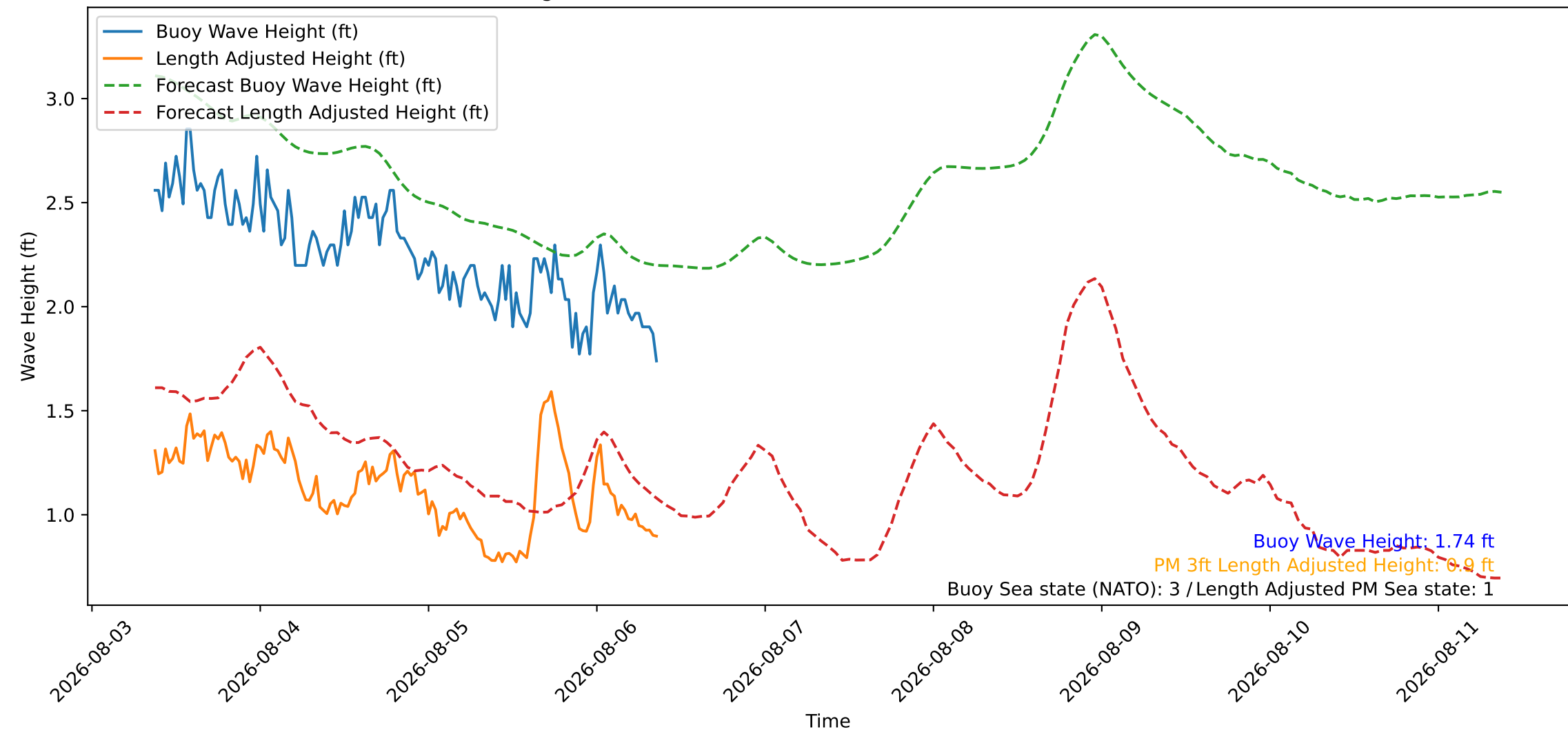
Wave Heights over Time for Oceanside Harbor at 2026-08-06 09:10:27
