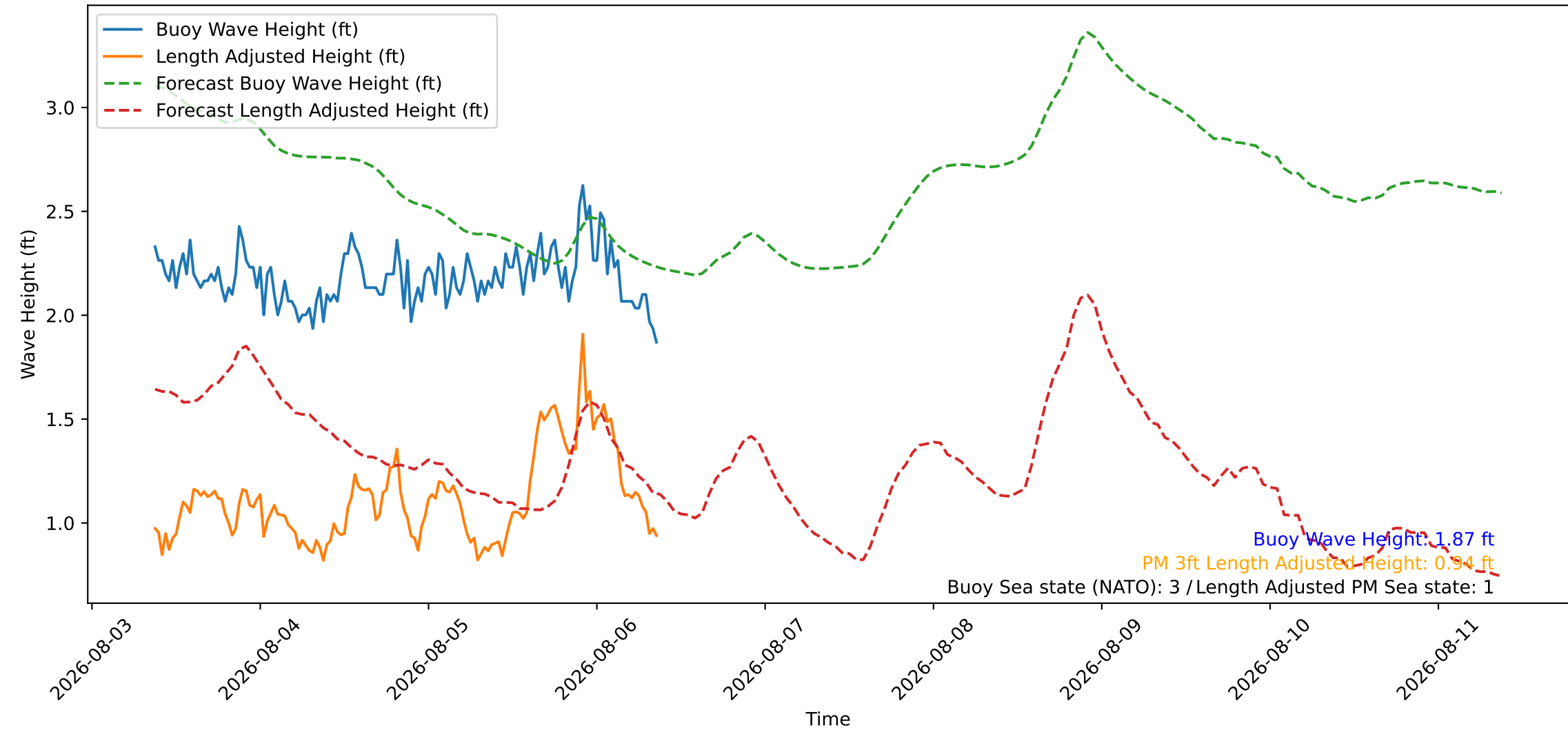
Wave Heights over Time for Green Beach at 2026-08-06 09:11:09
