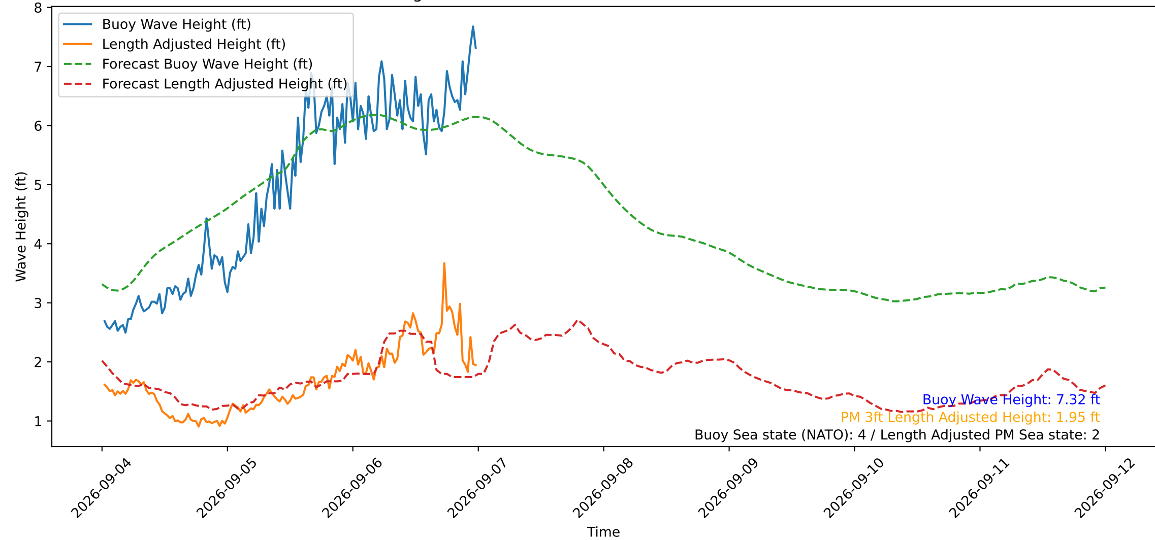
Wave Heights over Time for Green Beach at 2026-09-07 00:21:14
