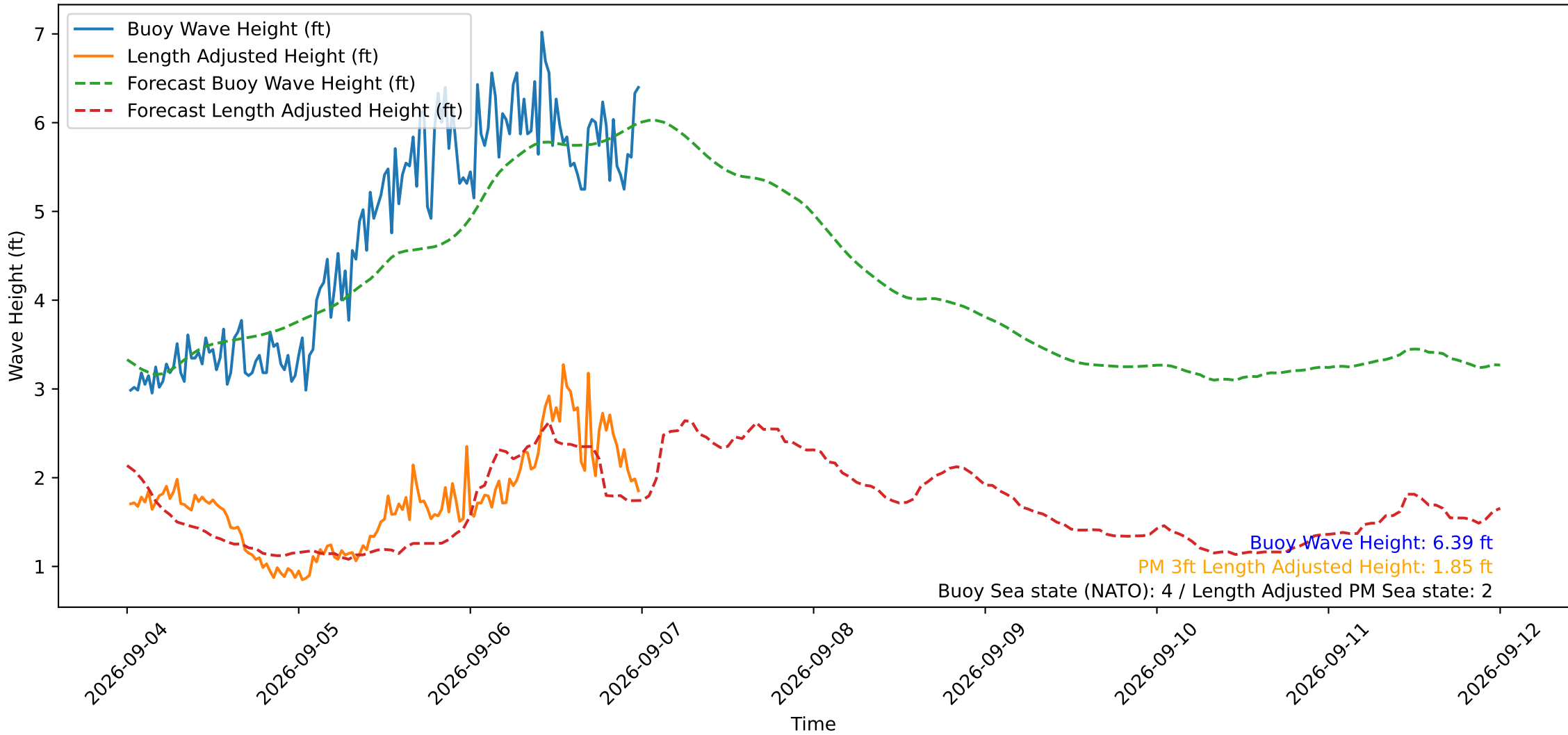
Wave Heights over Time for Oceanside Harbor at 2026-09-07 00:20:29
