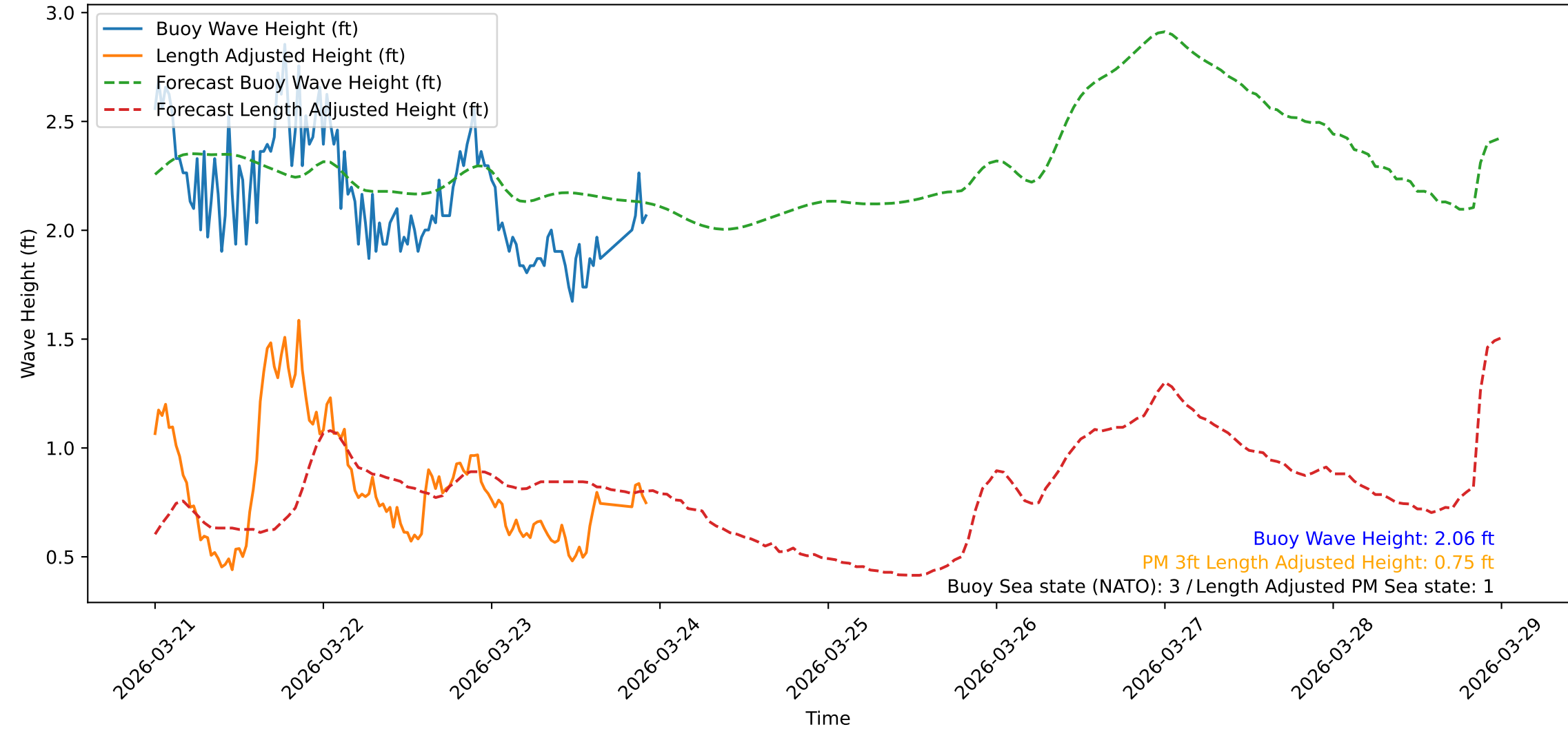
Wave Heights over Time for Red Beach at 2026-03-23 23:30:47
