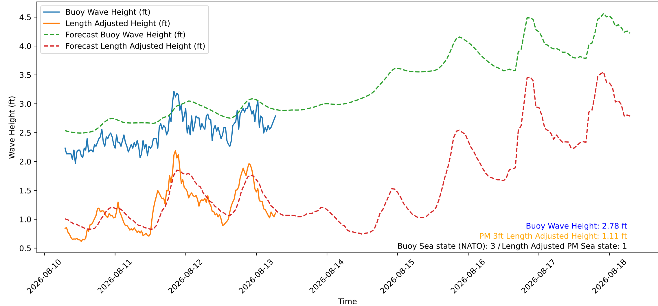
Wave Heights over Time for Green Beach at 2026-08-13 07:11:08
