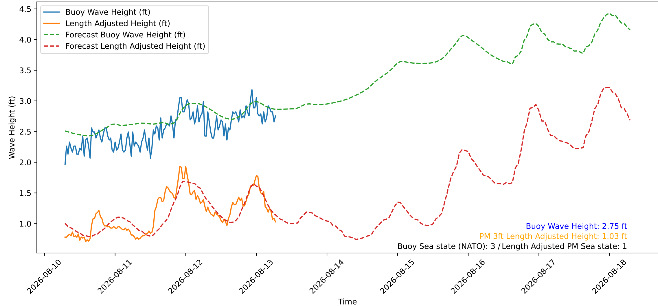
Wave Heights over Time for Oceanside Harbor at 2026-08-13 07:10:26
