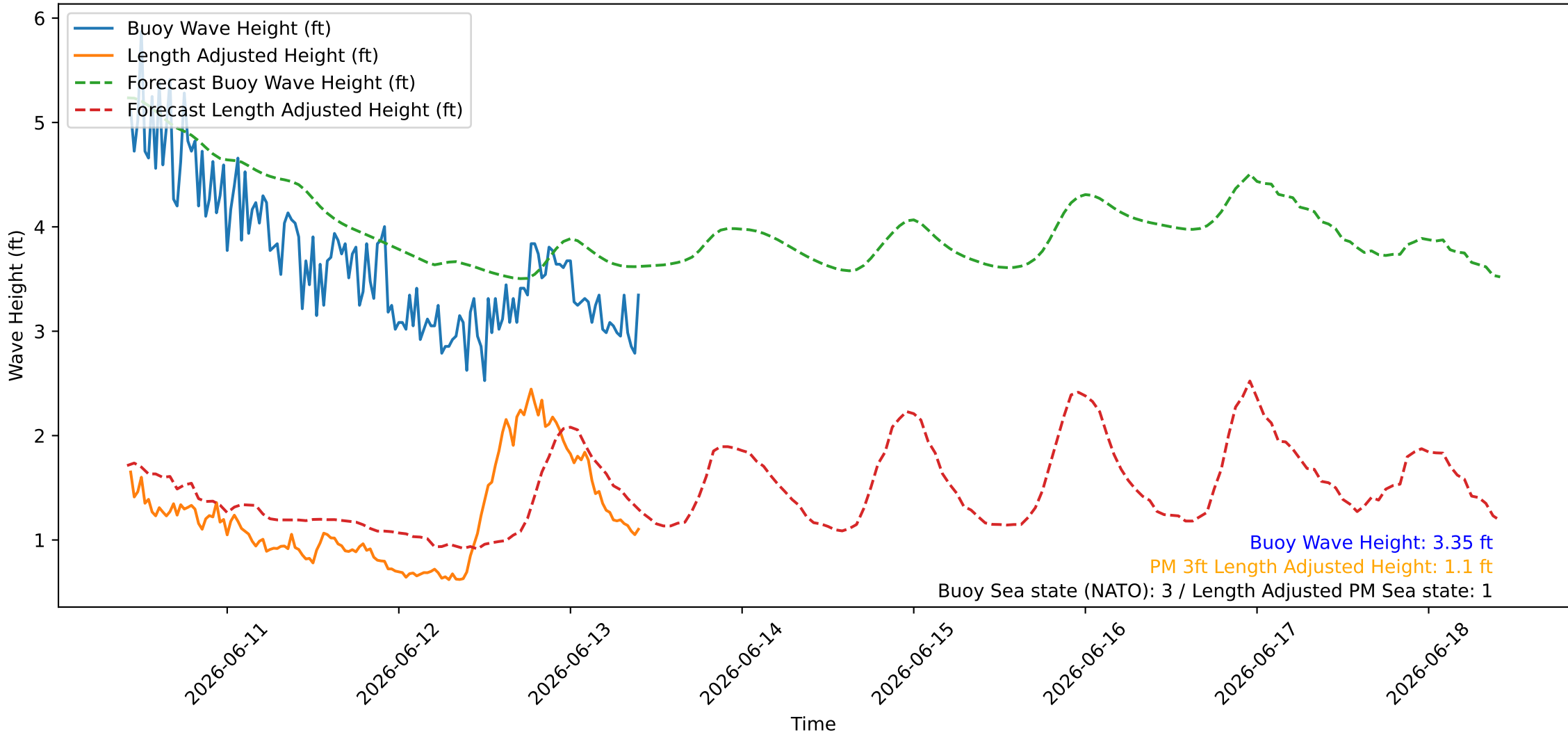
Wave Heights over Time for Red Beach at 2026-06-13 10:20:46
