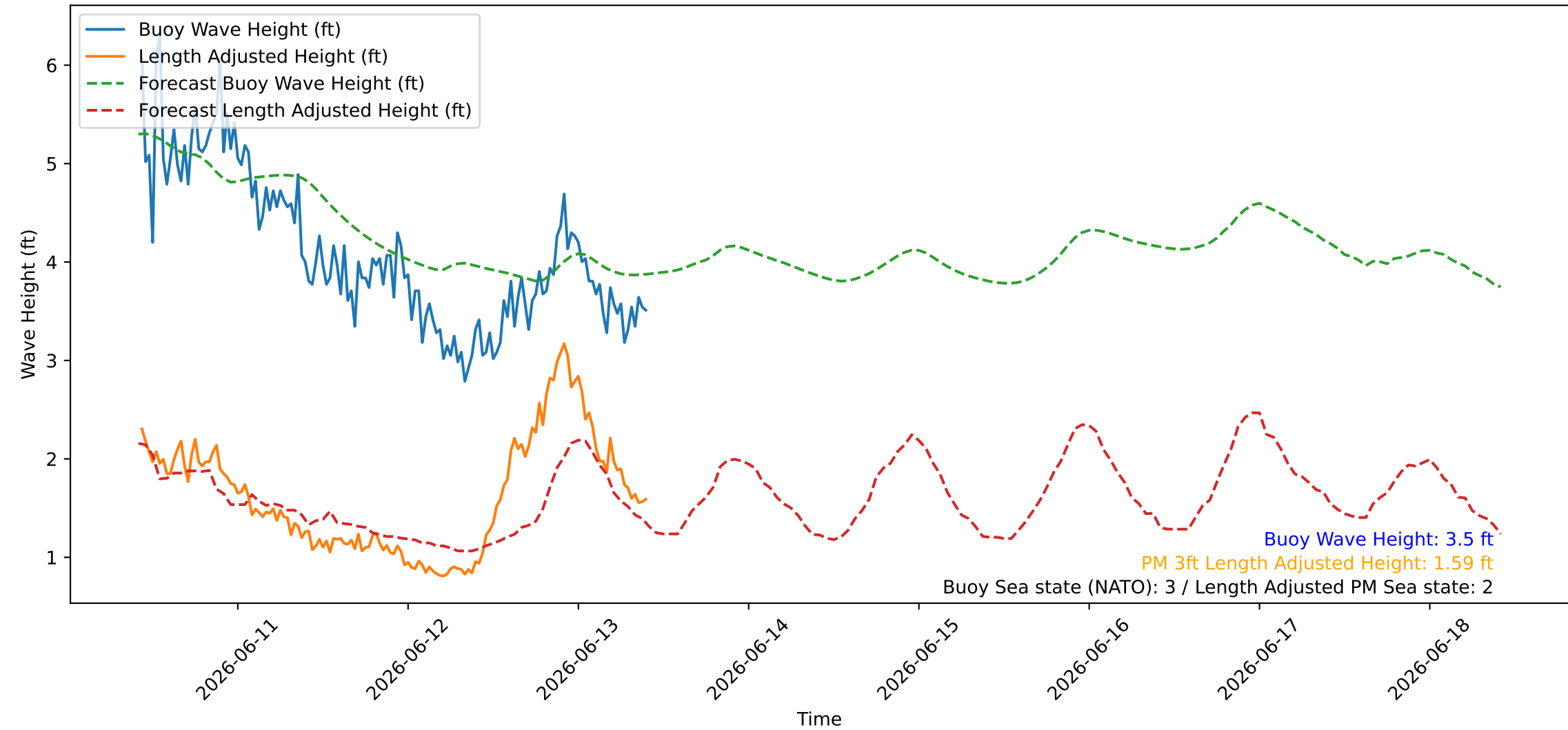
Wave Heights over Time for Oceanside Harbor at 2026-06-13 10:20:26
