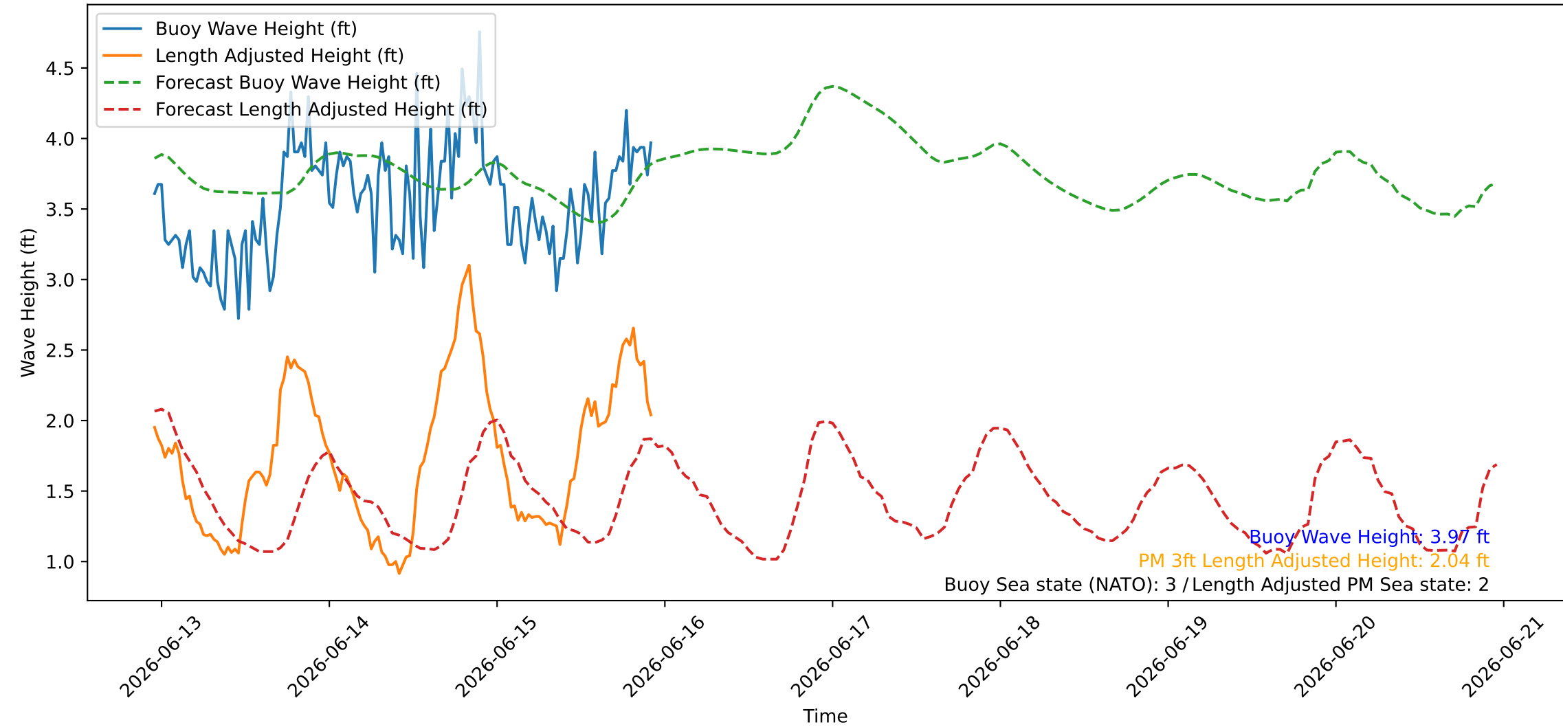
Wave Heights over Time for Red Beach at 2026-06-15 22:50:47
