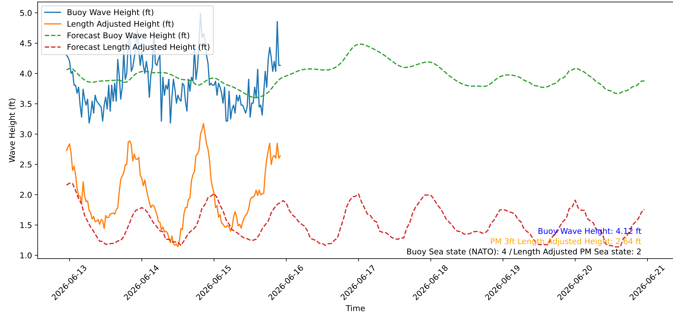
Wave Heights over Time for Oceanside Harbor at 2026-06-15 22:50:26
