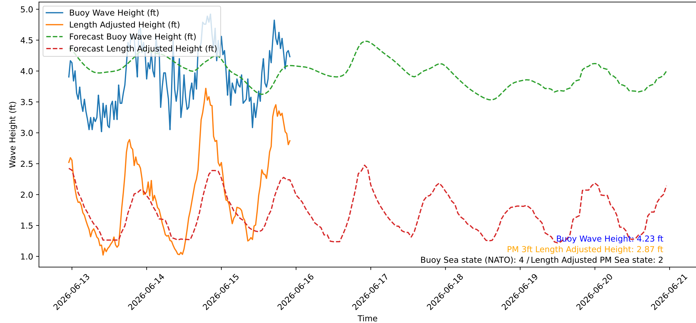
Wave Heights over Time for Green Beach at 2026-06-15 22:51:09
