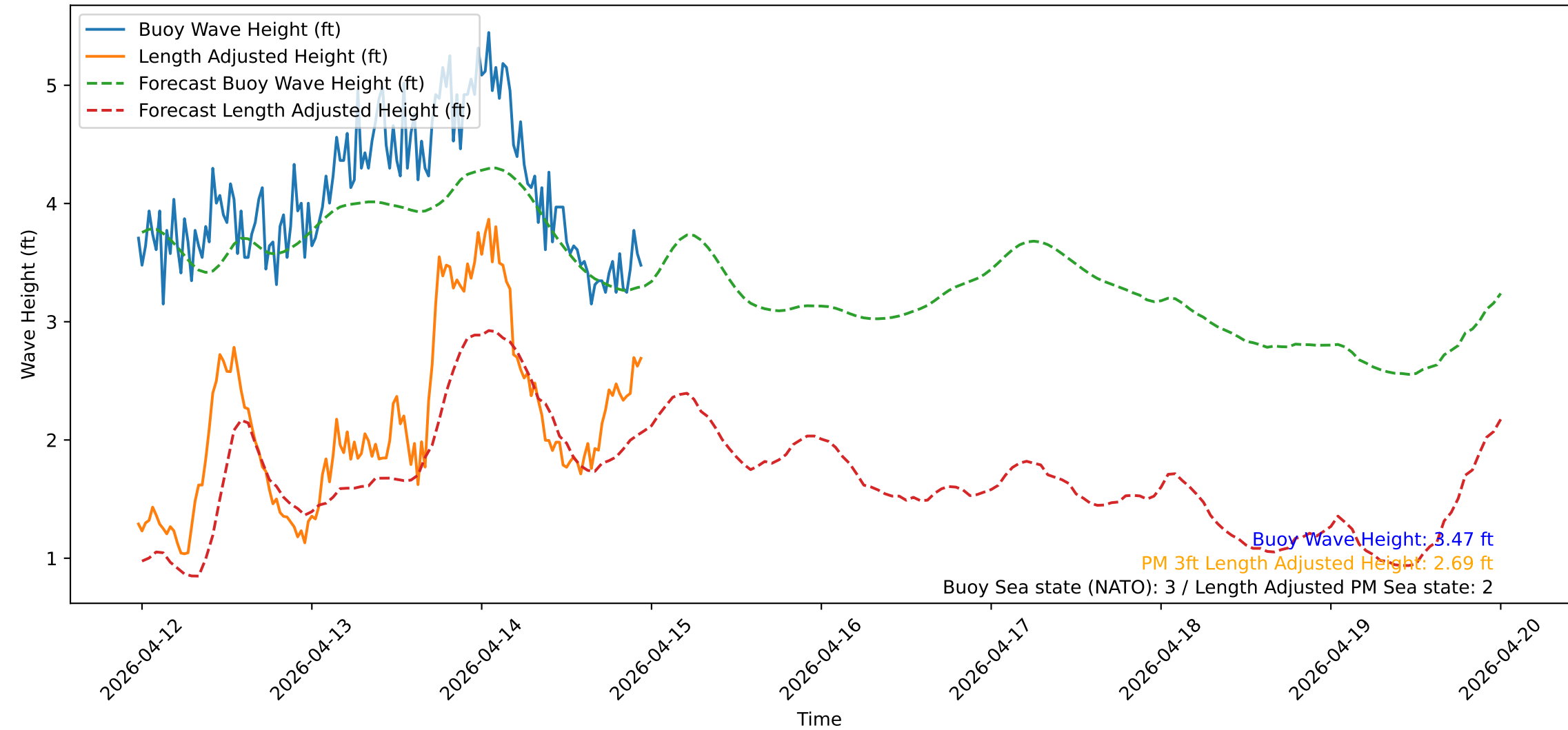
Wave Heights over Time for Oceanside Harbor at 2026-04-14 23:30:31
