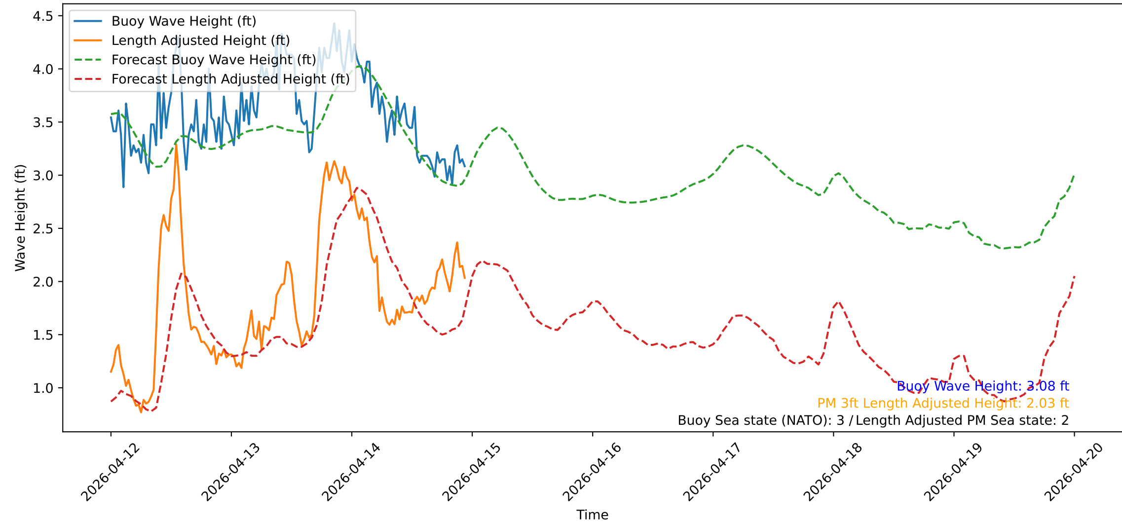
Wave Heights over Time for Red Beach at 2026-04-14 23:30:50
