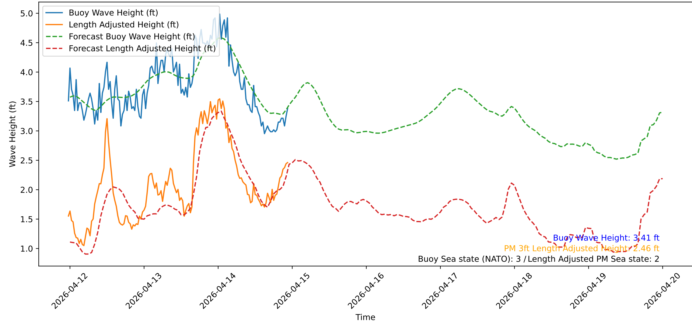
Wave Heights over Time for Green Beach at 2026-04-14 23:31:13
