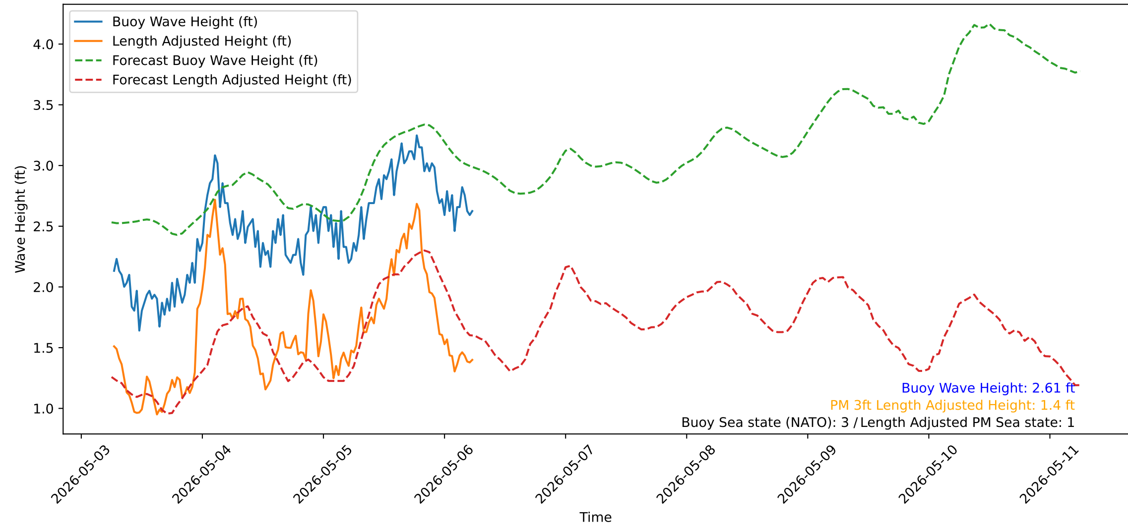
Wave Heights over Time for Oceanside Harbor at 2026-05-06 06:20:31
