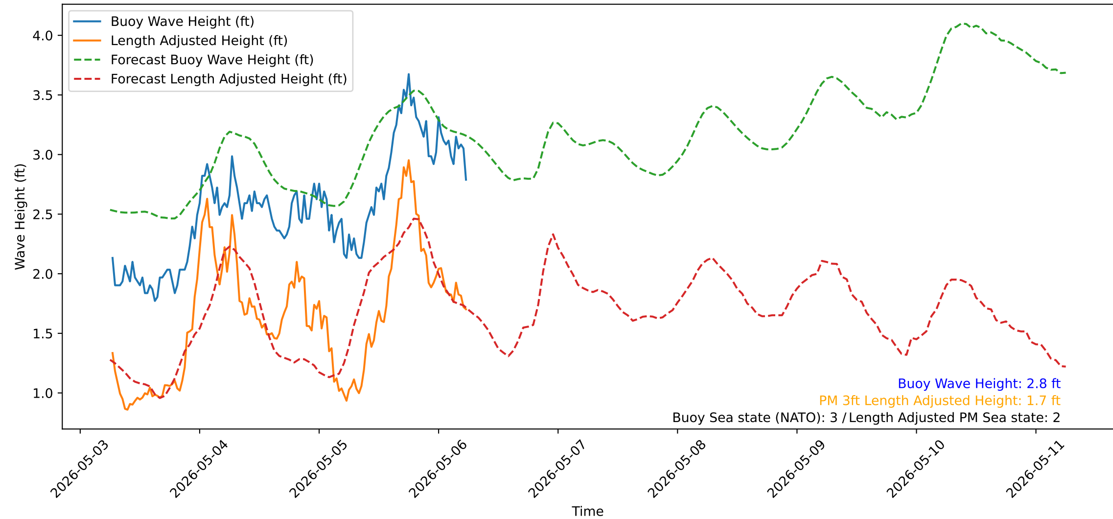
Wave Heights over Time for Green Beach at 2026-05-06 06:21:13
