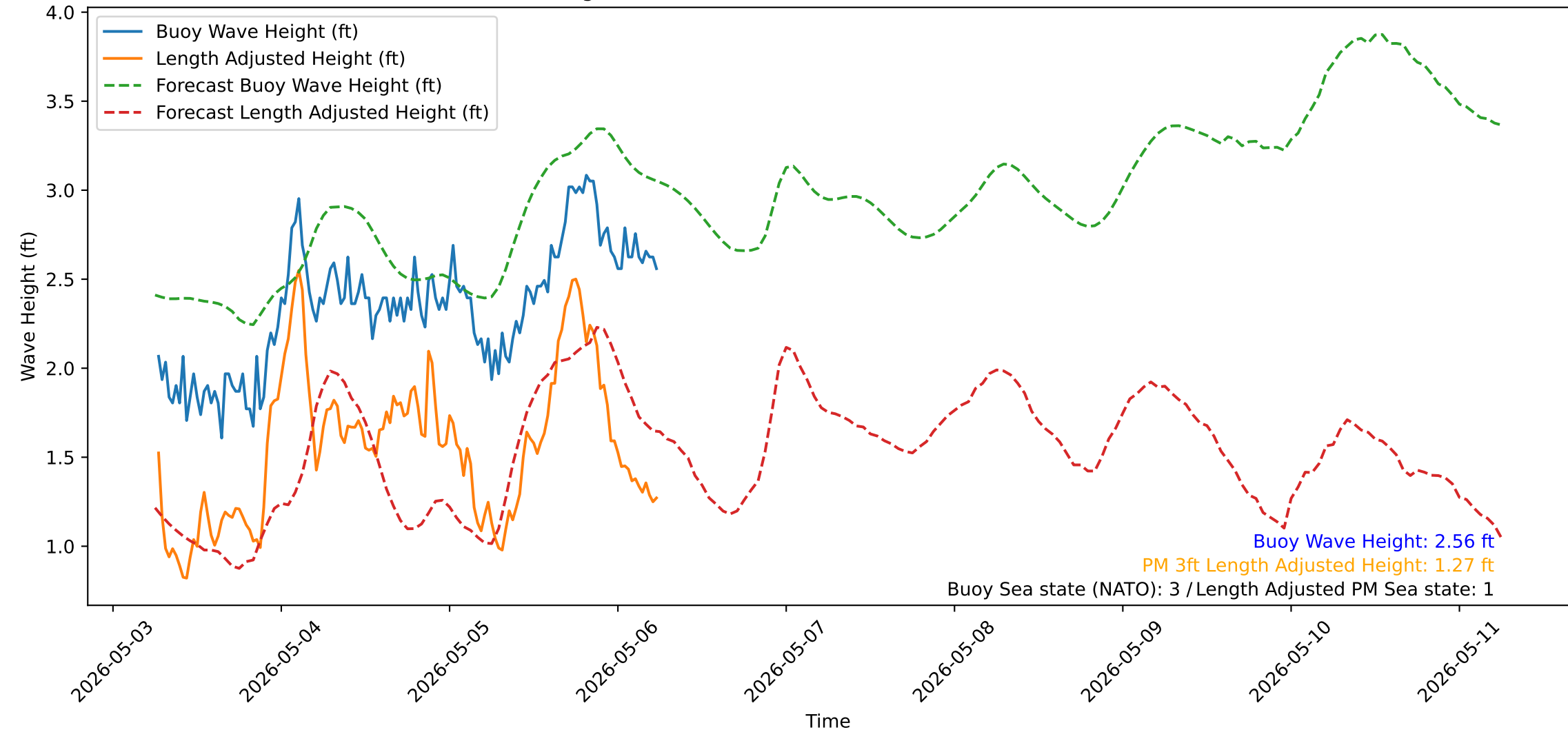
Wave Heights over Time for Red Beach at 2026-05-06 06:20:51
