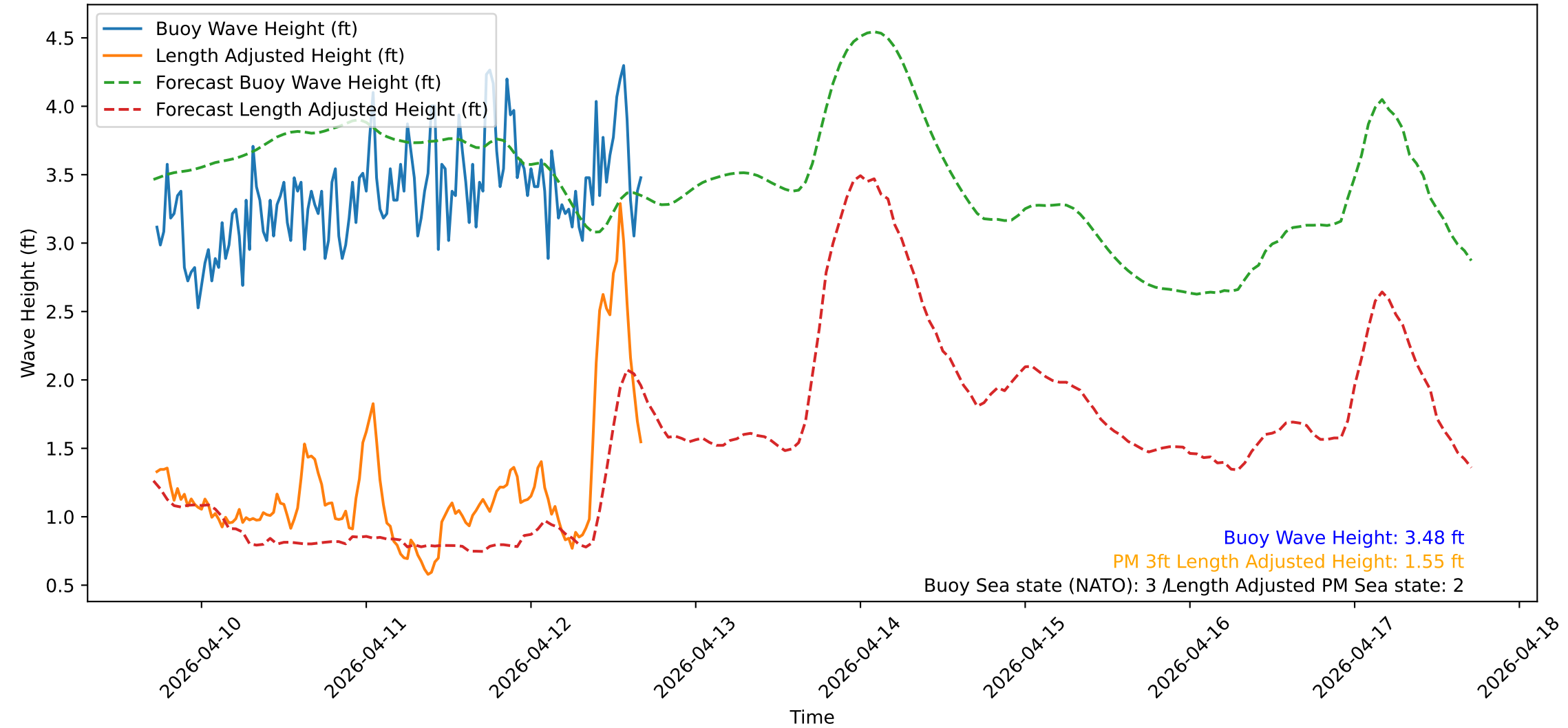
Wave Heights over Time for Red Beach at 2026-04-12 17:00:49
