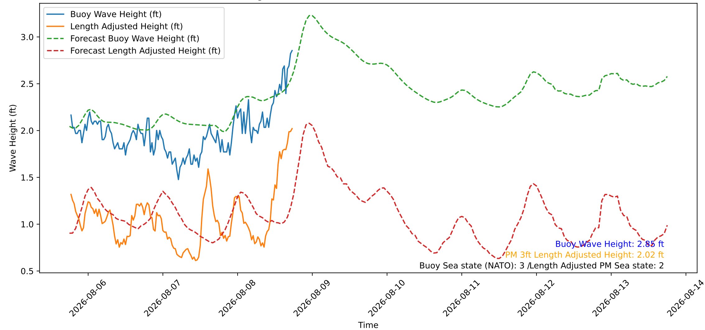
Wave Heights over Time for Red Beach at 2026-08-08 18:10:46
