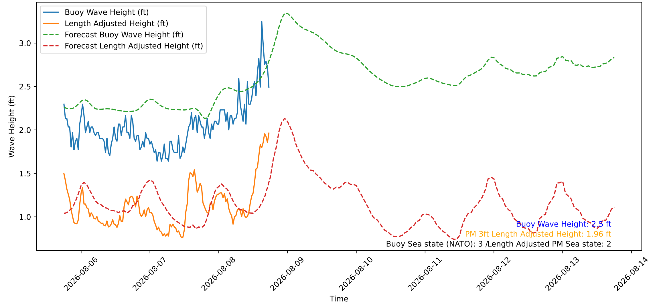
Wave Heights over Time for Oceanside Harbor at 2026-08-08 18:10:26
