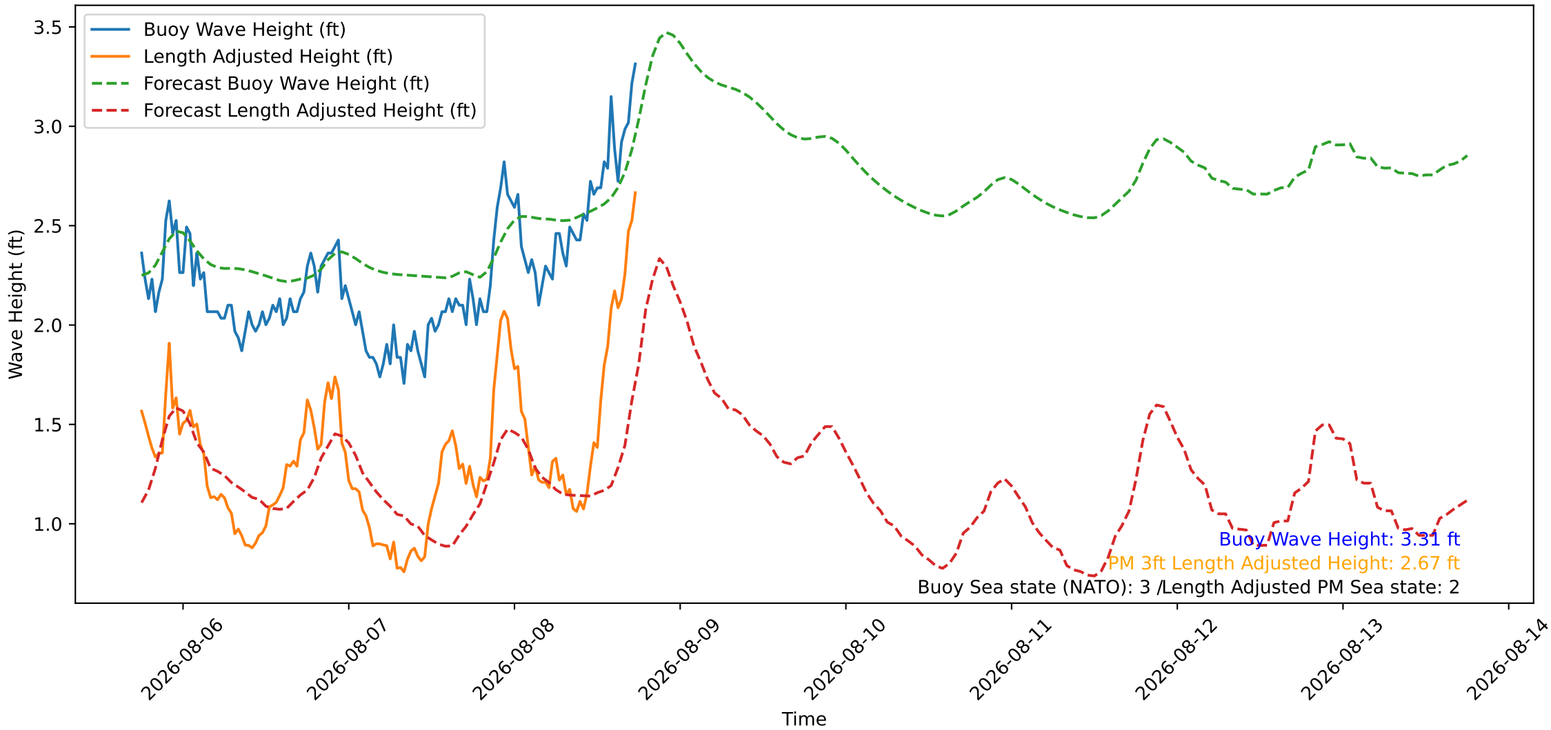
Wave Heights over Time for Green Beach at 2026-08-08 18:11:09
