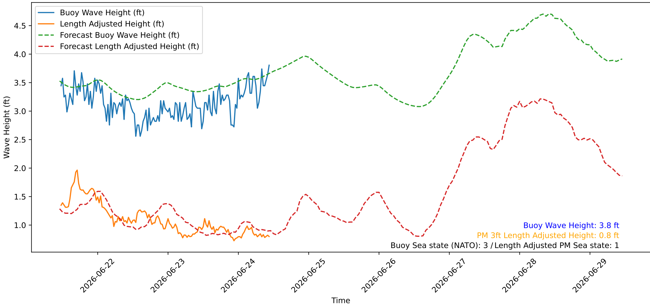
Wave Heights over Time for Oceanside Harbor at 2026-06-24 11:20:26
