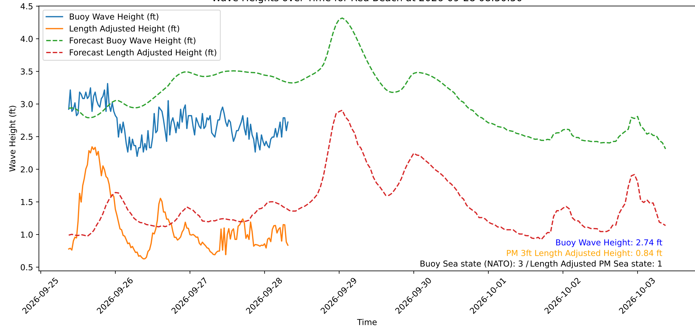
Wave Heights over Time for Red Beach at 2026-09-28 08:30:50
