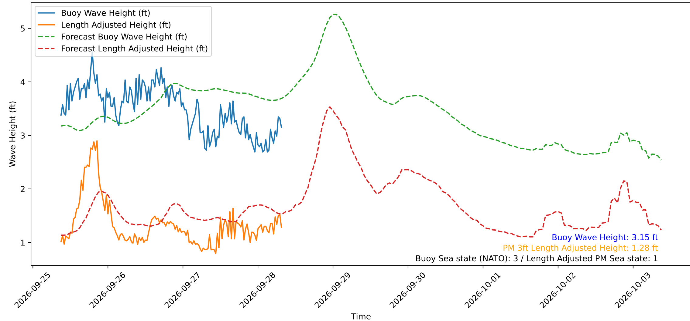
Wave Heights over Time for Green Beach at 2026-09-28 08:31:12
