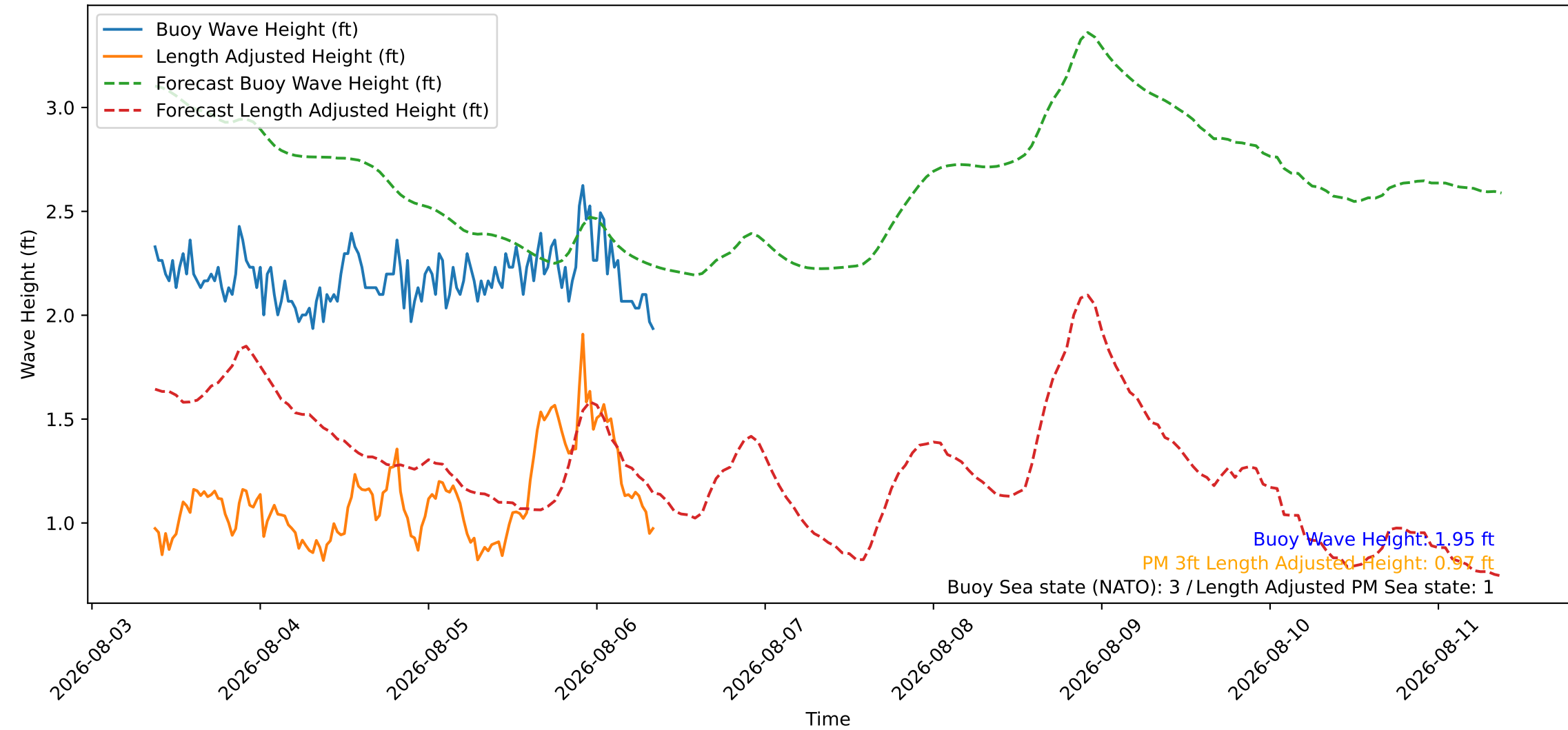
Wave Heights over Time for Green Beach at 2026-08-06 09:01:07
