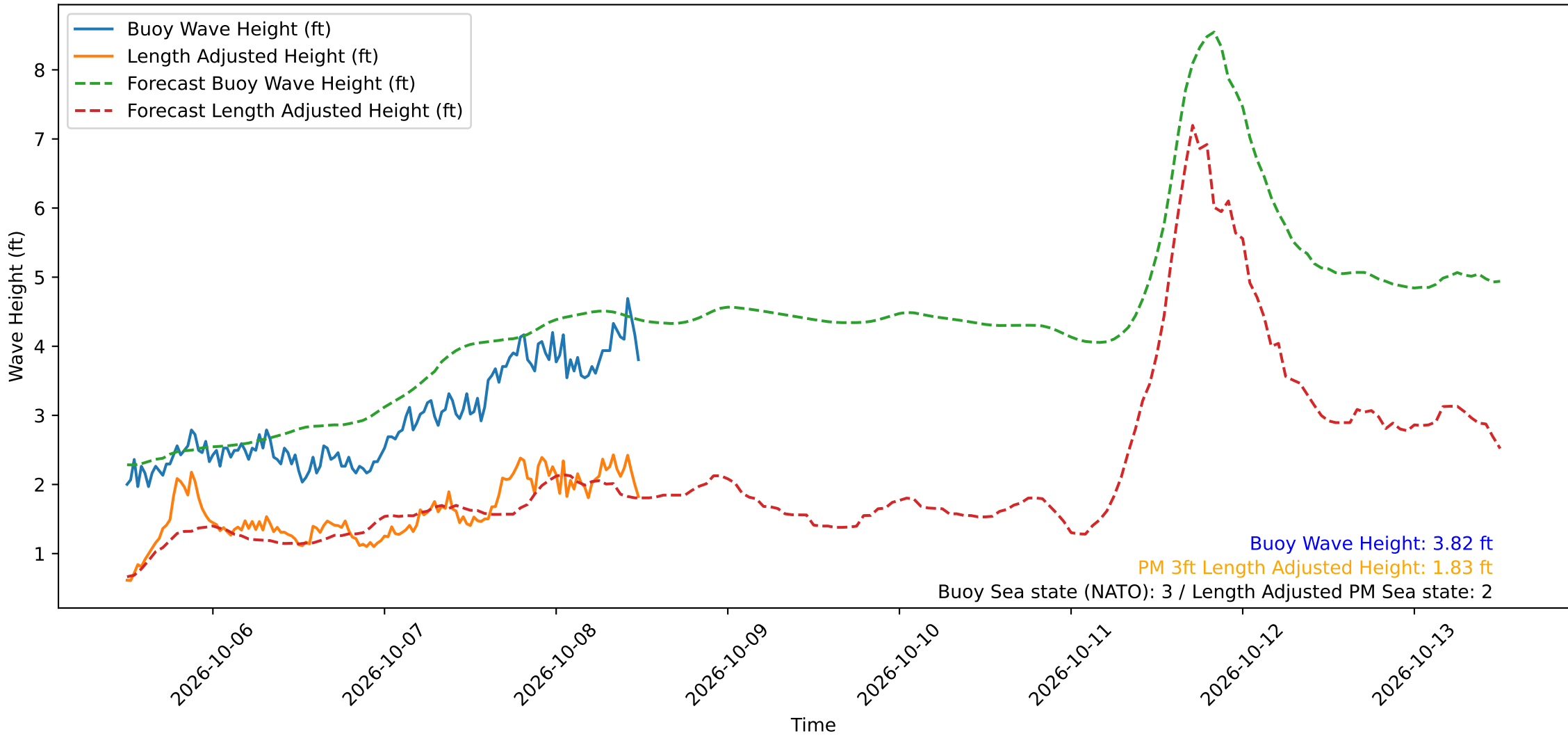
Wave Heights over Time for Oceanside Harbor at 2026-10-08 12:10:30
