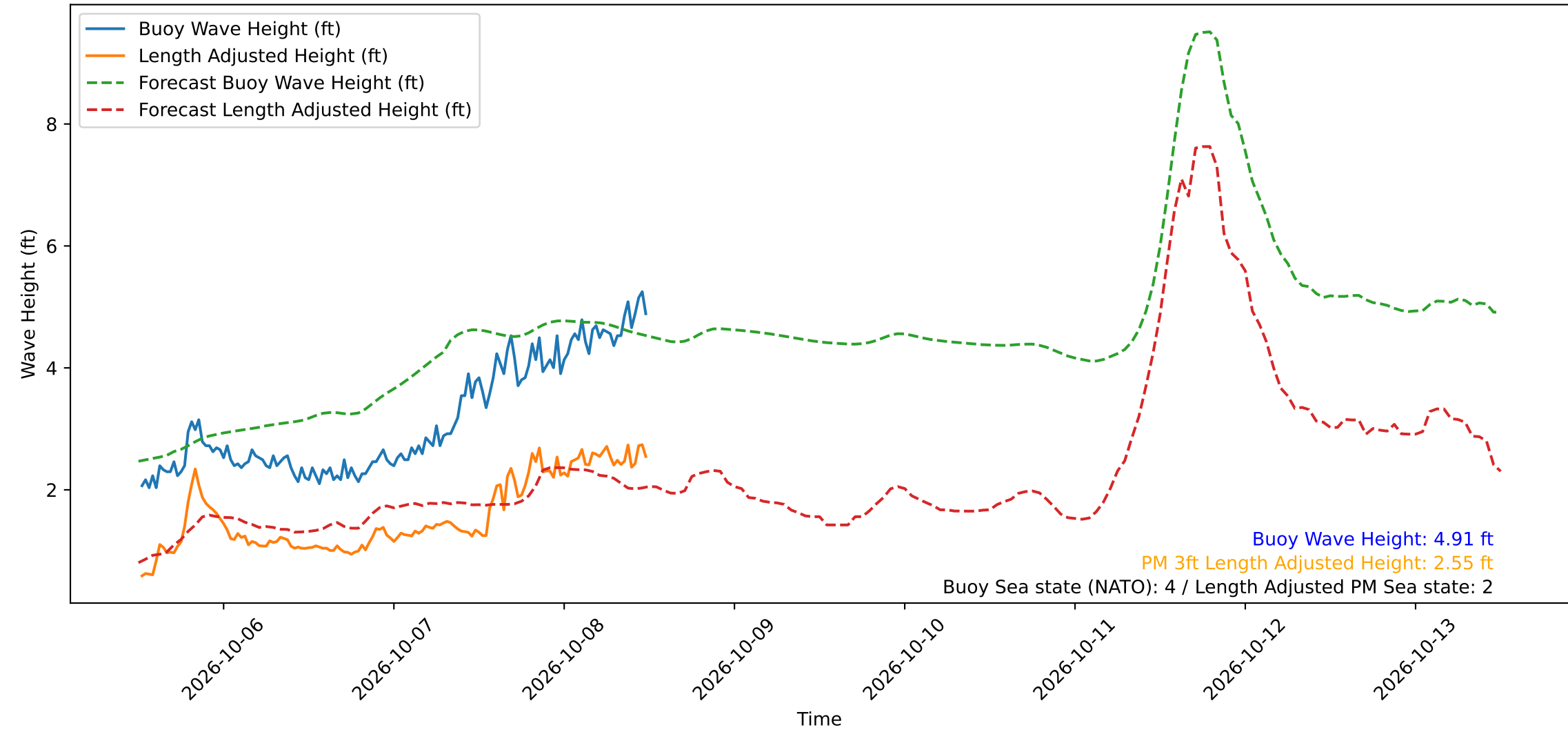
Wave Heights over Time for Green Beach at 2026-10-08 12:11:12
