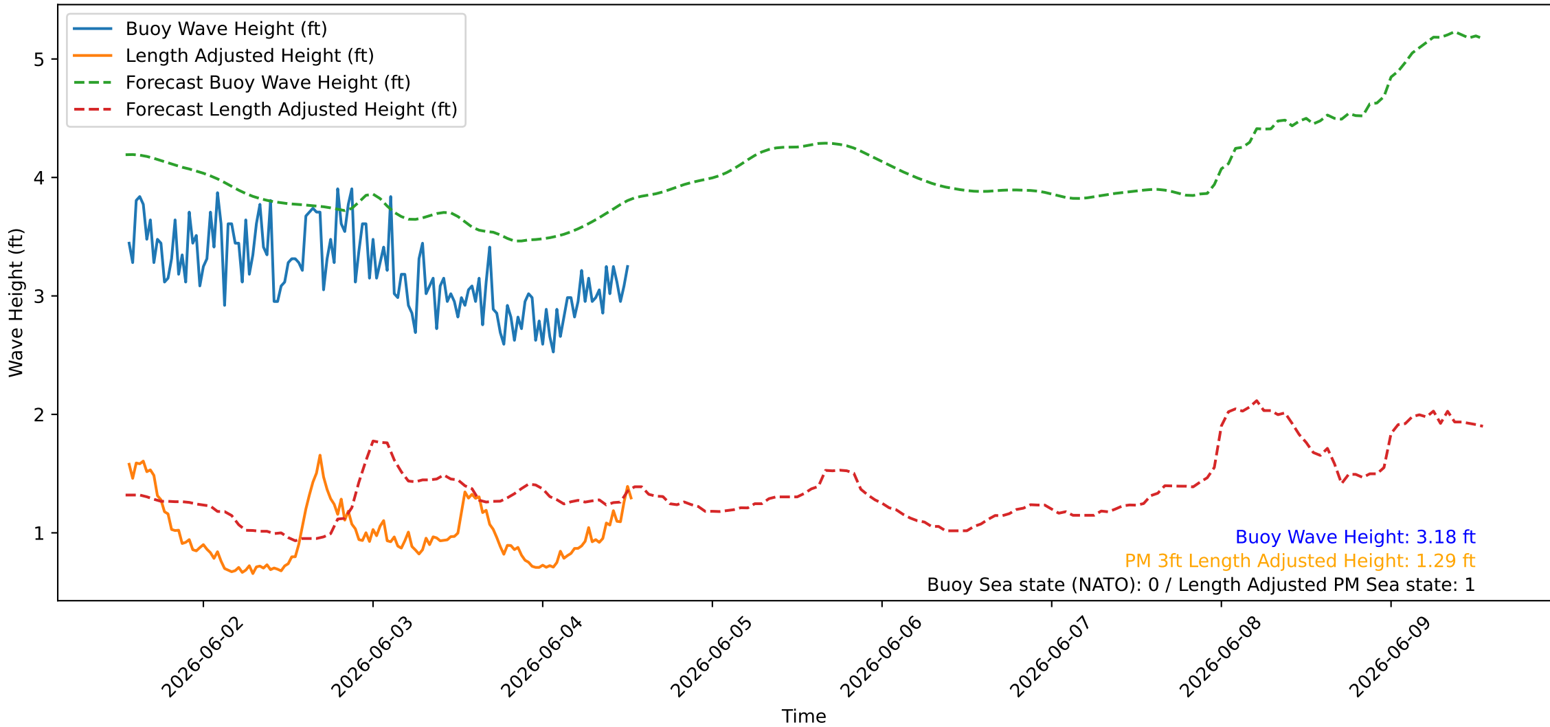
Wave Heights over Time for Red Beach at 2026-06-04 13:10:44
