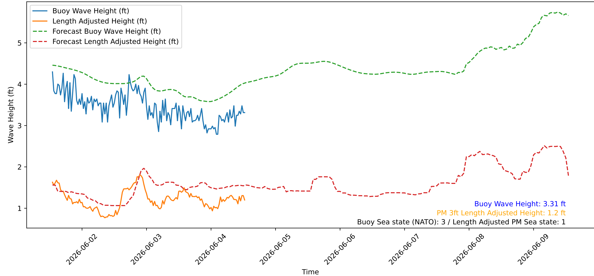
Wave Heights over Time for Green Beach at 2026-06-04 13:11:06
