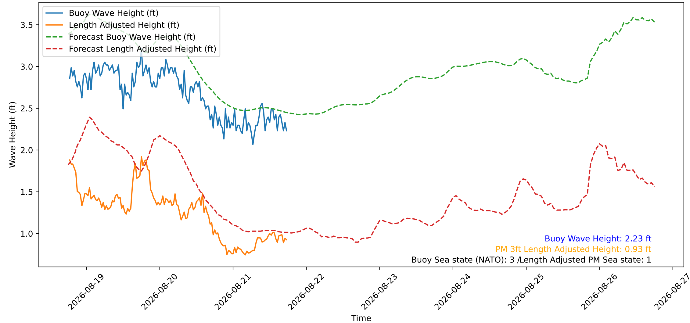
Wave Heights over Time for Red Beach at 2026-08-21 18:10:46
