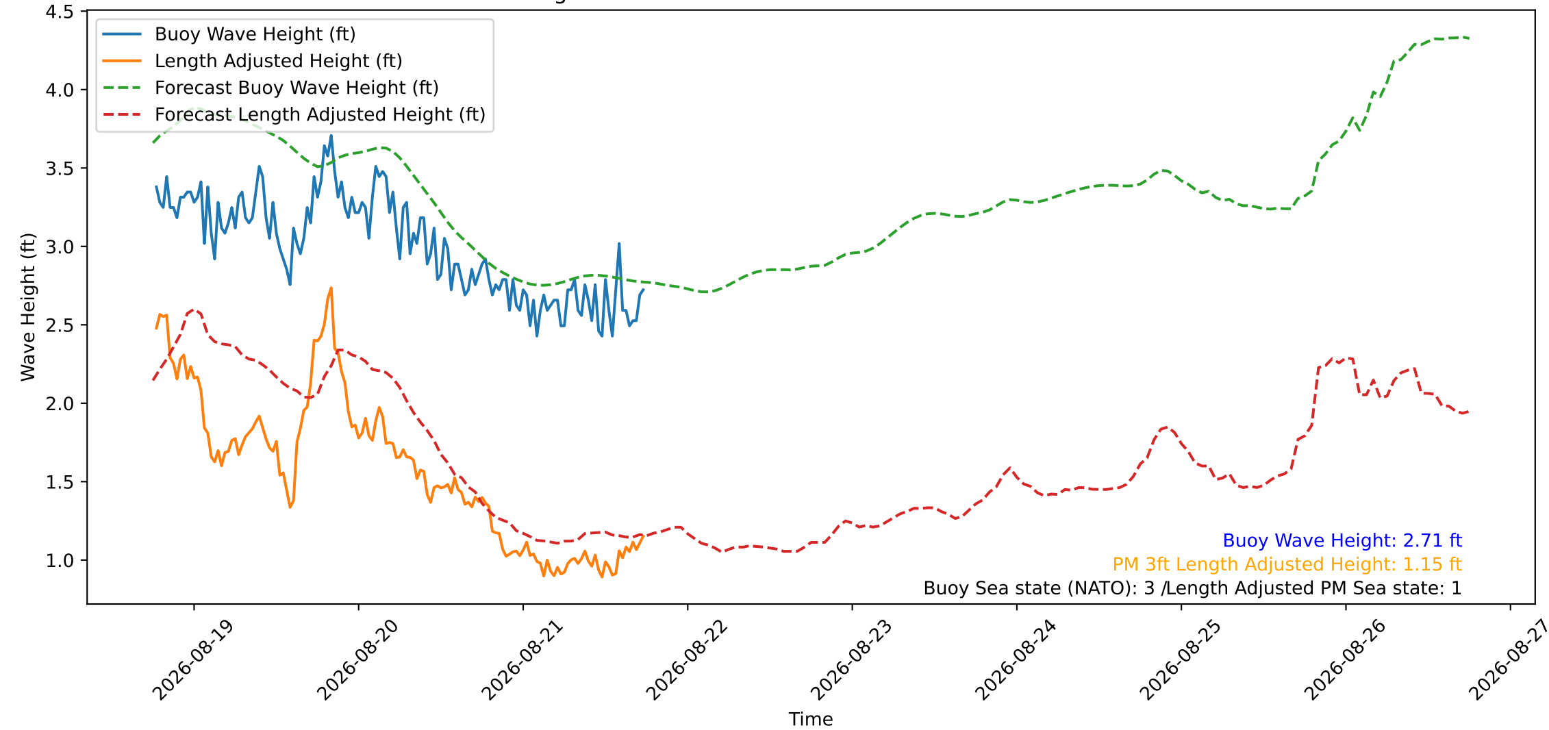
Wave Heights over Time for Green Beach at 2026-08-21 18:11:09
