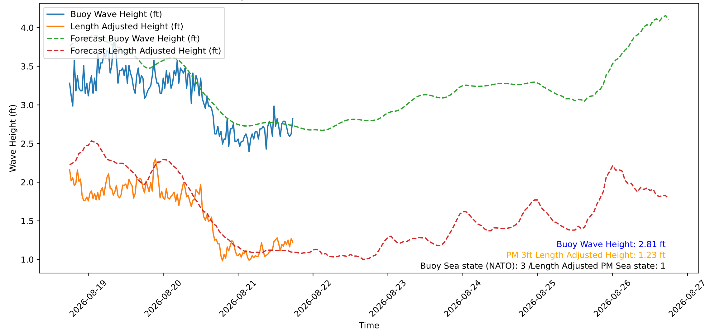
Wave Heights over Time for Oceanside Harbor at 2026-08-21 18:10:27
