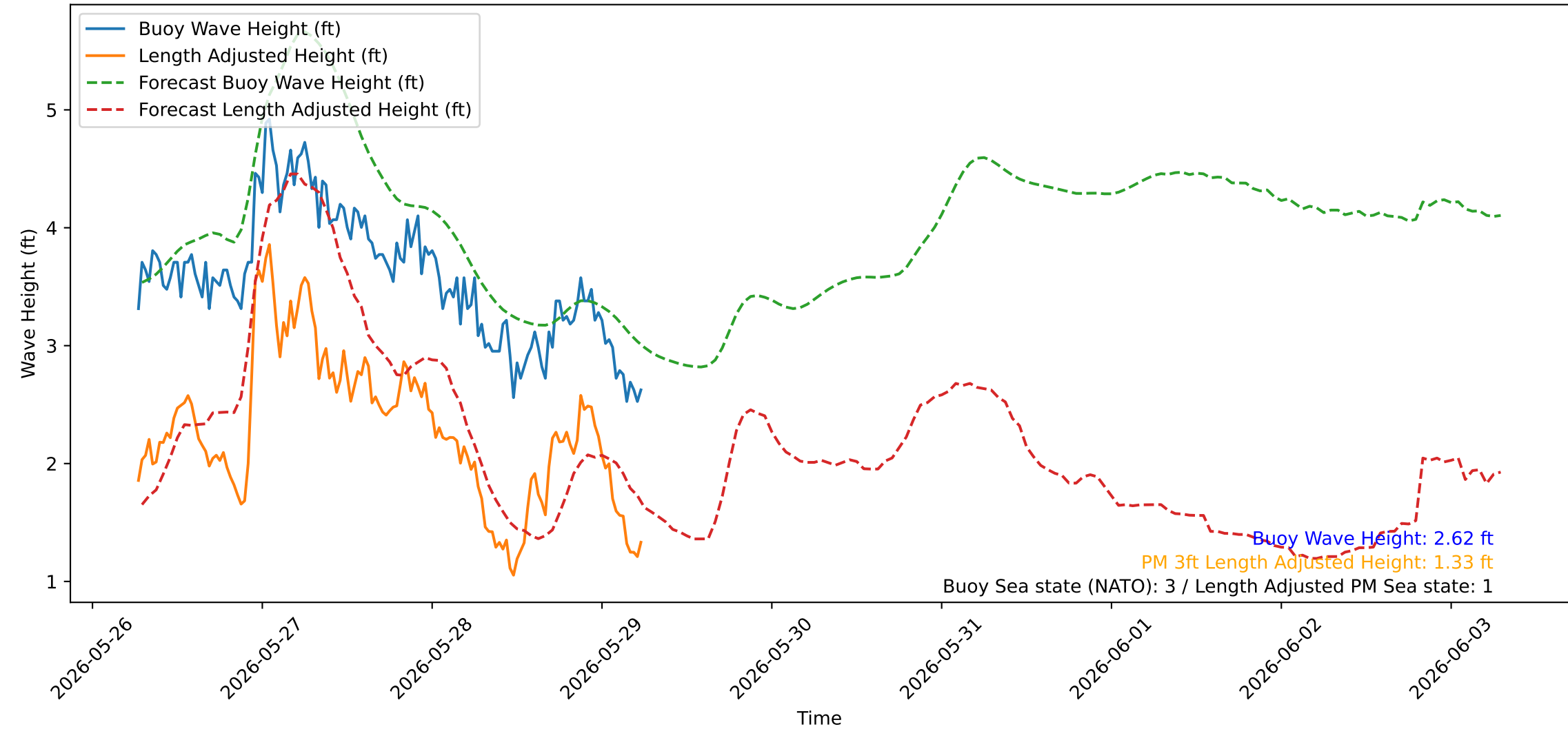
Wave Heights over Time for Green Beach at 2026-05-29 06:31:03
