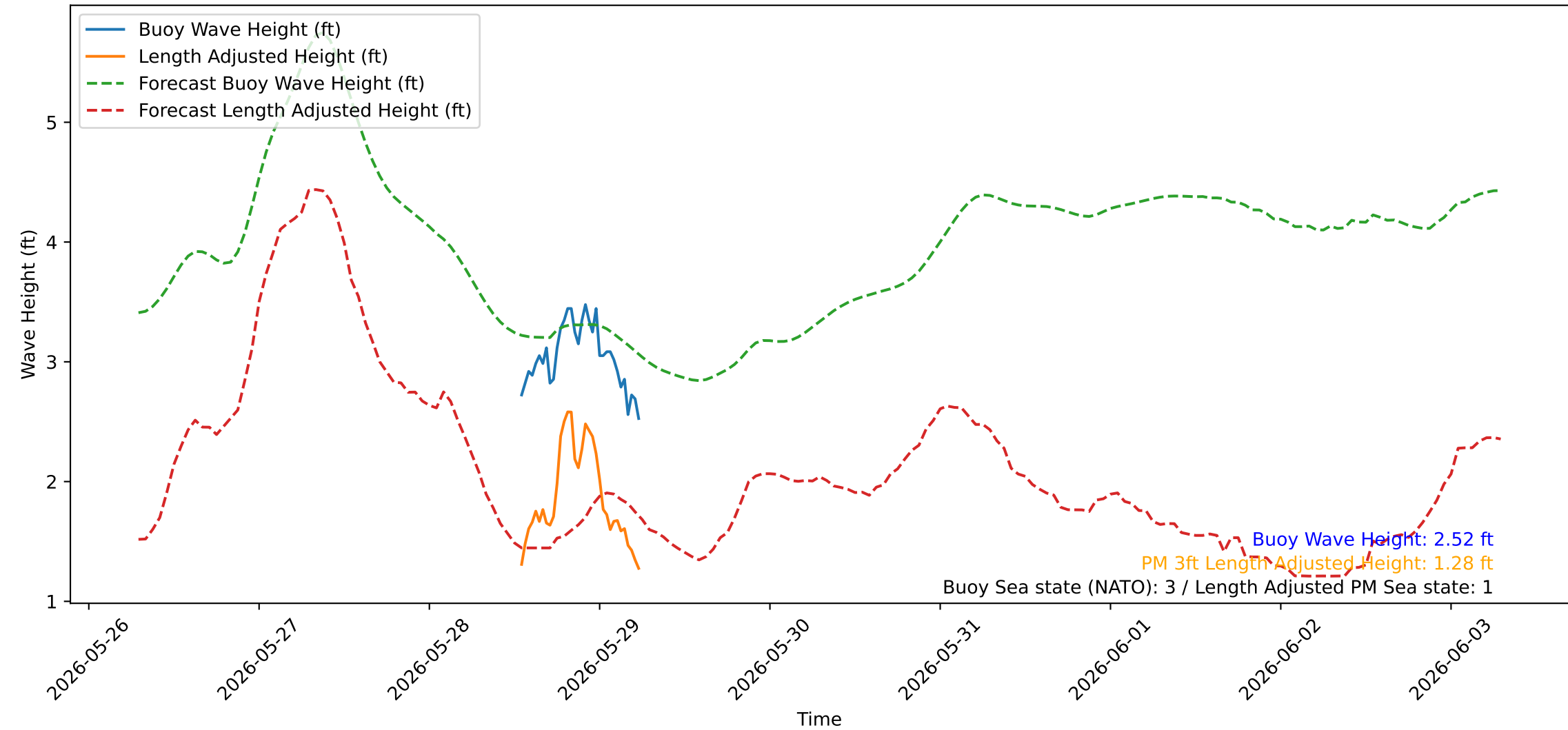
Wave Heights over Time for Oceanside Harbor at 2026-05-29 06:30:21
