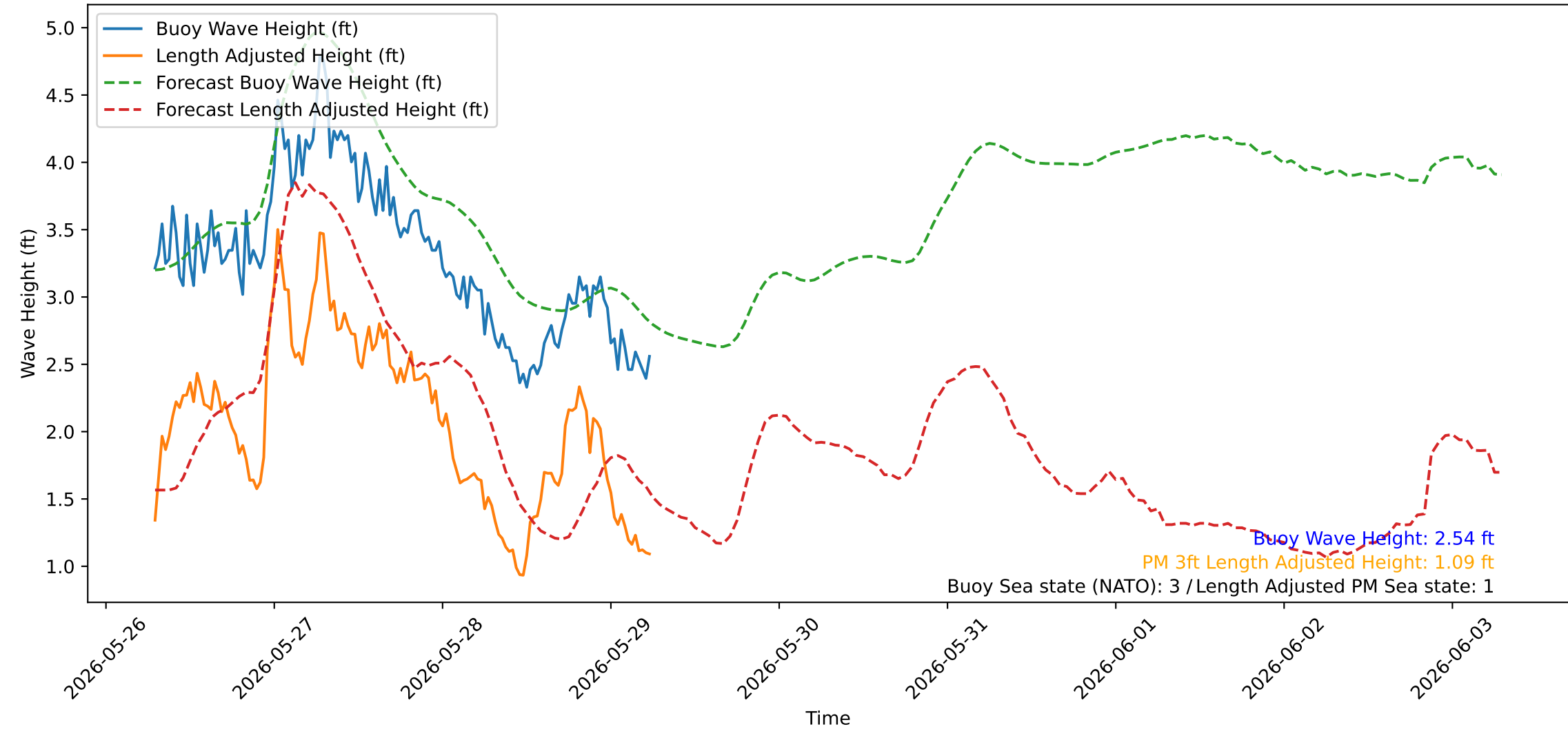
Wave Heights over Time for Red Beach at 2026-05-29 06:30:40
