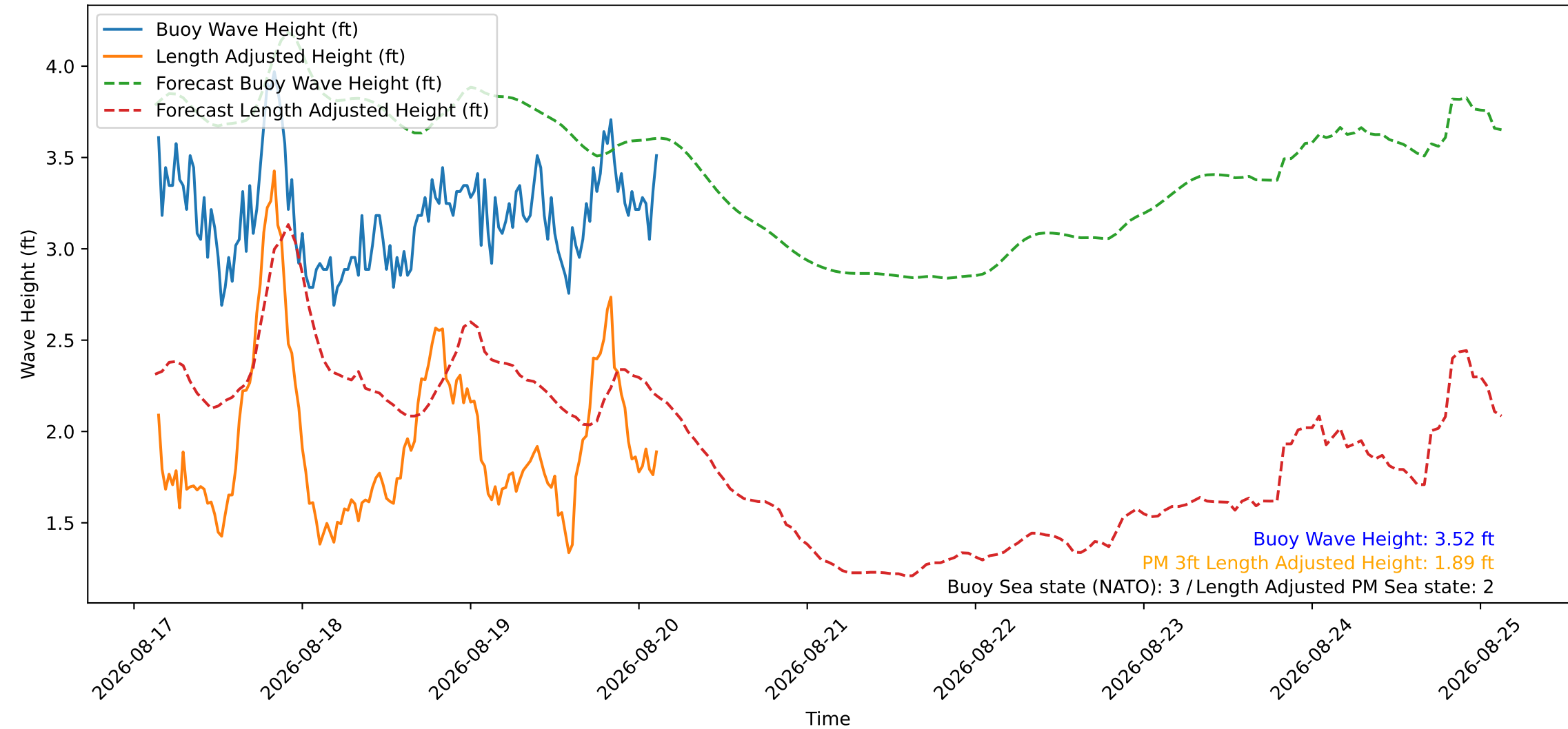
Wave Heights over Time for Green Beach at 2026-08-20 03:21:11
