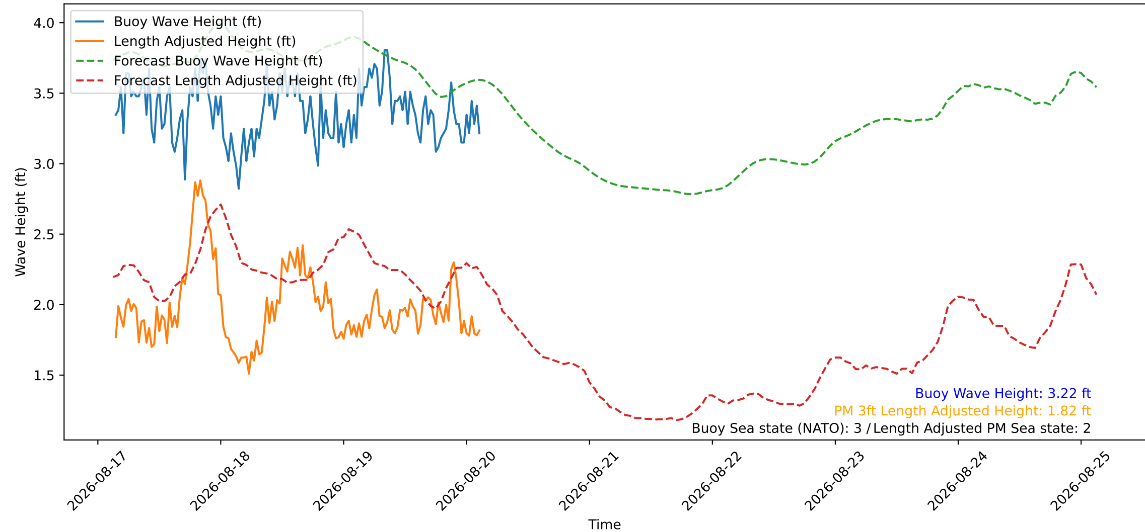
Wave Heights over Time for Oceanside Harbor at 2026-08-20 03:20:26
