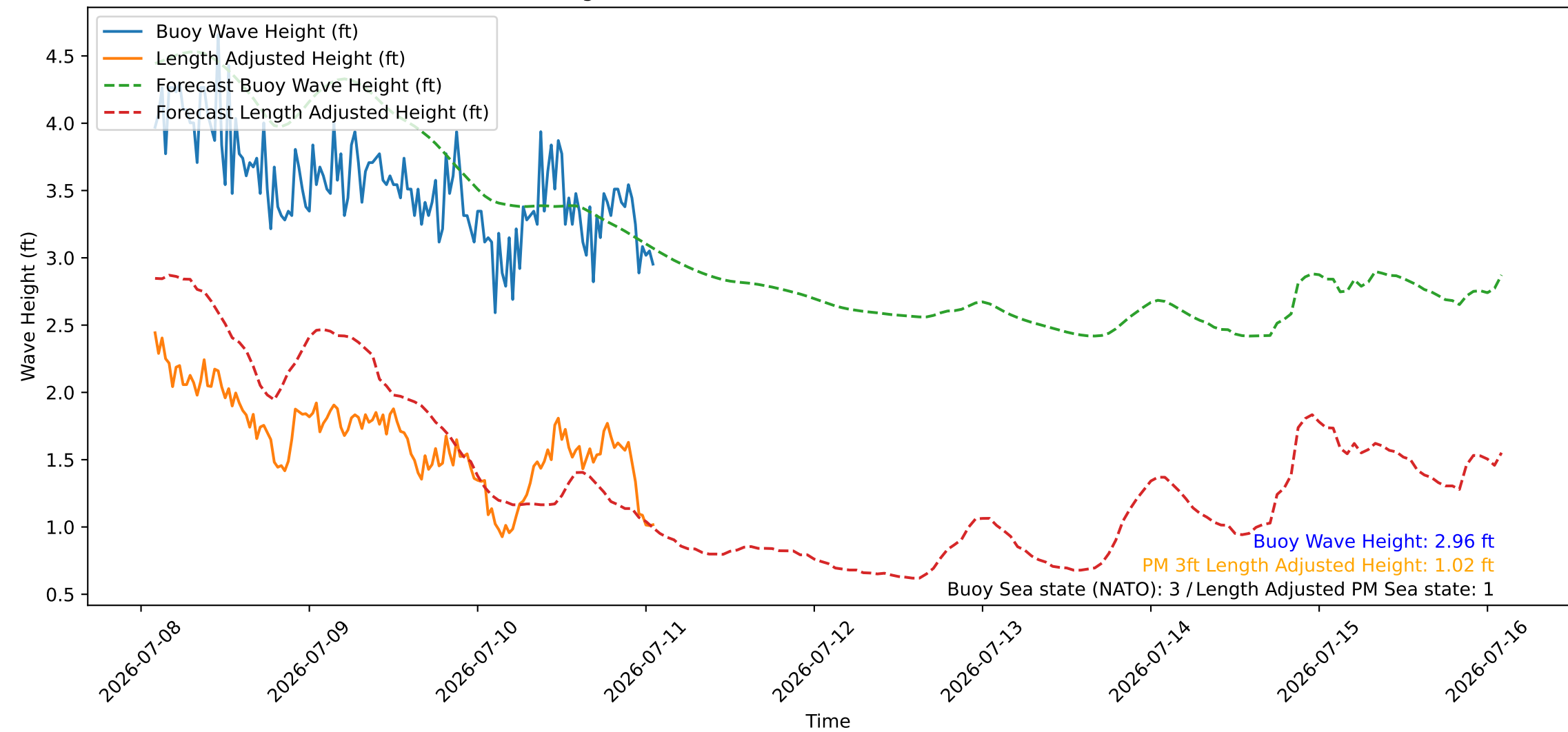
Wave Heights over Time for Red Beach at 2026-07-11 01:50:48
