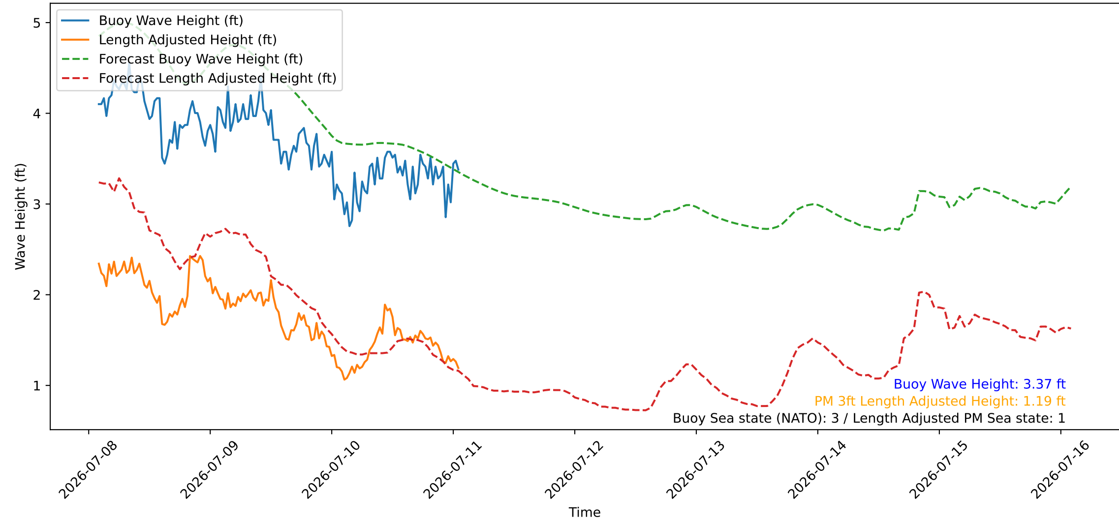
Wave Heights over Time for Green Beach at 2026-07-11 01:51:10
