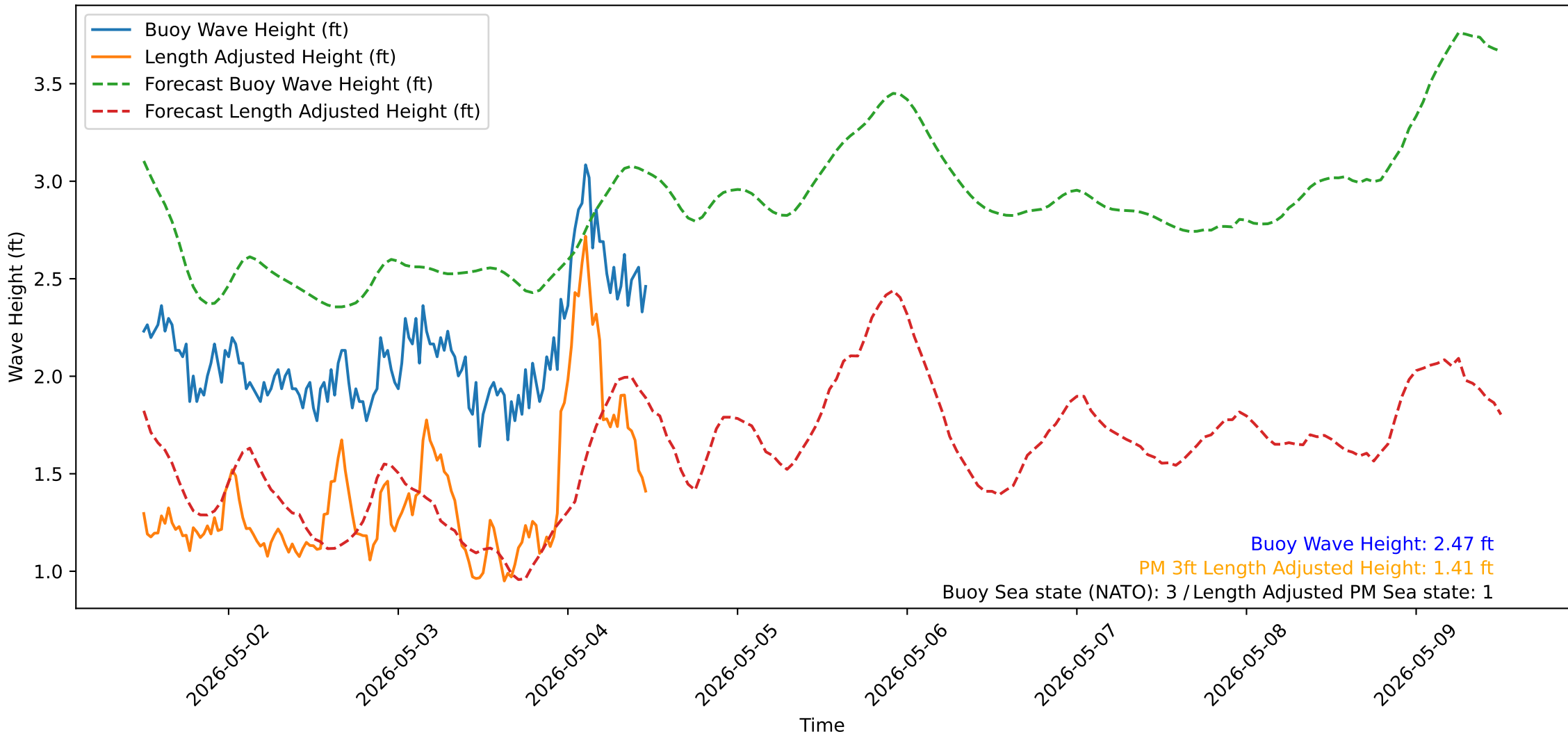
Wave Heights over Time for Oceanside Harbor at 2026-05-04 11:50:31
