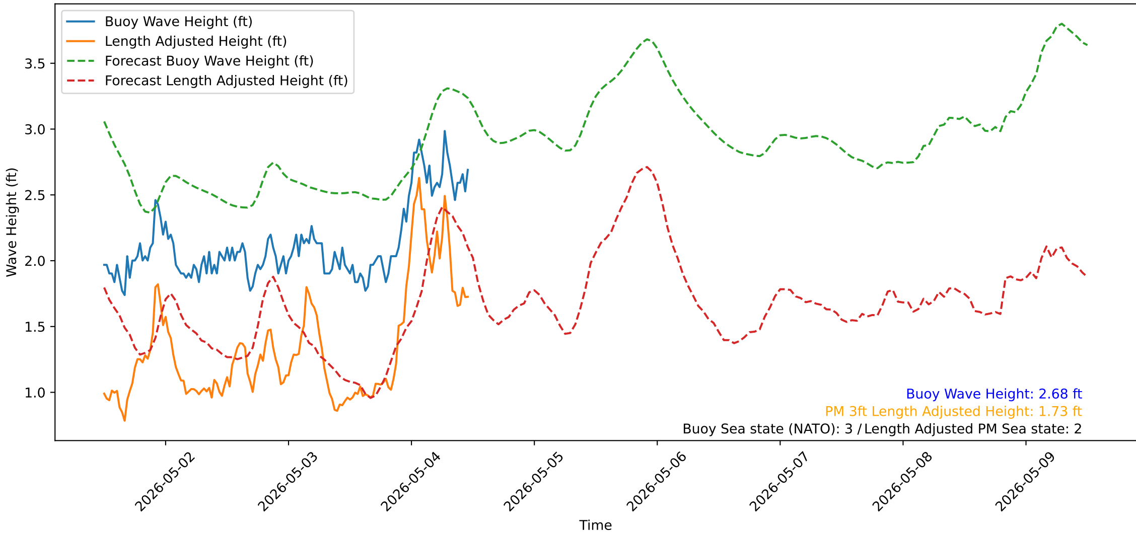
Wave Heights over Time for Green Beach at 2026-05-04 11:51:13
